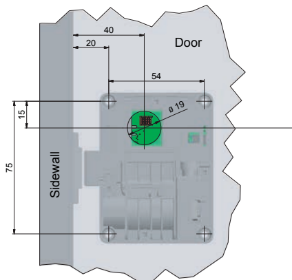
Mounting position of lock M410 / M410 pro
