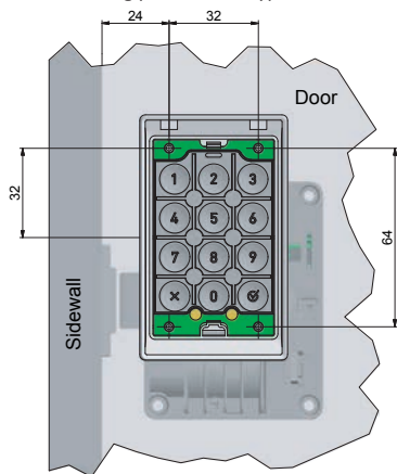
Mounting position of keypad TA03
