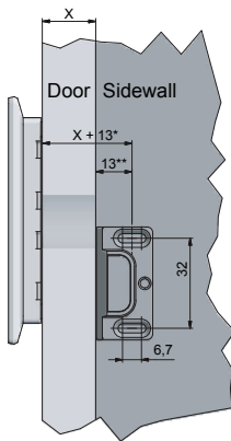
Mounting position of striker plate 4005
