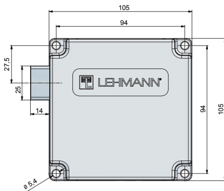
(M610 / M610 pro for left hand doors)
