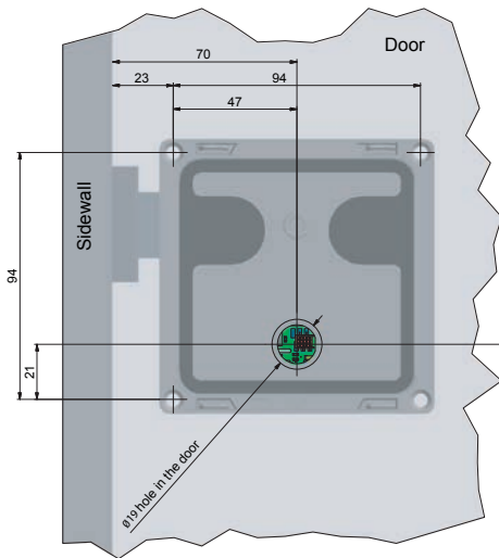
Mounting position of lock M610 / M610 pro
