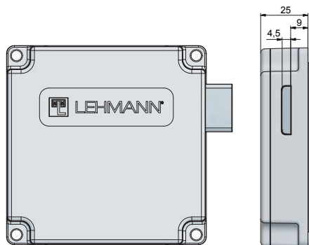
(M610 / M610 pro for right hand doors)
