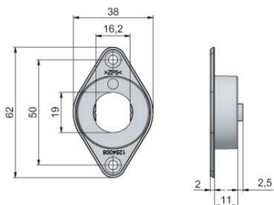
Fixing element 1619
