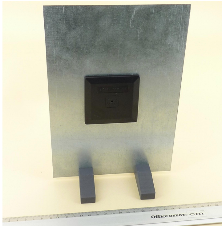
201474_eut01: Front view EUT in Setup B
