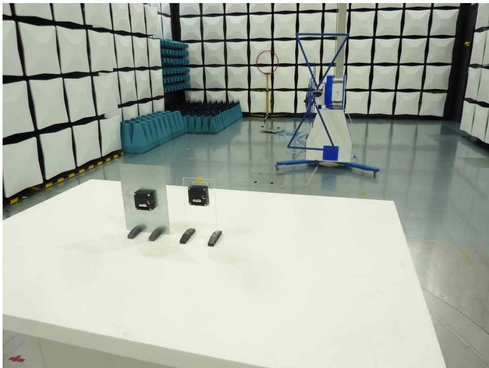
201474_04: Final measurement 30 - 1000 MHz
