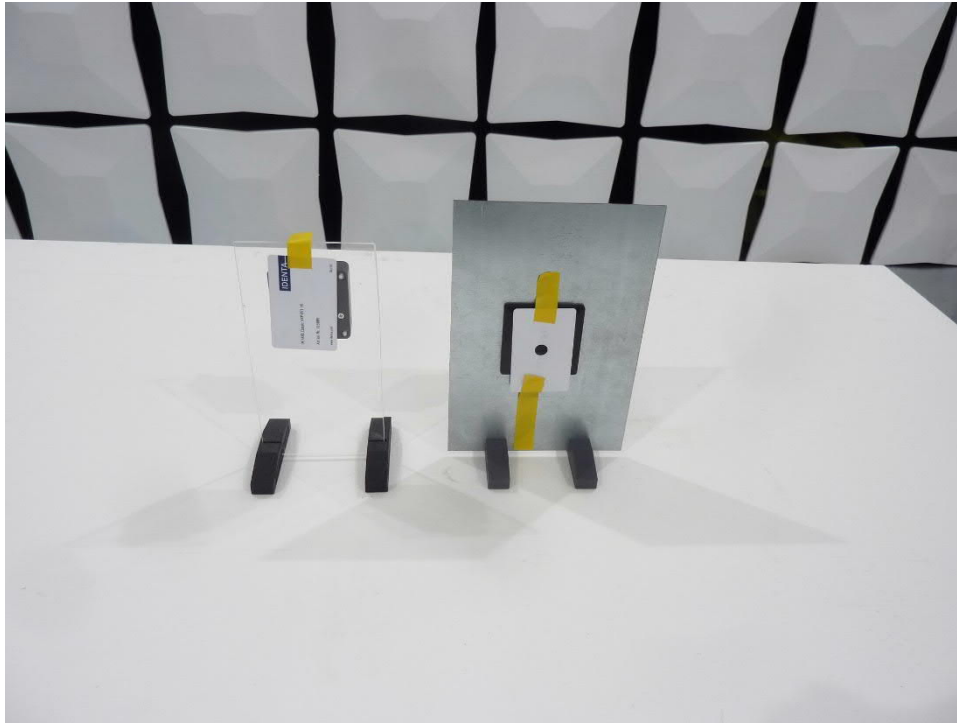
201474_01: Setup EUT
