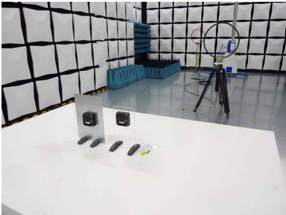
201474_02: Preliminary measurement 9 kHz - 30 MHz
