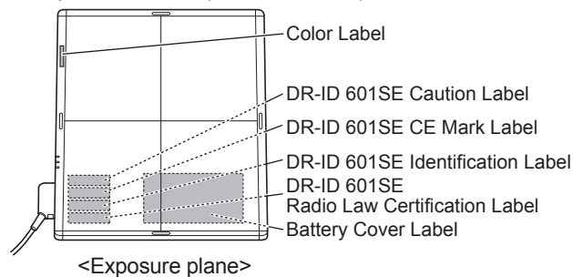
Flat panel sensor (DR-ID 601SE)
