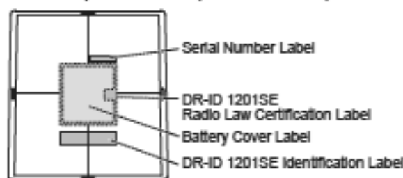
Flat panel sensor (DR-ID 1201SE)
