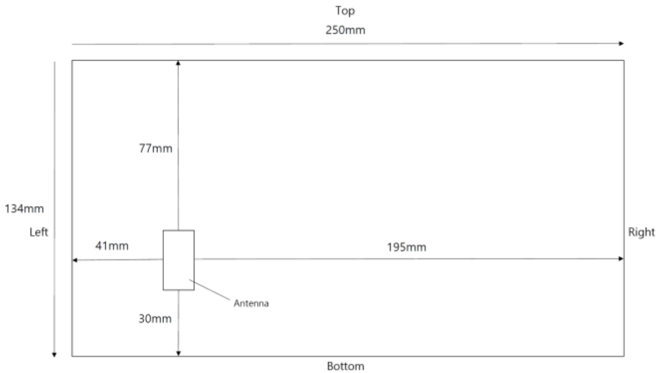
Figure E-1 Antenna Location
