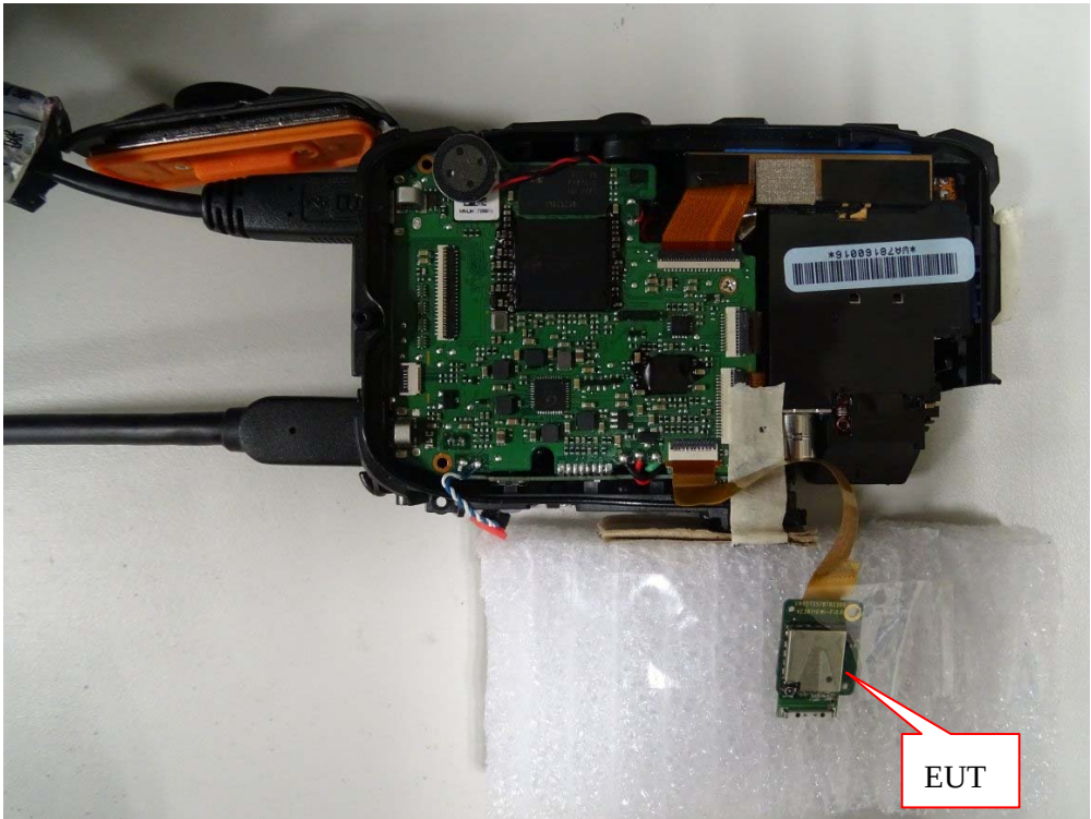
Test Fixture
