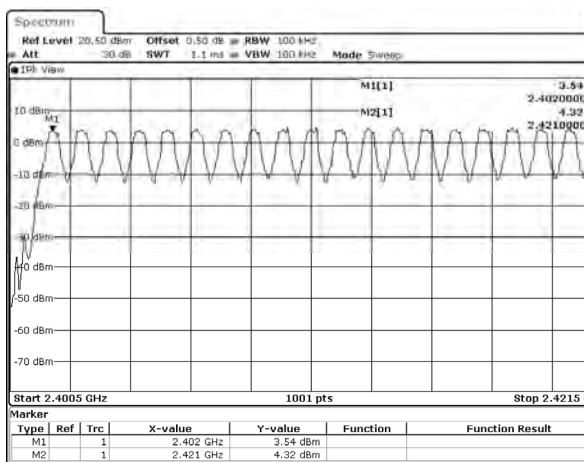
2402-2421MHz
