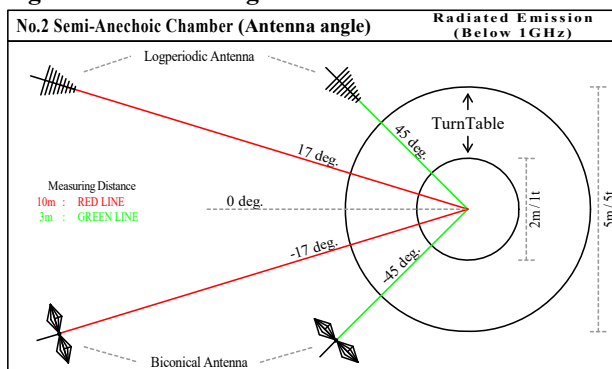
Figure 2. Antenna angle
