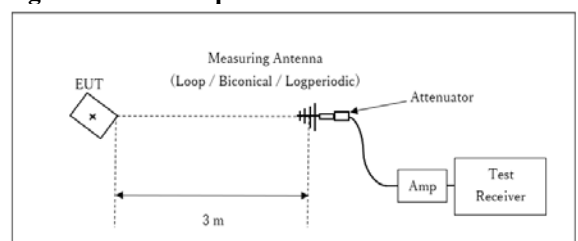
Figure 3. Test setup
