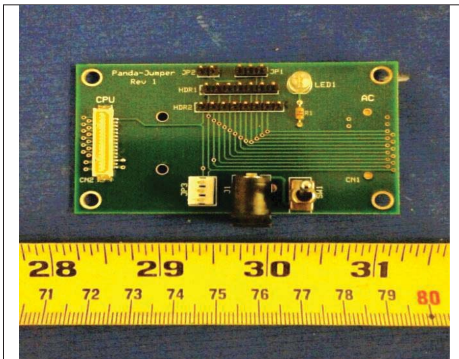
PCBA2 –Top View
