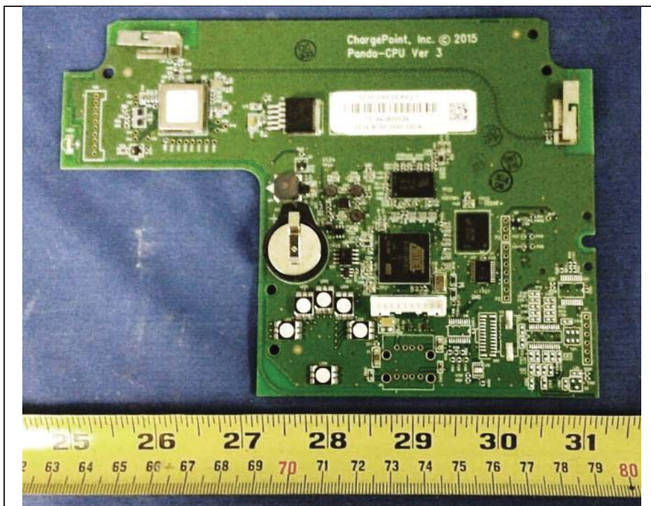
EUT Top View
