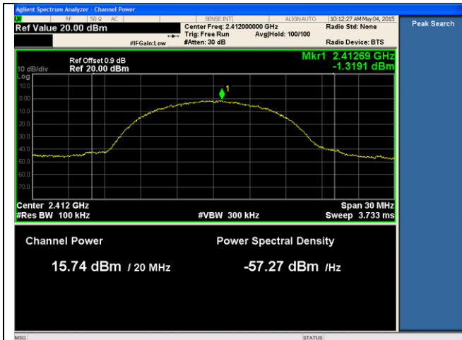
PSD-2.4G-802.11b Low
