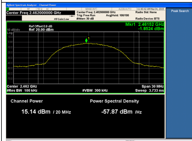
PSD-2.4G-802.11b High
