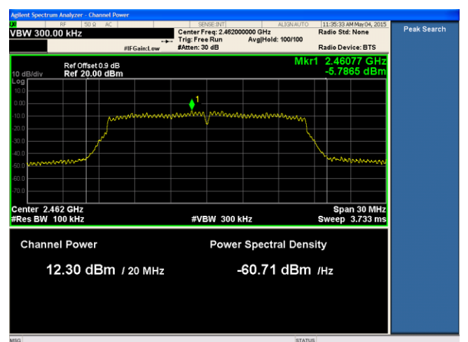
PSD-2.4G-802.11g High
