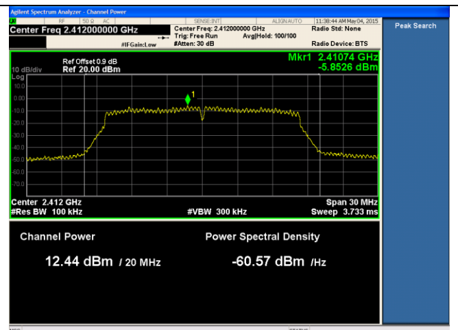
PSD-2.4G-802.11g Low
