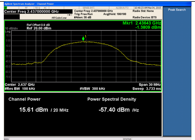
PSD-2.4G-802.11b Mid
