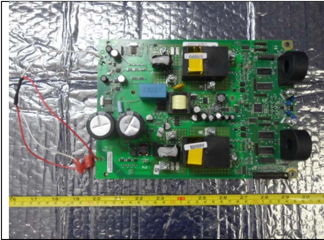
PCBA – Power Supply Top View
