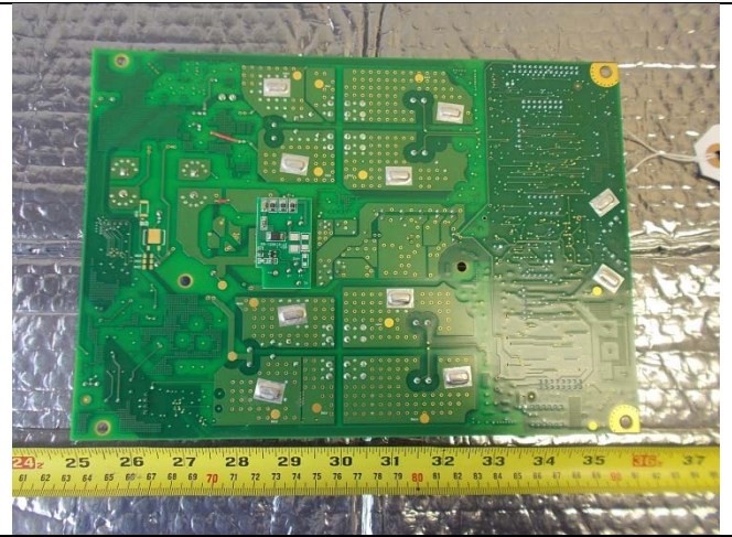
PCBA – Power Supply Bottom View
