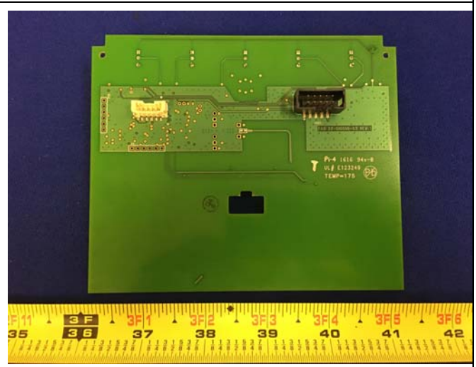
EUT-RFID Board with antenna Rear View
