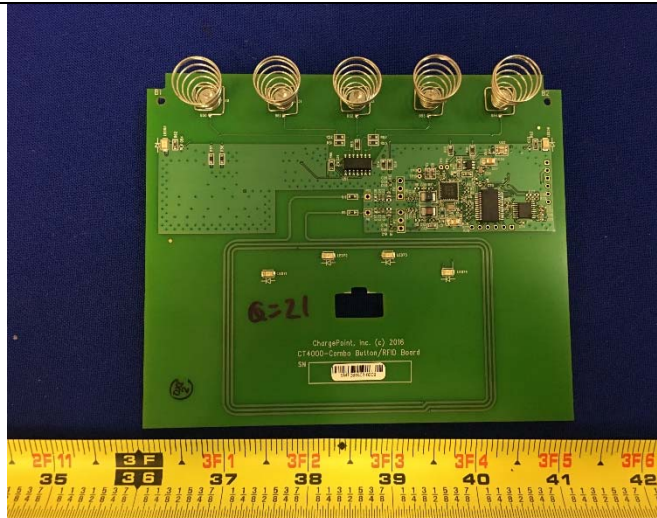
EUT-RFID Board with antenna Front View
