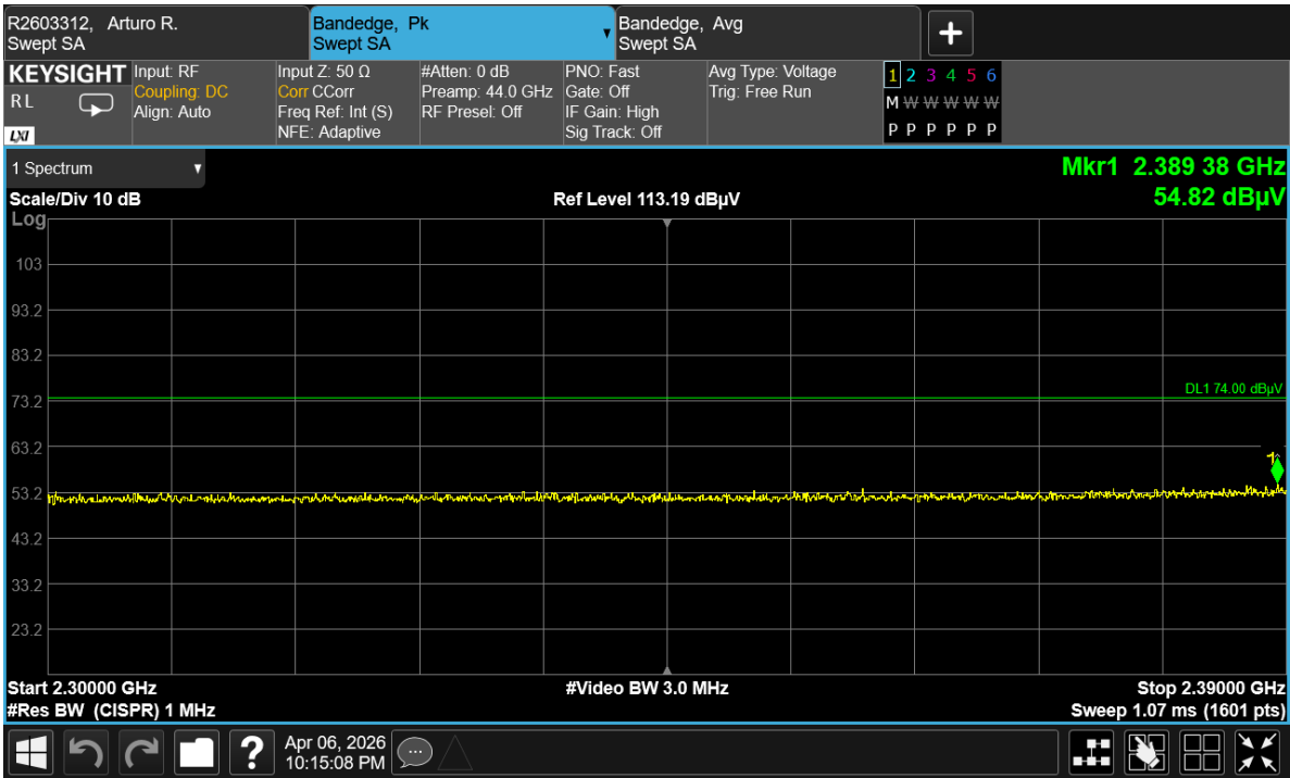
Low Channel, 2412 MHz, Lower Band Edge, Peak Measurement
