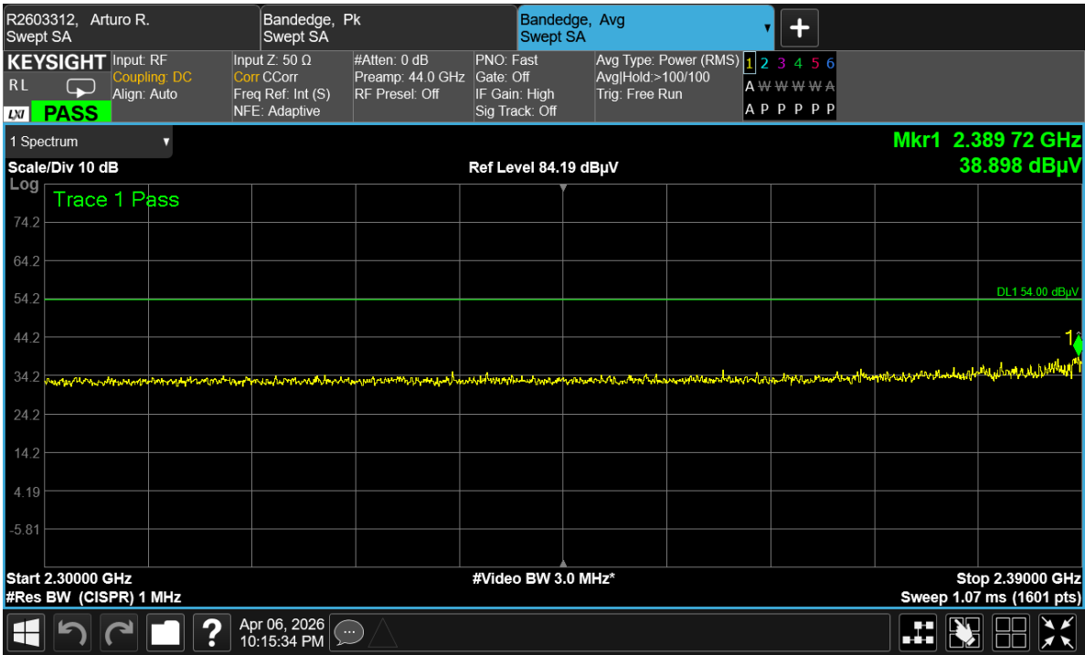
Low Channel, 2412 MHz, Lower Band Edge, Average Measurement
