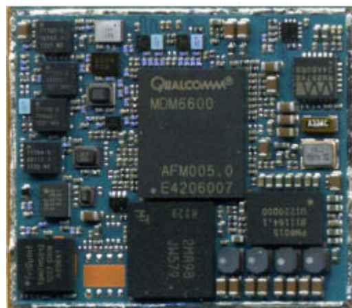
EUT – WWAN Radio without Shielding
