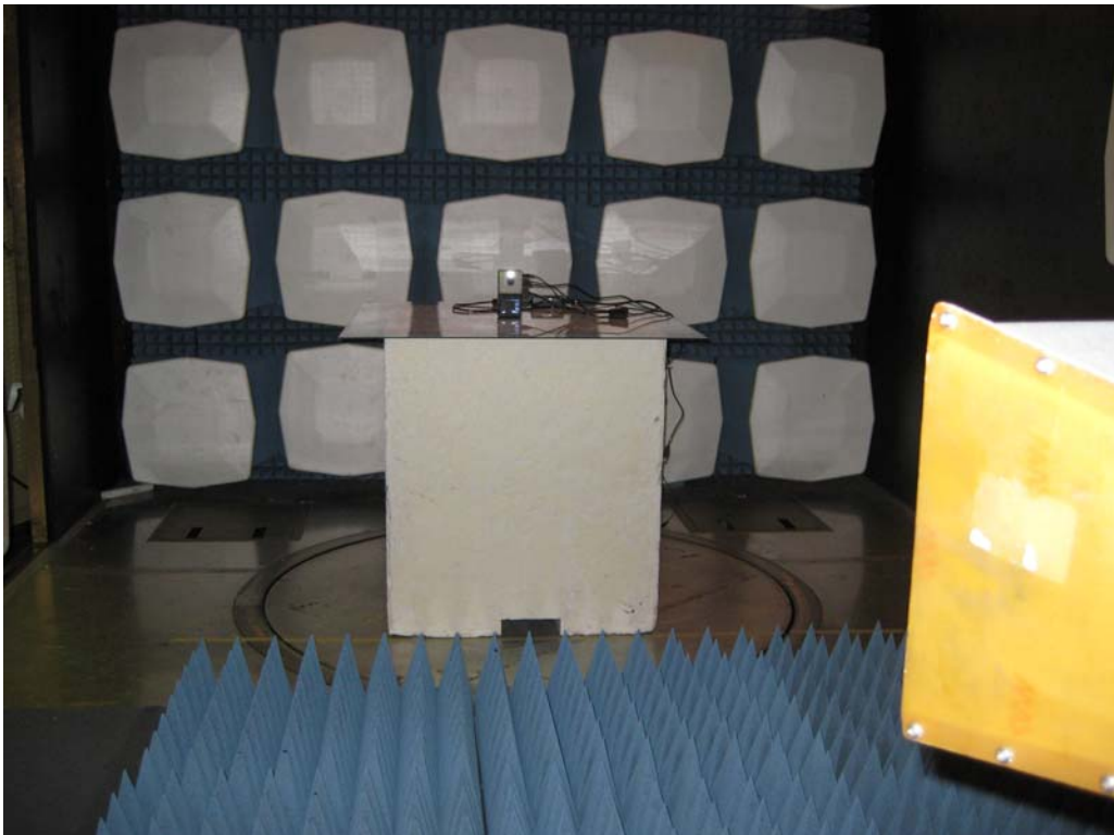
Radiated Emissions #2
