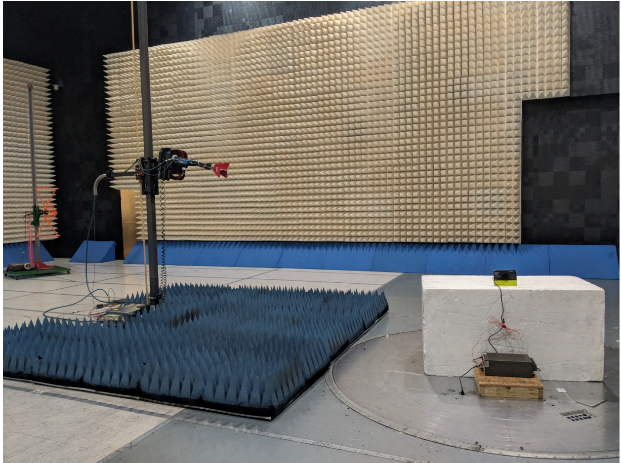
Radiated emissions, 1-18GHz, idle
