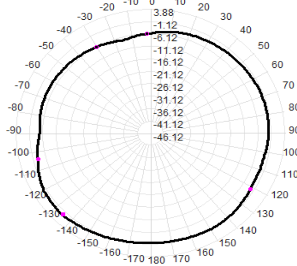
Total(H-XY), Max= 0.04dBi, CirD=7.38
