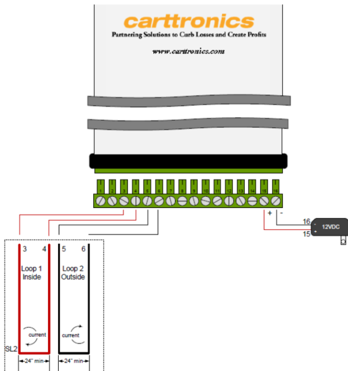
Fig.4 Sentry Connection Diagram
