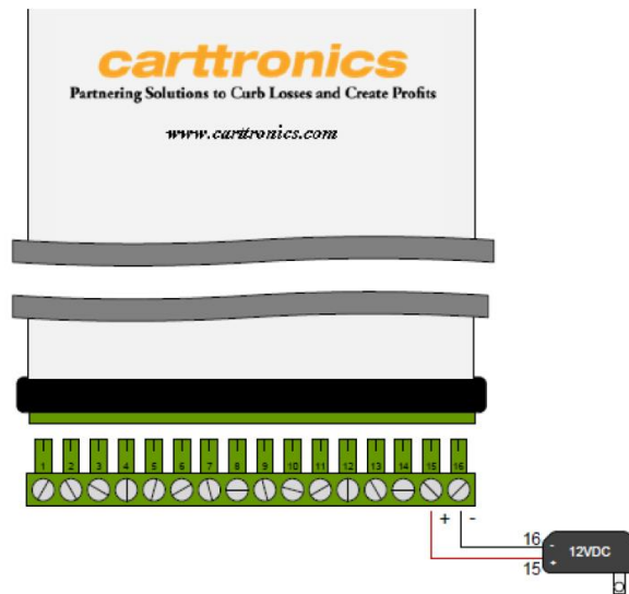
Fig.3 Permit Issuer Diagram
