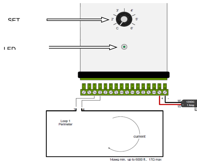
Fig.2 TX2 Connection Diagram
