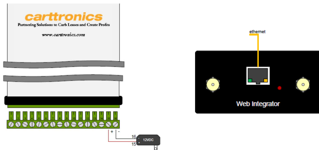
Fig.1 Web Integrator Connection Diagram
