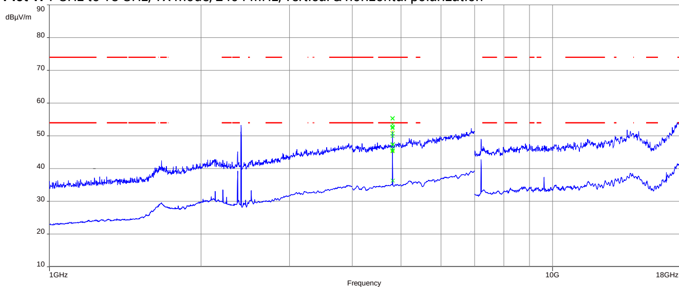
Plot 1: 1 GHz to 18 GHz, TX mode, 2404 MHz, vertical & horizontal polarization
