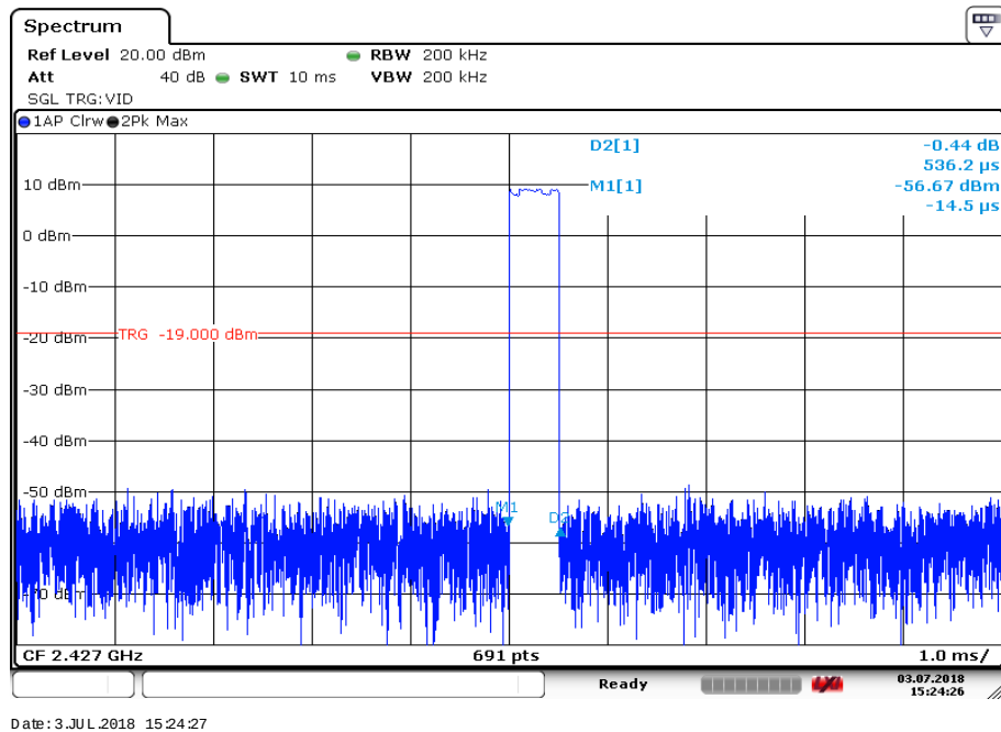
Plot 2: 2427 MHz, Zero span, pulse width
