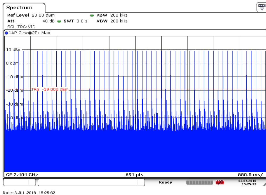
Plot 4: 2404 MHz, 8.8 s sweep
