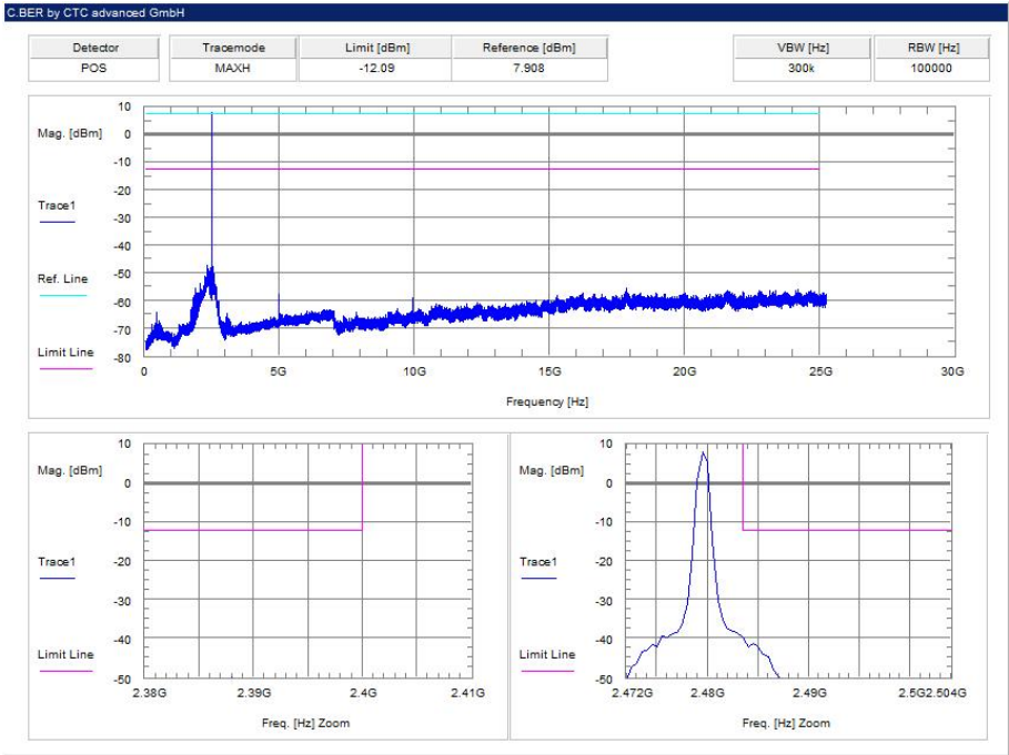
Plot 3: highest channel – 2479.3 MHz
