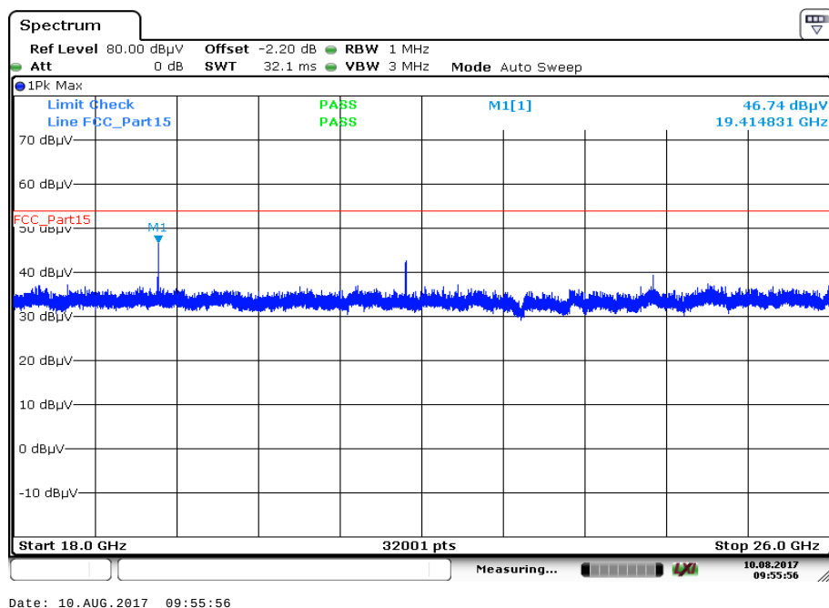
Plot 4: 18 GHz to 26 GHz, TX mode, 2427.0 MHz, vertical & horizontal polarization
