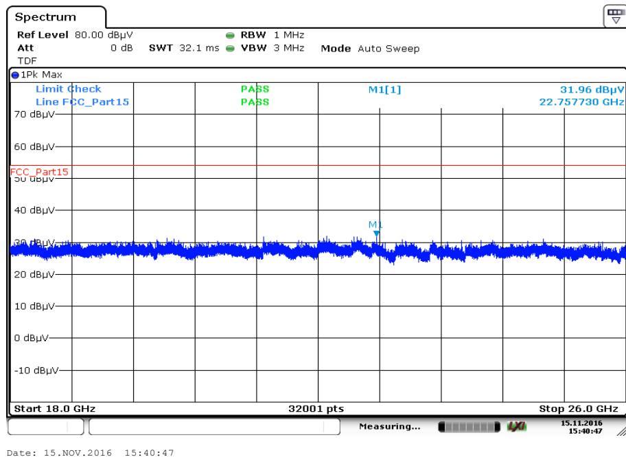
Plot 4: 18 GHz to 26 GHz, TX mode, 2404.0 MHz, vertical & horizontal polarization
