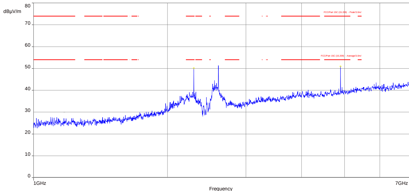
Plot 5: 1 GHz to 7 GHz, TX mode, 2447.0 MHz, vertical & horizontal polarization
