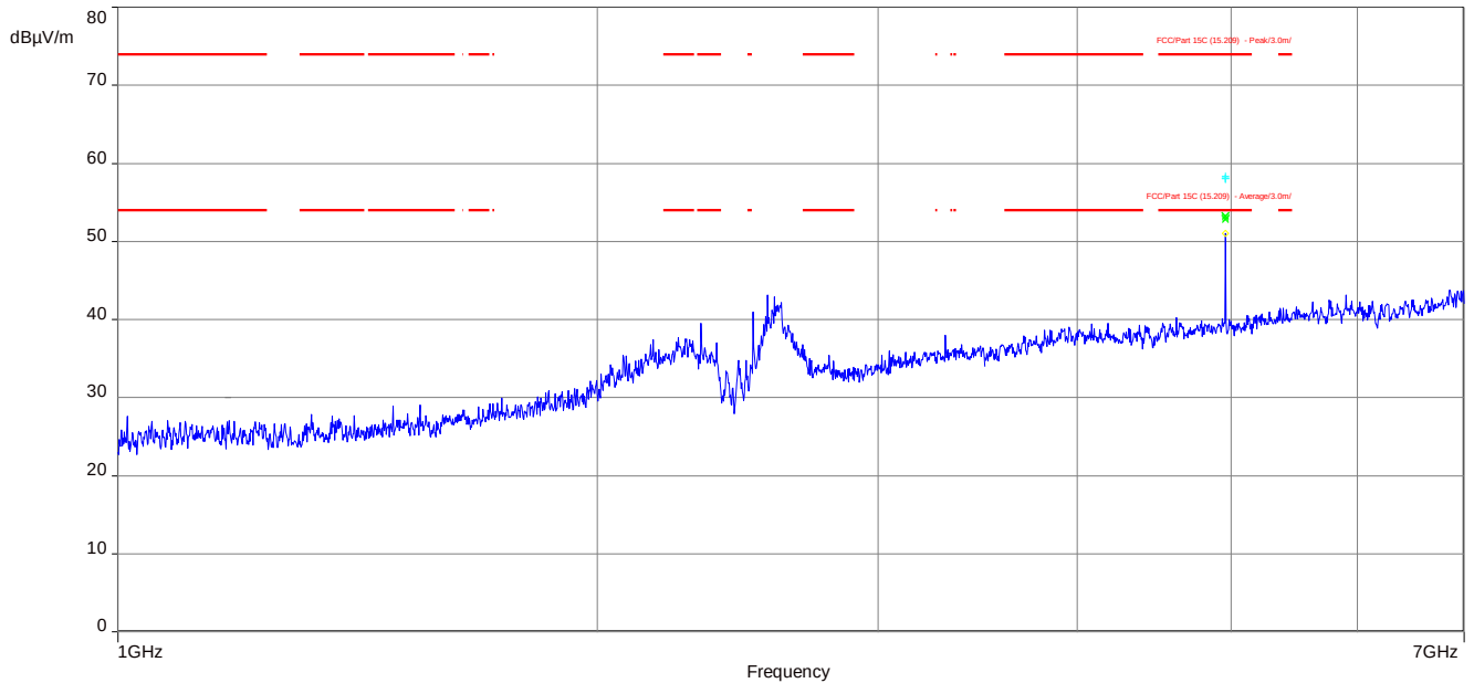
Plot 9: 1 GHz to 7 GHz, TX mode, 2479.3 MHz, vertical & horizontal polarization
