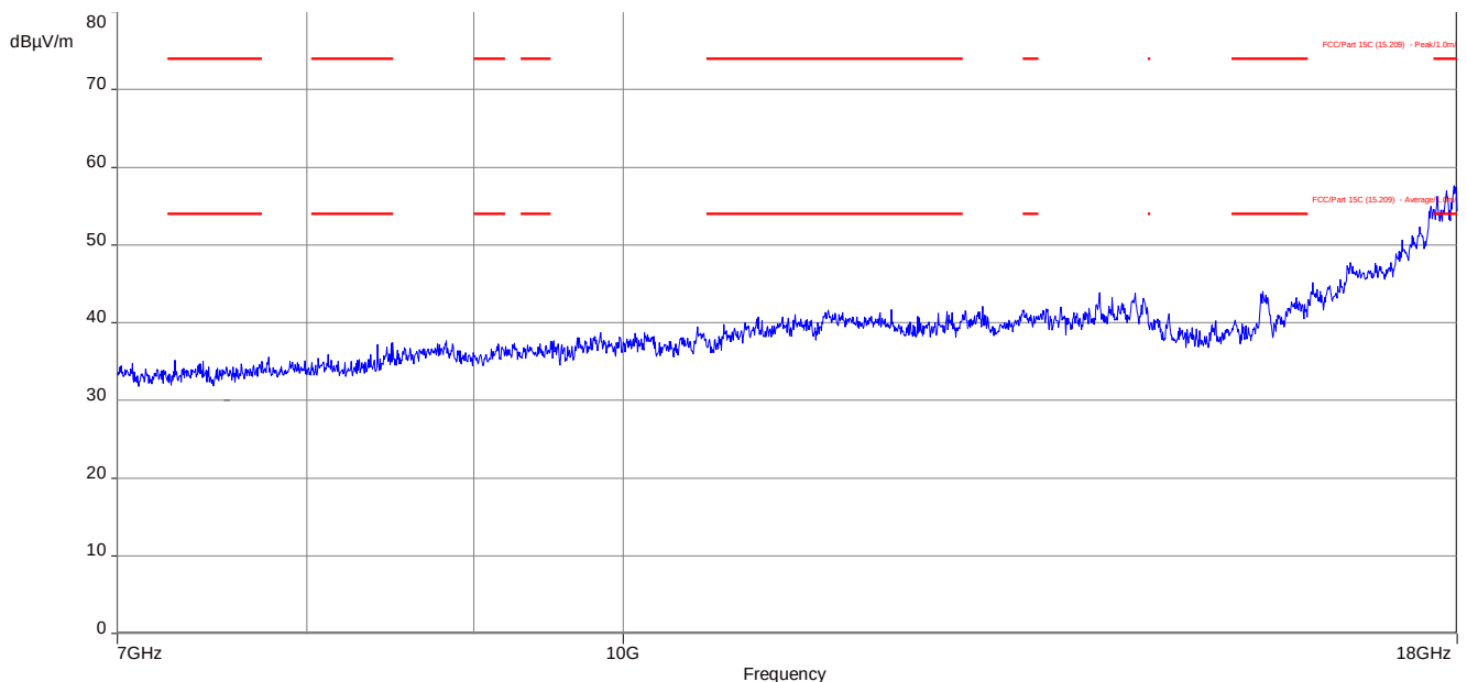
Plot 10: 7 GHz to 18 GHz, TX mode, 2479.3 MHz, vertical & horizontal polarization
