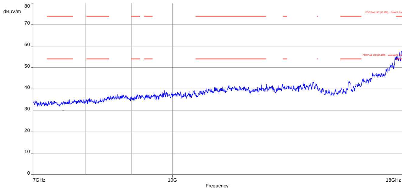
Plot 6: 7 GHz to 18 GHz, TX mode, 2447.0 MHz, vertical & horizontal polarization
