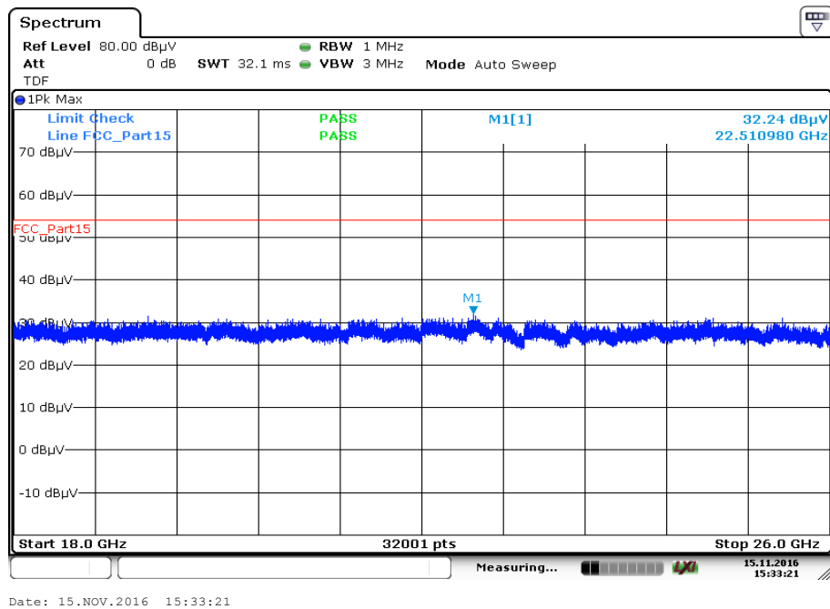
Plot 8: 18 GHz to 26 GHz, TX mode, 2447.0 MHz, vertical & horizontal polarization
