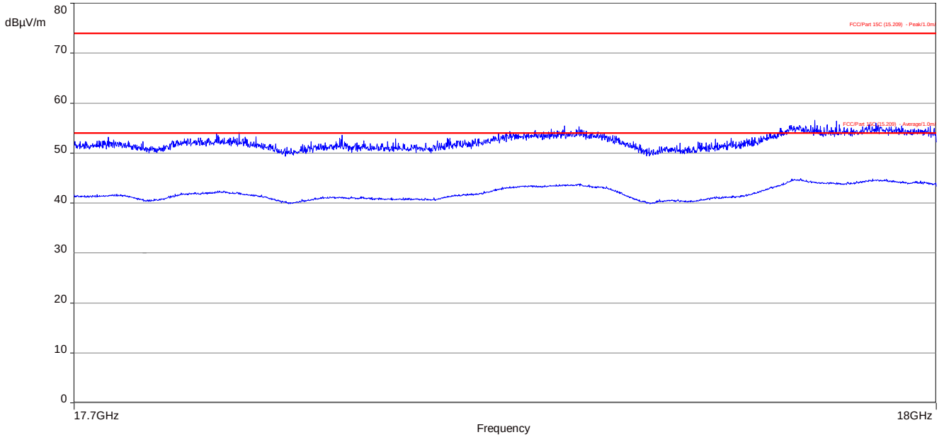
Plot 7: 17.7 GHz to 18 GHz, TX mode, 2447.0 MHz, vertical & horizontal polarization
