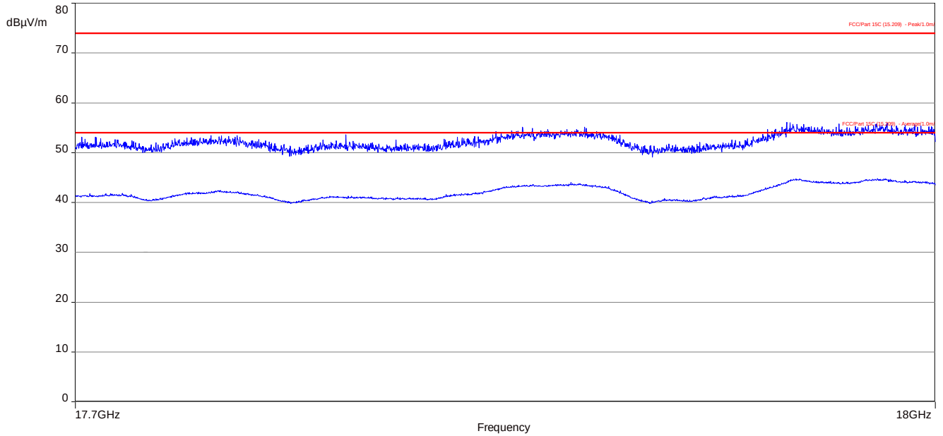
Plot 3: 17.7 GHz to 18 GHz, TX mode, 2404.0 MHz, vertical & horizontal polarization
