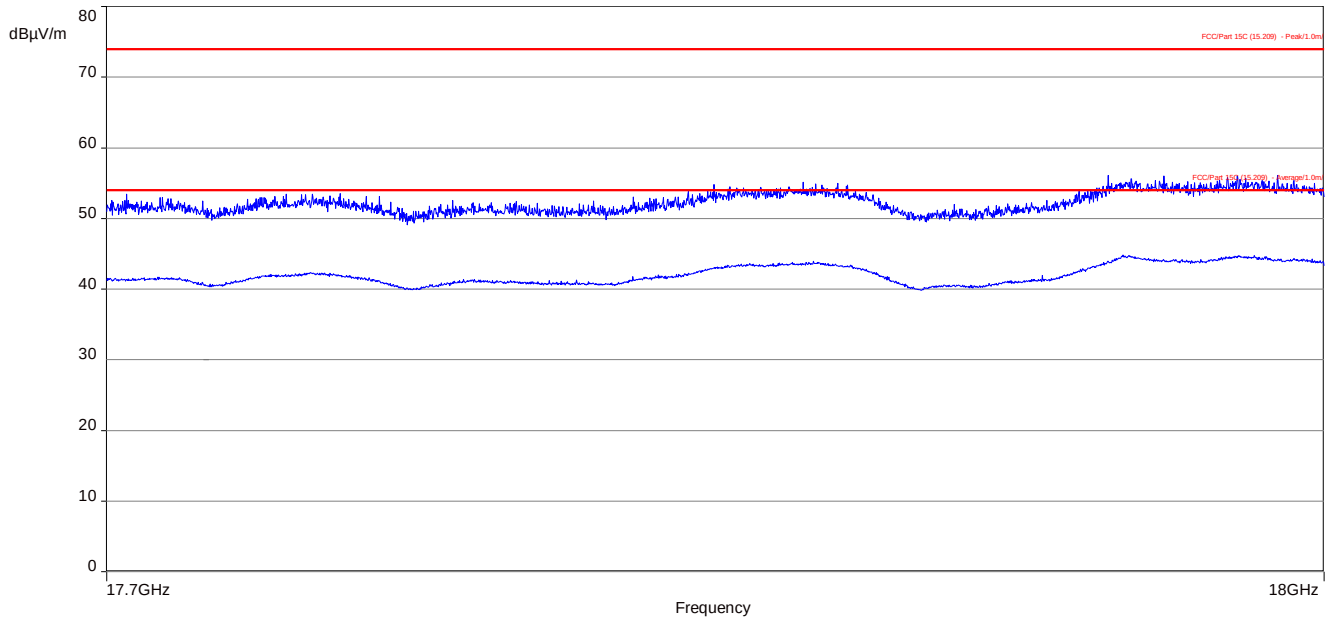
Plot 11: 17.7 GHz to 18 GHz, TX mode, 2479.3 MHz, vertical & horizontal polarization
