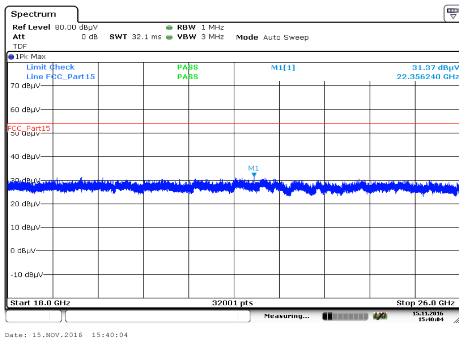
Plot 12: 18 GHz to 26 GHz, TX mode, 2479.3 MHz, vertical & horizontal polarization
