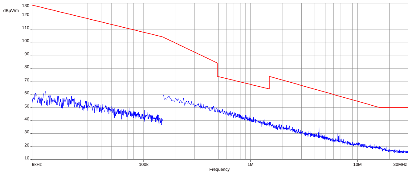
Plot 3: 9 kHz to 30 MHz, TX Mode, high channel, transmit mode
