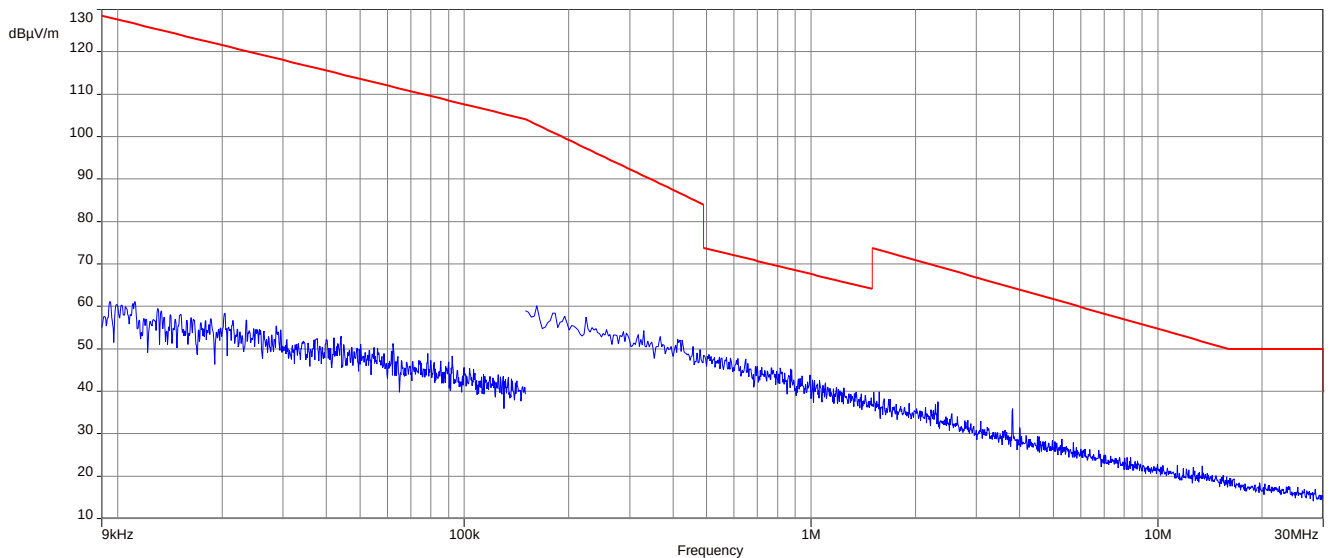
Plot 2: 9 kHz to 30 MHz, TX Mode, mid channel, transmit mode
