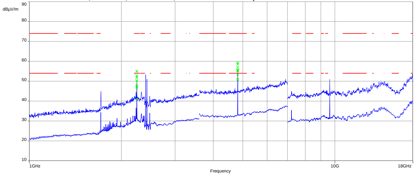
Plot 1: 1 GHz to 18 GHz, TX mode, low channel, vertical & horizontal polarization
