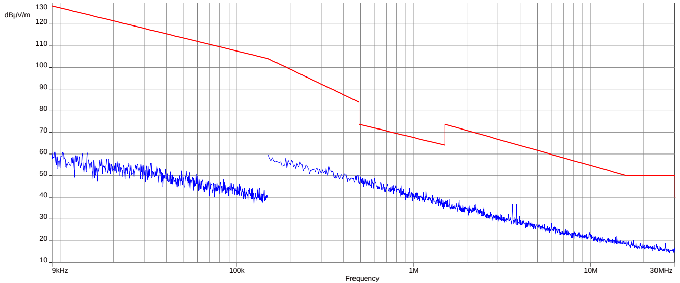
Plot 1: 9 kHz to 30 MHz, TX Mode, low channel, transmit mode
