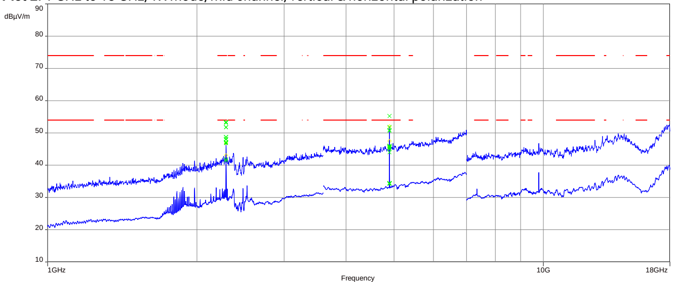
Plot 2: 1 GHz to 18 GHz, TX mode, mid channel, vertical & horizontal polarization
