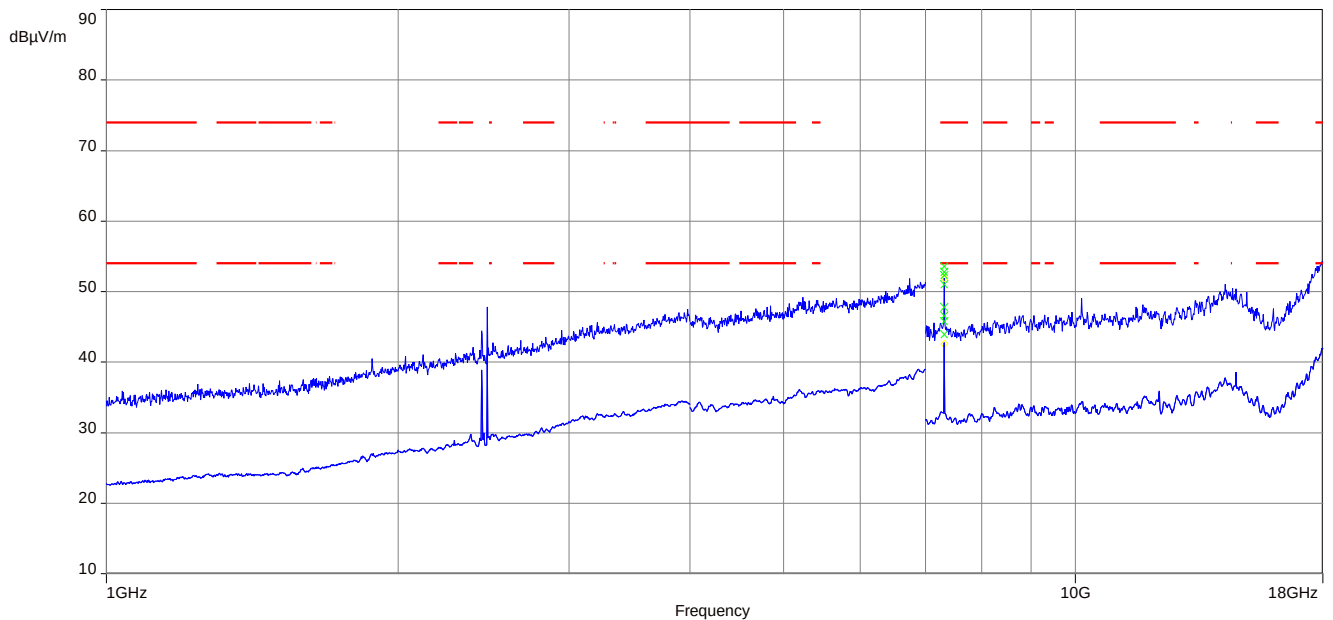
Plot 2: 1 GHz to 18 GHz, TX mode, 2440 MHz, vertical & horizontal polarization, 1 Msps
