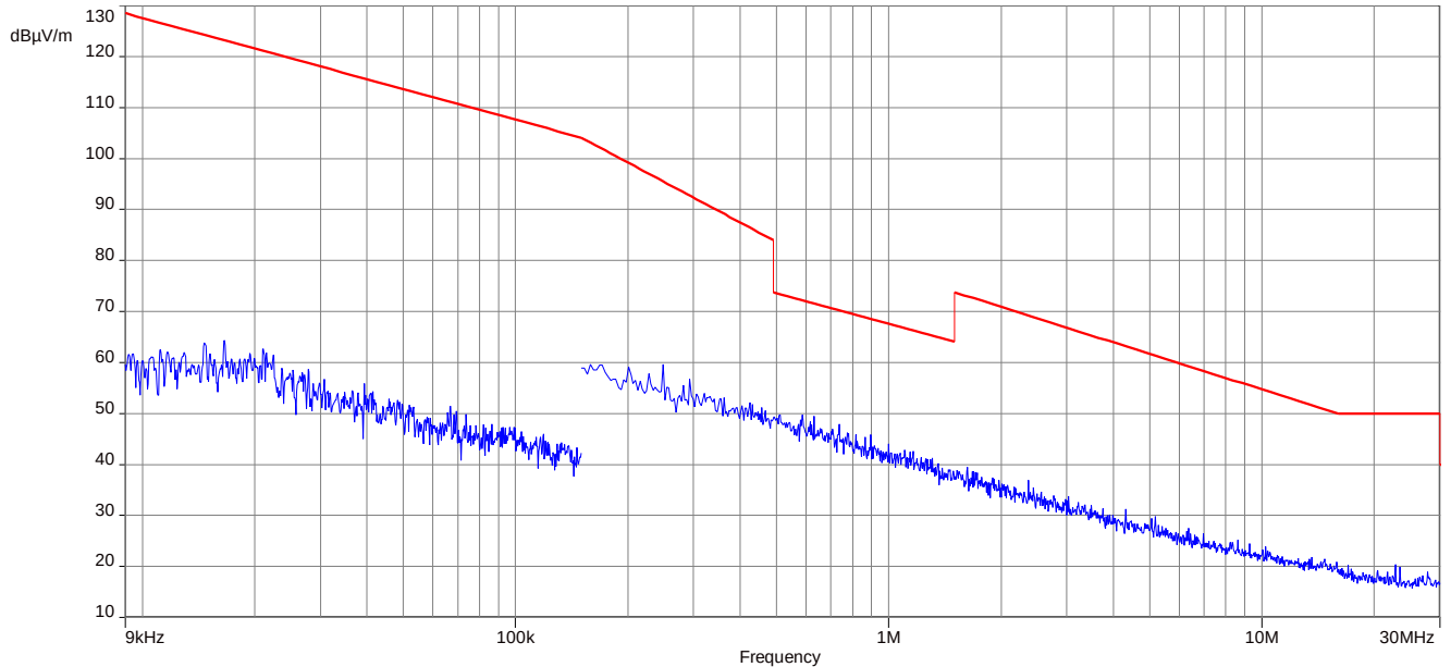
Plot 1: 9 kHz to 30 MHz, 2402 MHz, transmit mode, 1 Msps
