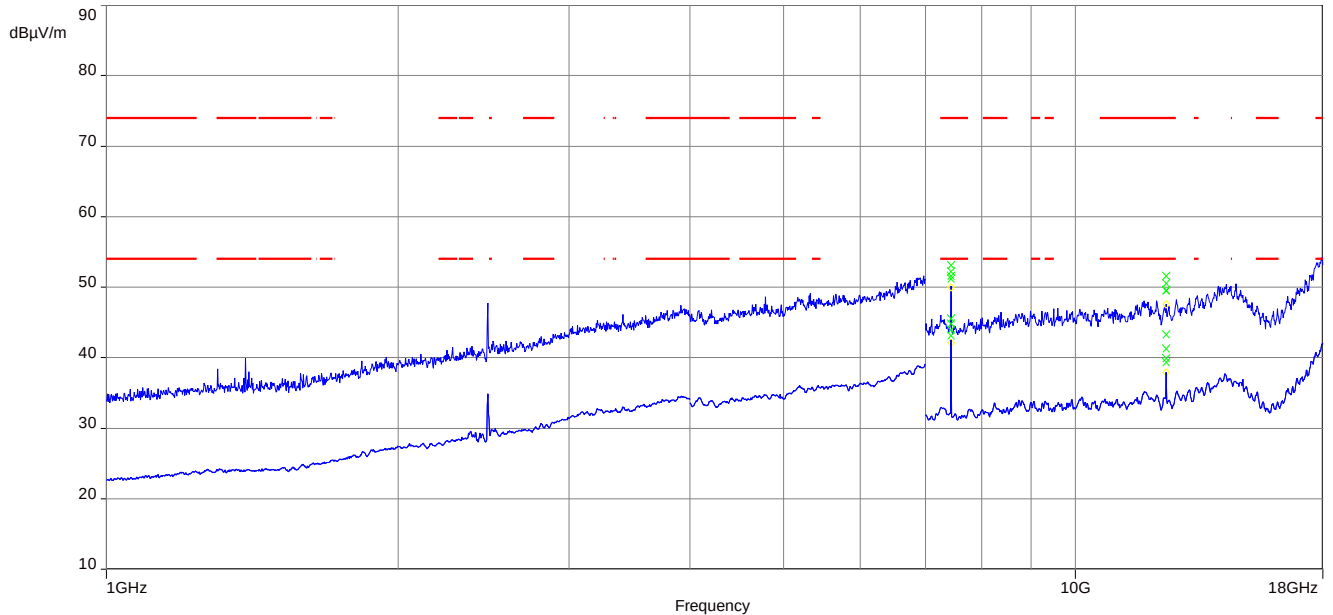
Plot 3: 1 GHz to 18 GHz, TX mode, 2480 MHz, vertical & horizontal polarization, 1 Msps
