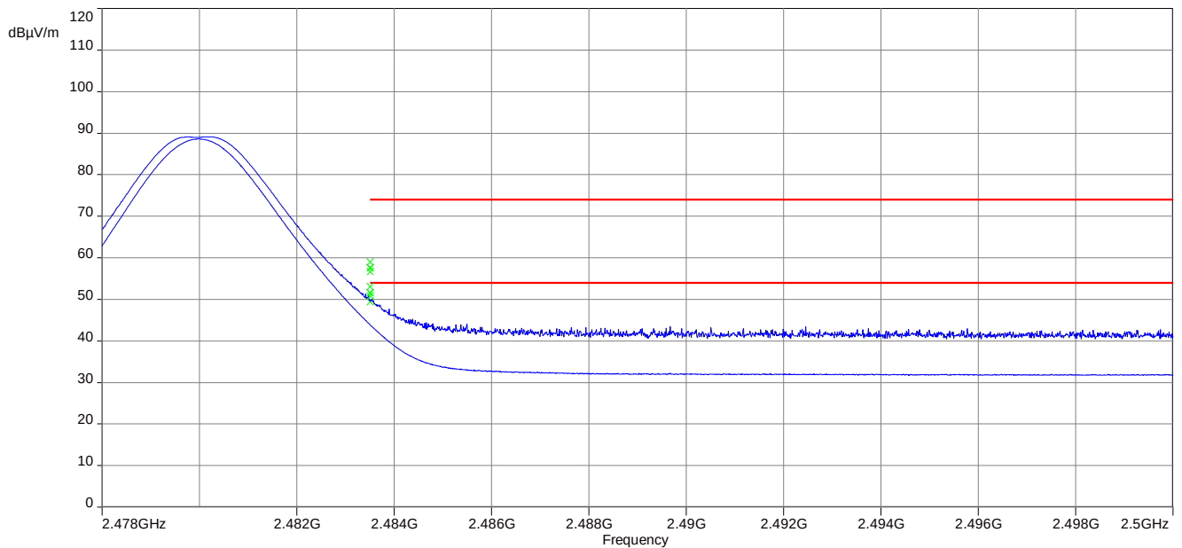
Plot 2: Upper restricted band, 1 Msp
