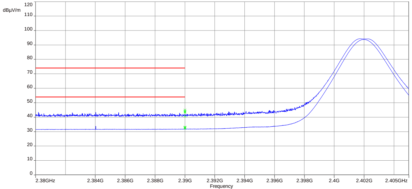
Plot 1: Lower restricted band, 1 Msp
