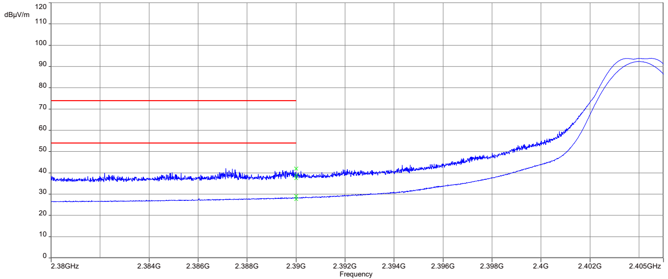
Plot 7: Lower restricted band, 2 Msps, Horizontal plane
