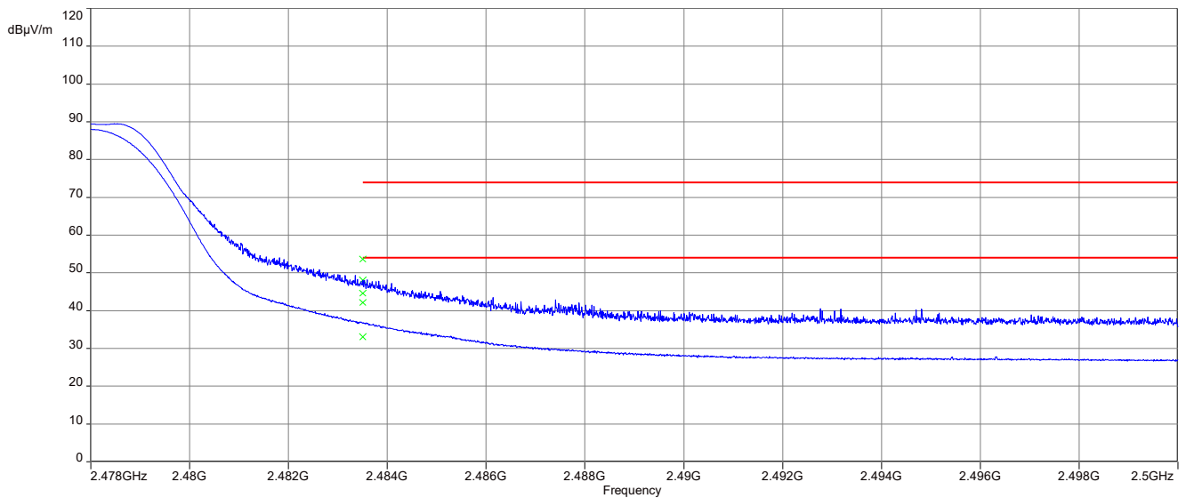
Plot 8: Upper restricted band, 2 Msps, Horizontal plane
