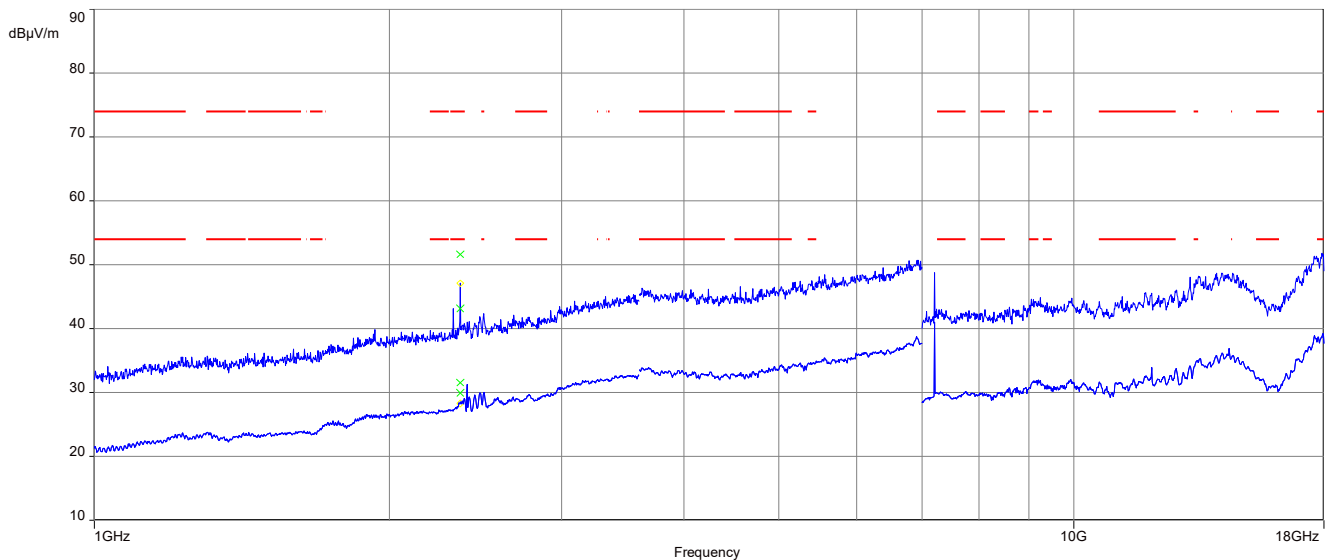
Plot 4: 1 GHz to 18 GHz, TX mode, 2402 MHz, vertical & horizontal polarization, 1 Msps, Horizontal Plane
