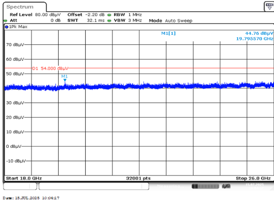
Plot 7: 18 GHz to 26 GHz, TX mode, 2480 MHz, vertical & horizontal polarization, 1 Msps
