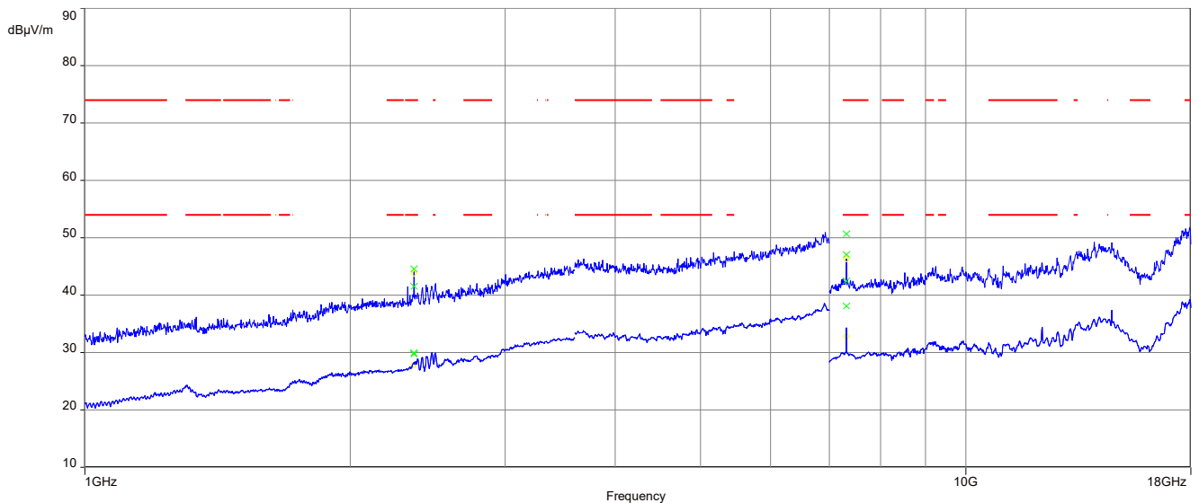
Plot 9: 1 GHz to 18 GHz, TX mode, 2440 MHz, vertical & horizontal polarization, 2 Msps, Vertical Plane
