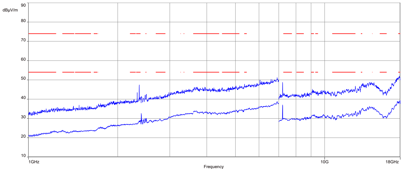
Plot 11: 1 GHz to 18 GHz, TX mode, 2404 MHz, vertical & horizontal polarization, 2 Msps, Horizontal Plane
