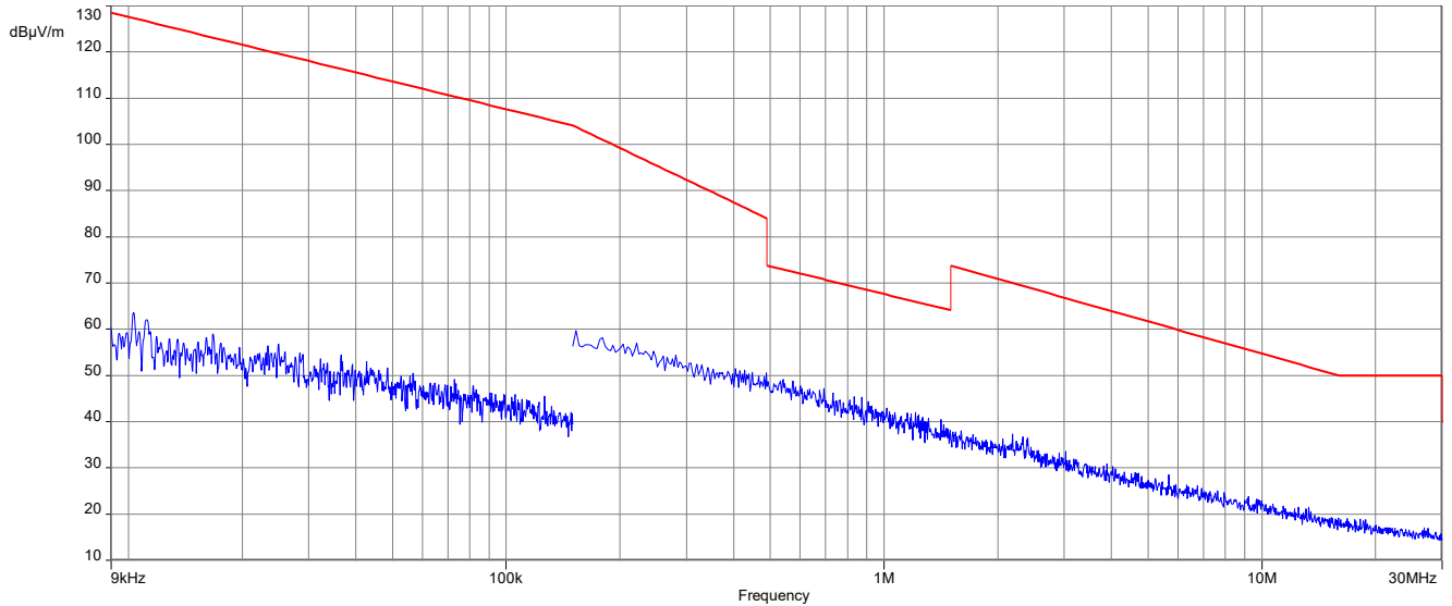
Plot 11: 9 kHz to 30 MHz, 2440 MHz, transmit mode, 2 Msps, Horizontal Plane
