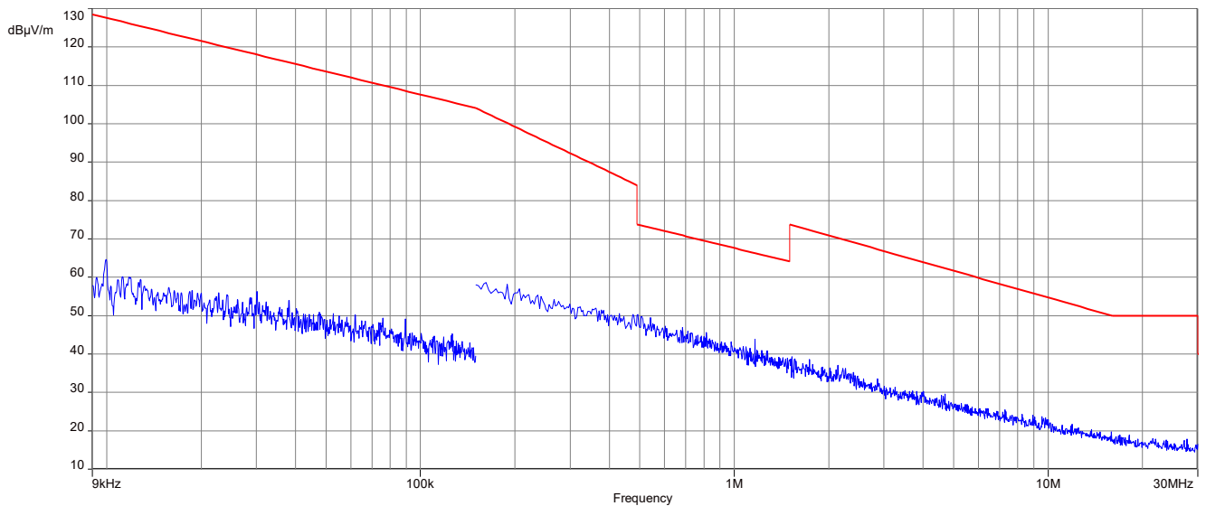
Plot 10: 9 kHz to 30 MHz, 2404 MHz, transmit mode, 2 Msps, Horizontal Plane
