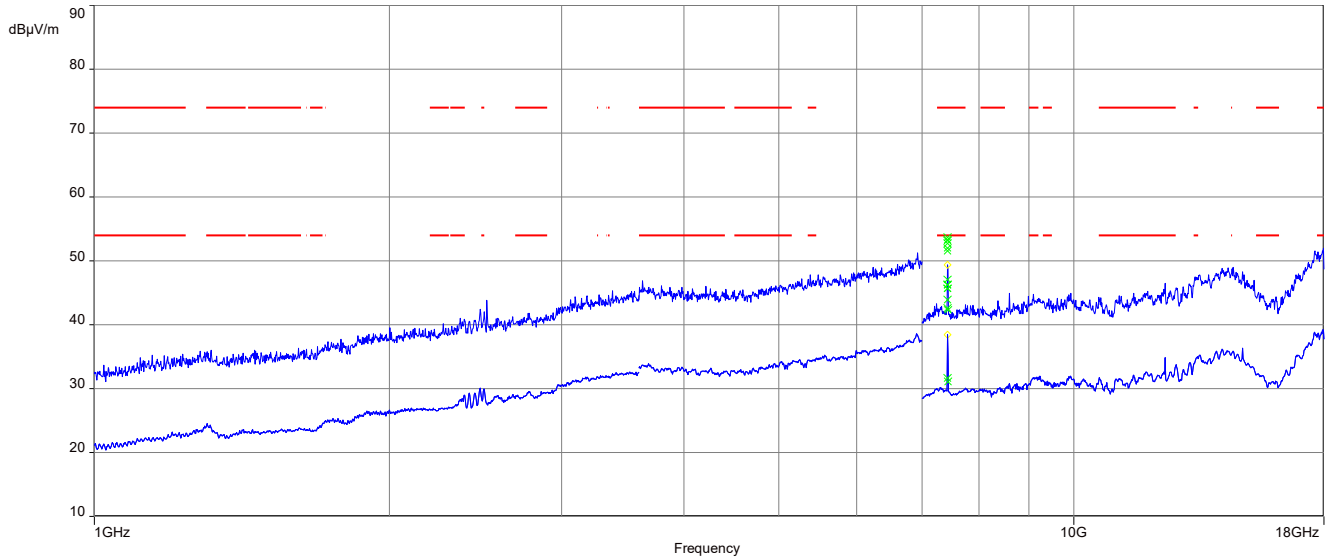
Plot 10: 1 GHz to 18 GHz, TX mode, 2478 MHz, vertical & horizontal polarization, 2 Msps, Vertical Plane
