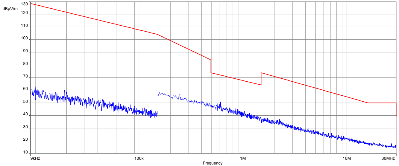
Plot 1: 9 kHz to 30 MHz, 2402 MHz, transmit mode, 1 Msps, Vertical Plane
