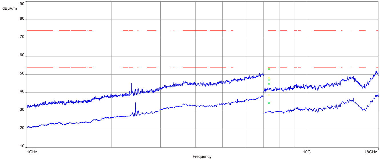
Plot 5: 1 GHz to 18 GHz, TX mode, 2440 MHz, vertical & horizontal polarization, 1 Msps, Horizontal Plane
