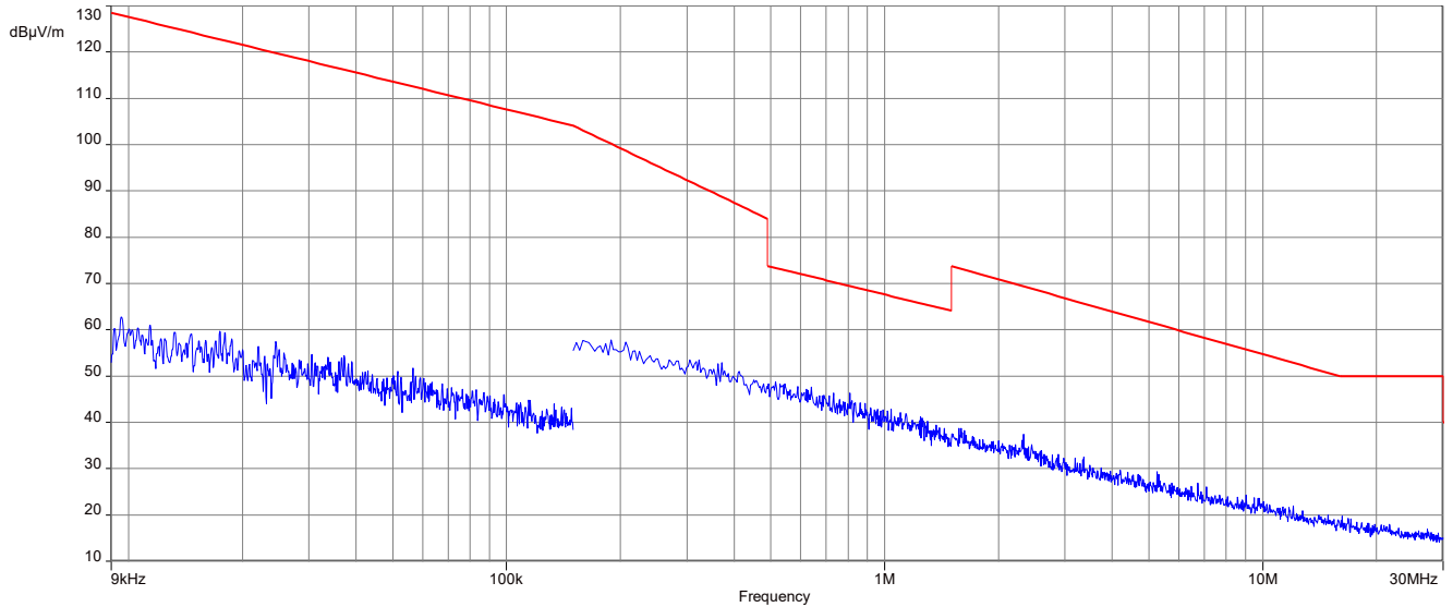
Plot 7: 9 kHz to 30 MHz, 2402 MHz, transmit mode, 1 Msps, Horizontal Plane
