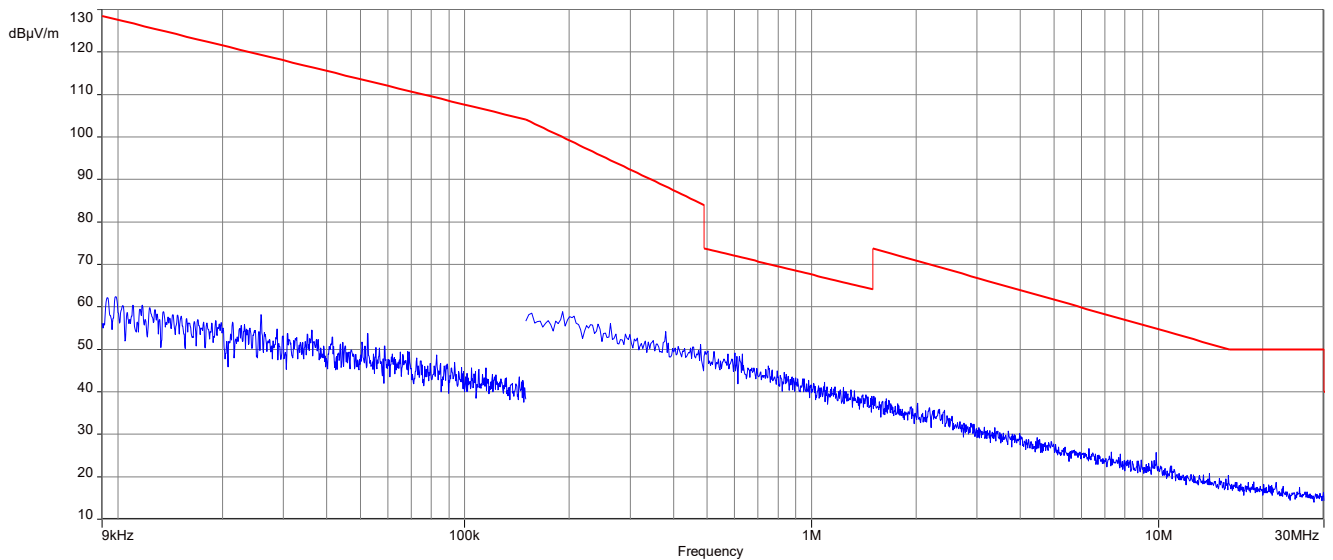
Plot 2: 9 kHz to 30 MHz, 2440 MHz, transmit mode, 1 Msps, Vertical Plane
