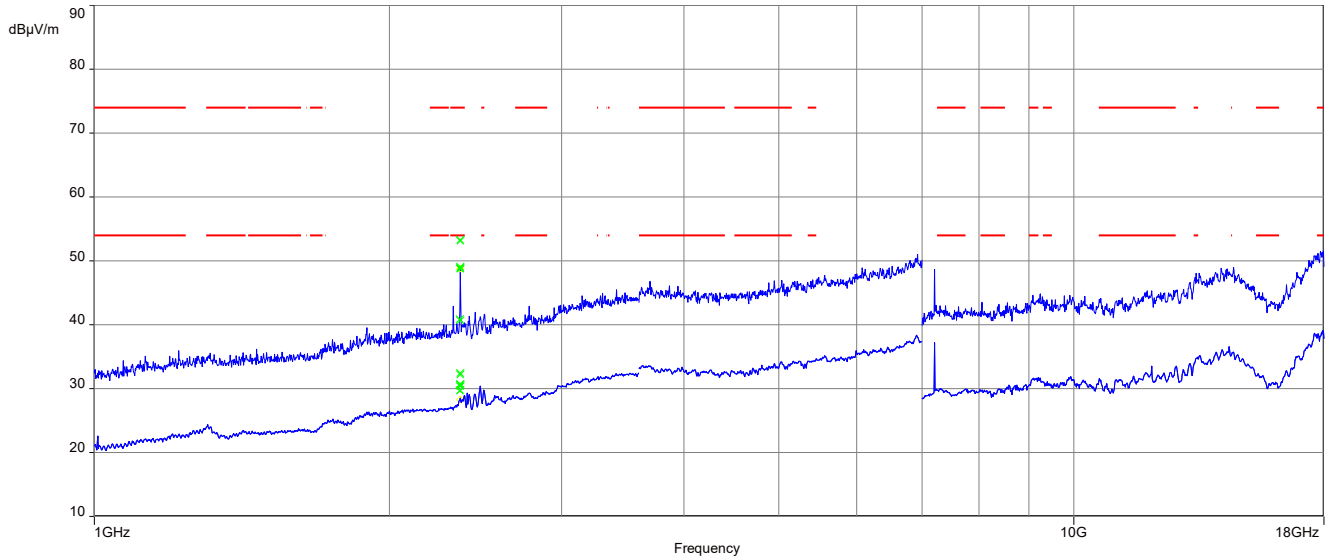
Plot 8: 1 GHz to 18 GHz, TX mode, 2404 MHz, vertical & horizontal polarization, 2 Msps, Vertical Plane
