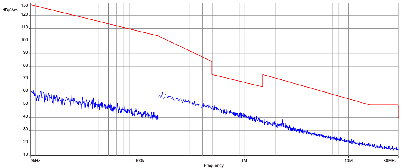
Plot 4: 9 kHz to 30 MHz, 2404 MHz, transmit mode, 2 Msps, Vertical Plane
