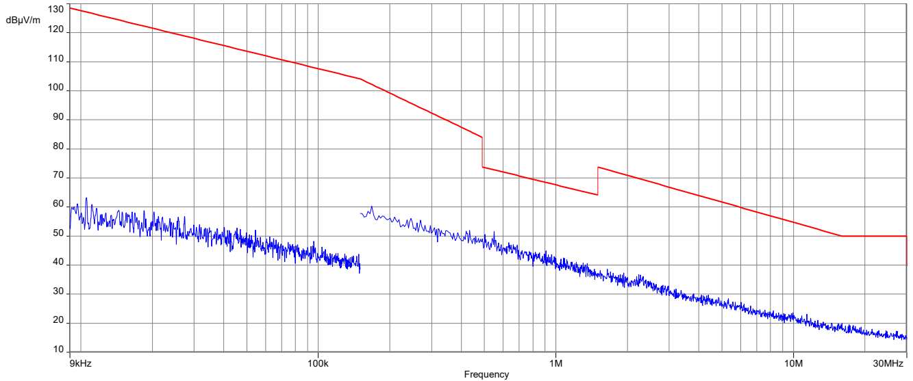
Plot 3: 9 kHz to 30 MHz, 2480 MHz, transmit mode, 1 Msps, Vertical Plane
