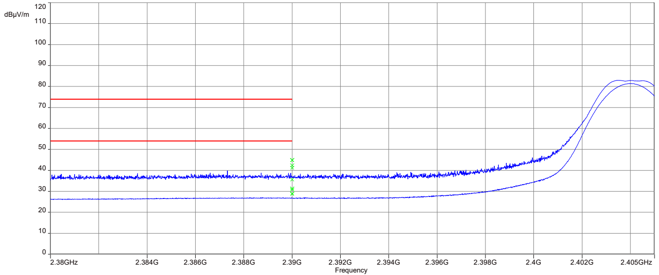
Plot 3: Lower restricted band, 2 Msps, Vertical plane
