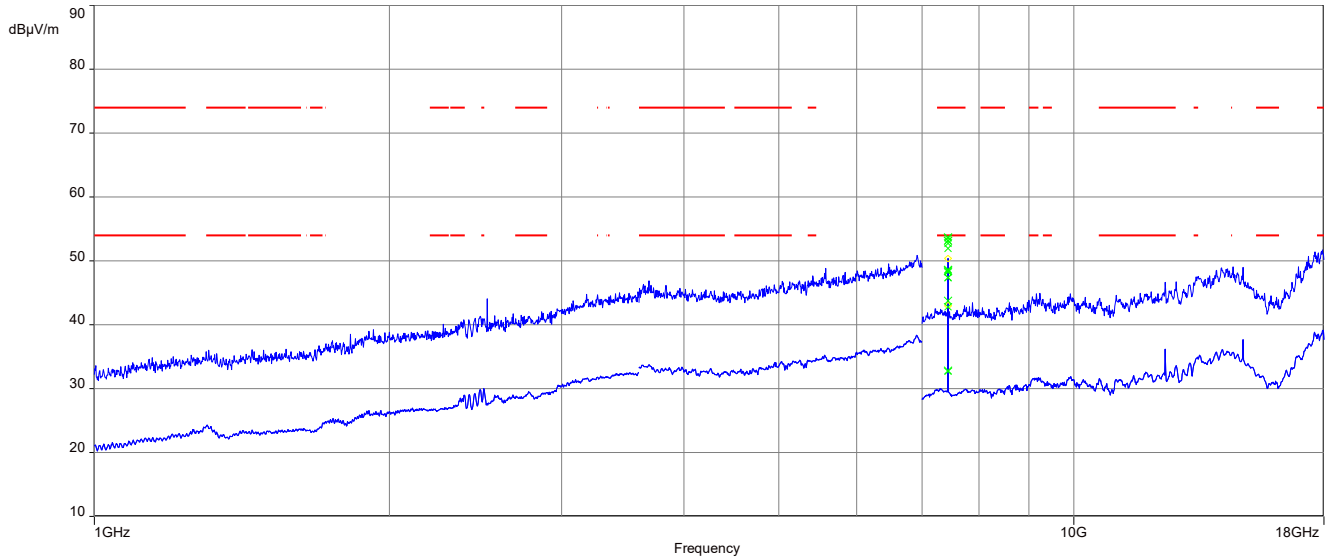
Plot 3: 1 GHz to 18 GHz, TX mode, 2480 MHz, vertical & horizontal polarization, 1 Msps, Vertical Plane
