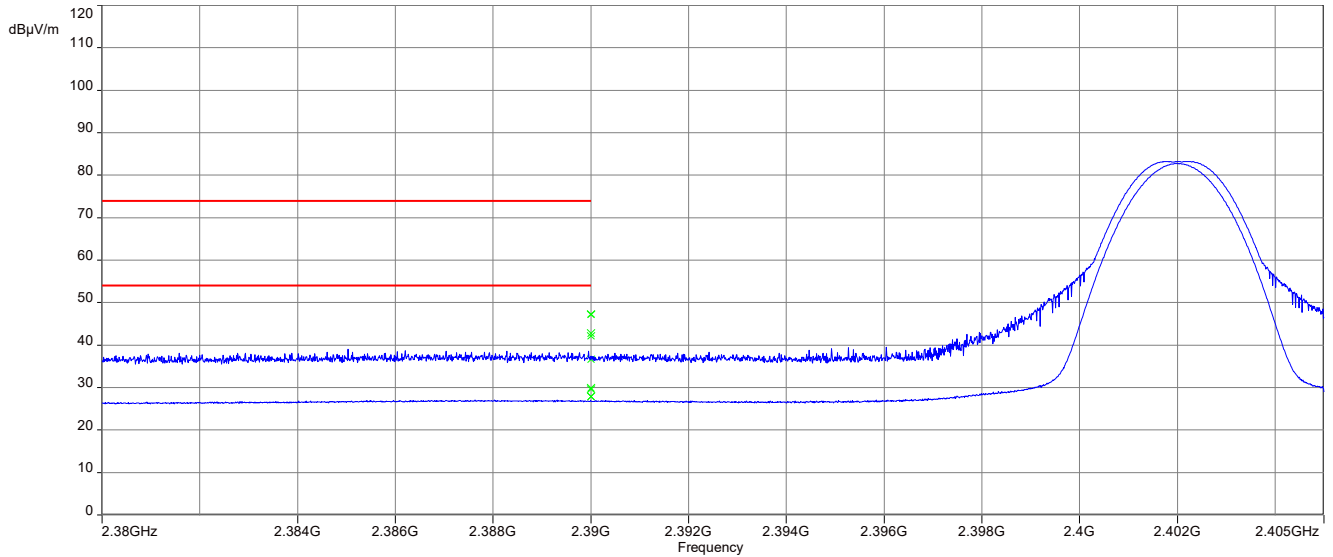
Plot 1: Lower restricted band, 1 Msps, Vertical plane
