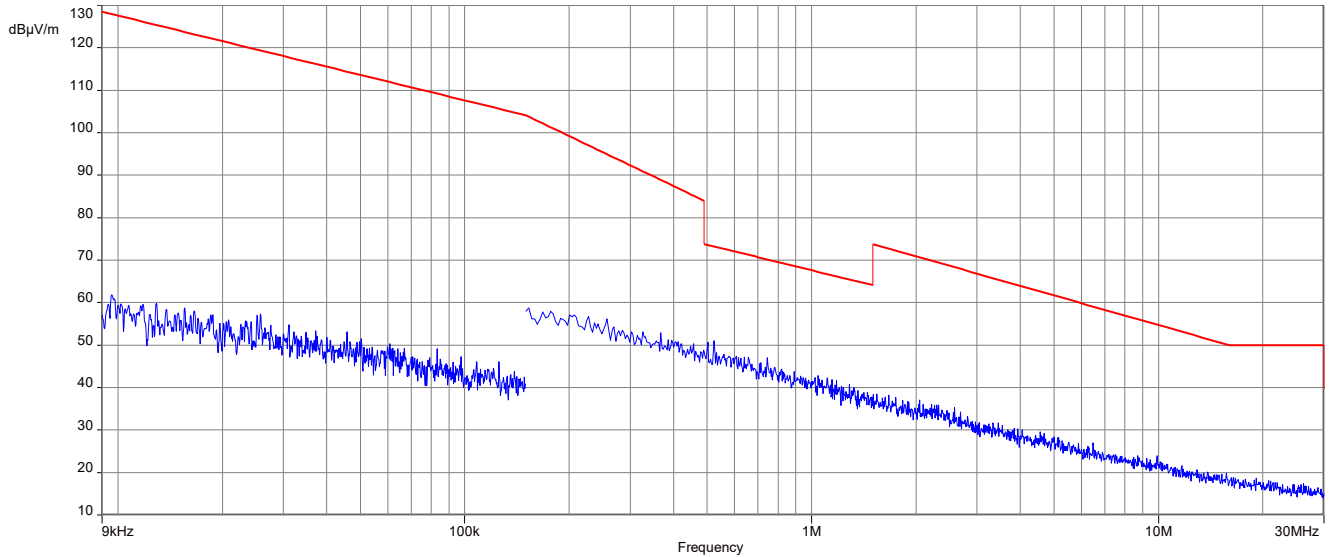
Plot 9: 9 kHz to 30 MHz, 2480 MHz, transmit mode, 1 Msps, Horizontal Plane
