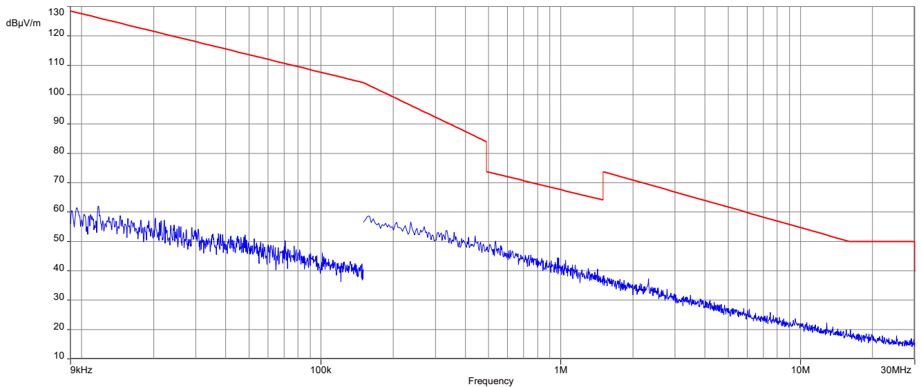
Plot 8: 9 kHz to 30 MHz, 2440 MHz, transmit mode, 1 Msps, Horizontal Plane
