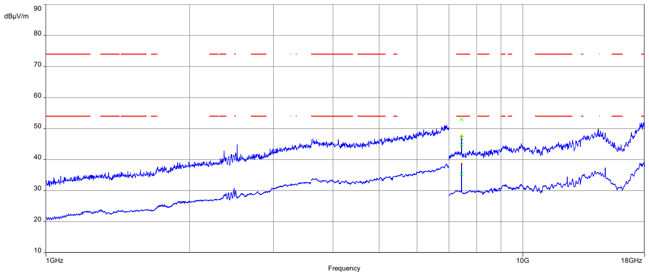
Plot 6: 1 GHz to 18 GHz, TX mode, 2480 MHz, vertical & horizontal polarization, 1 Msps, Horizontal Plane
