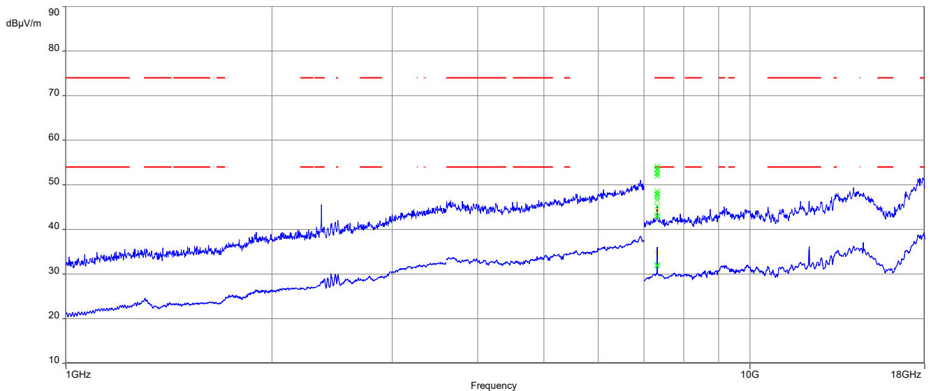
Plot 2: 1 GHz to 18 GHz, TX mode, 2440 MHz, vertical & horizontal polarization, 1 Msps, Vertical Plane
