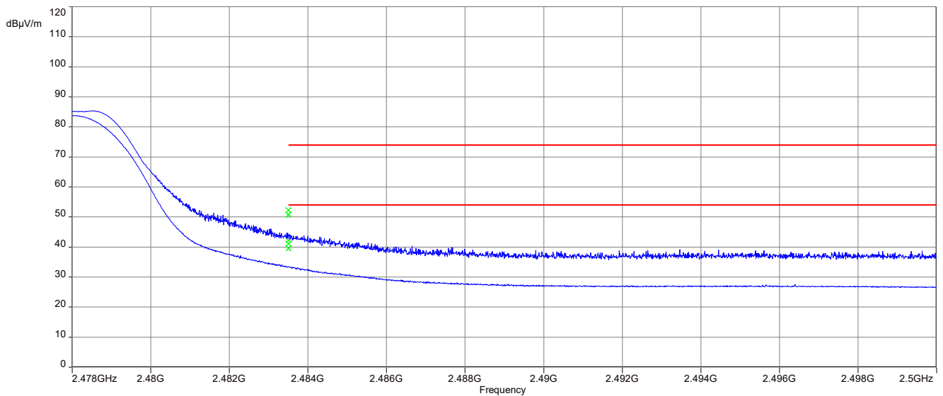
Plot 4: Upper restricted band, 2 Msps, Vertical plane
