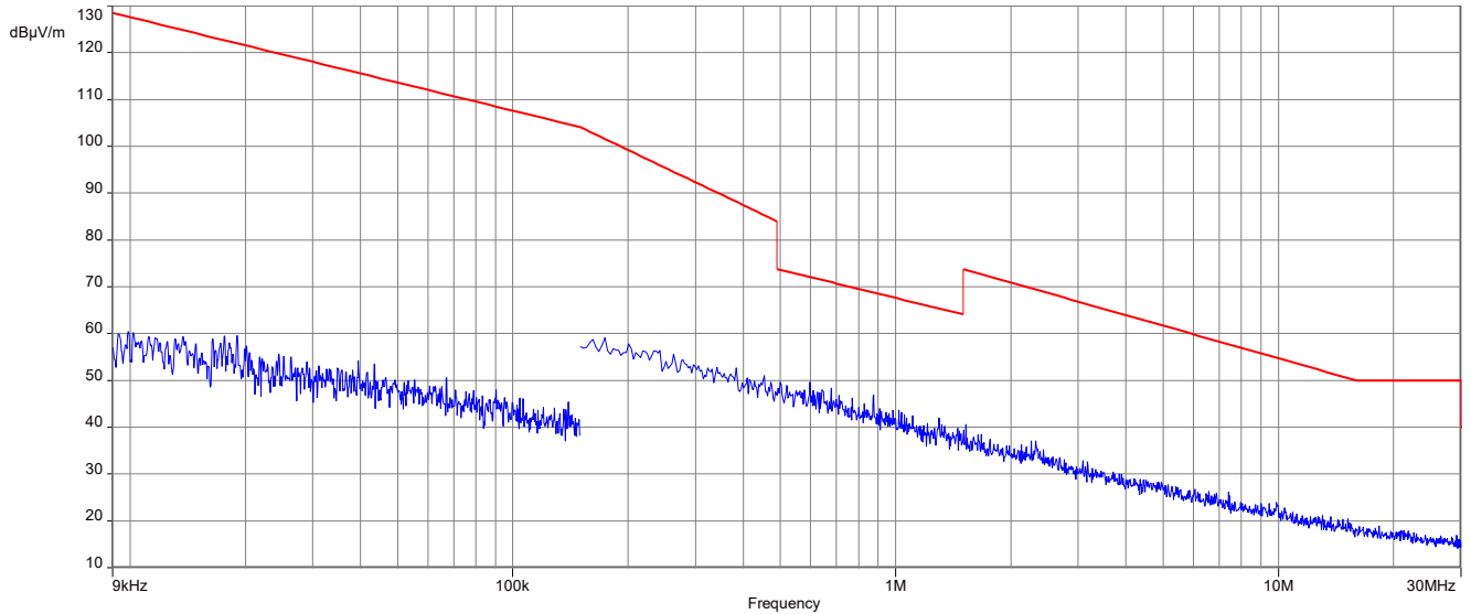
Plot 5: 9 kHz to 30 MHz, 2440 MHz, transmit mode, 2 Msps, Vertical Plane
