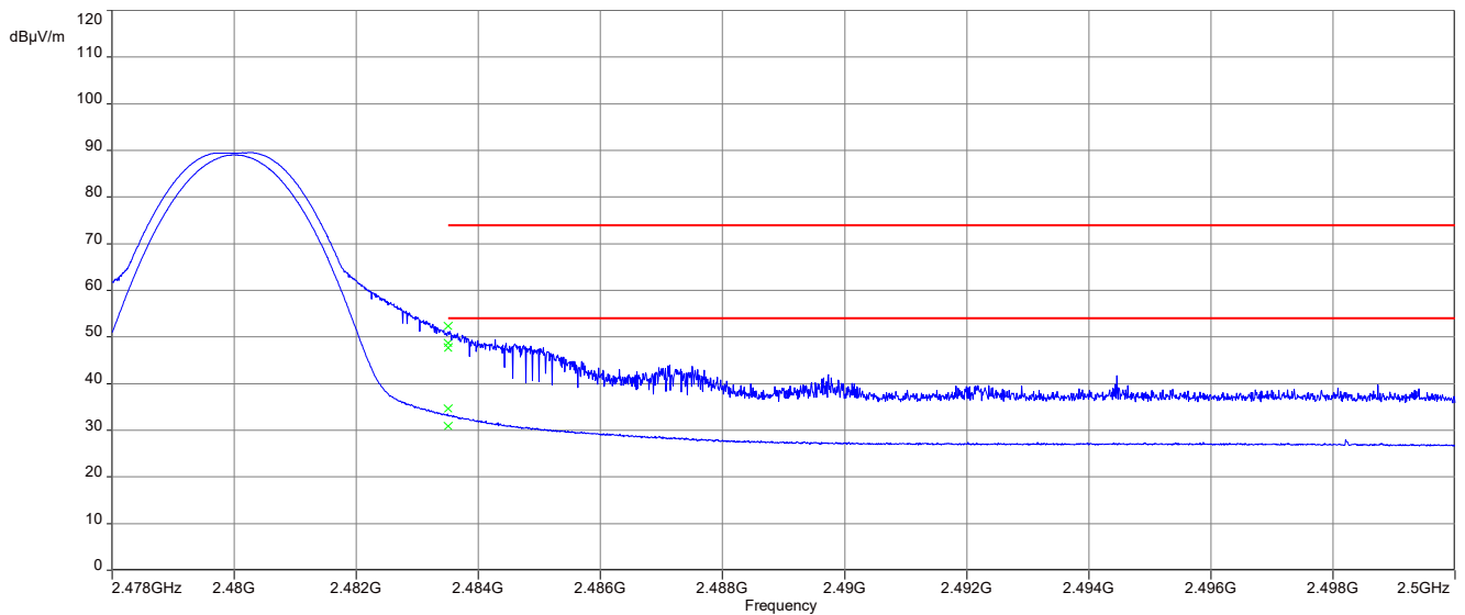
Plot 6: Upper restricted band, 1 Msps, Horizontal plane
