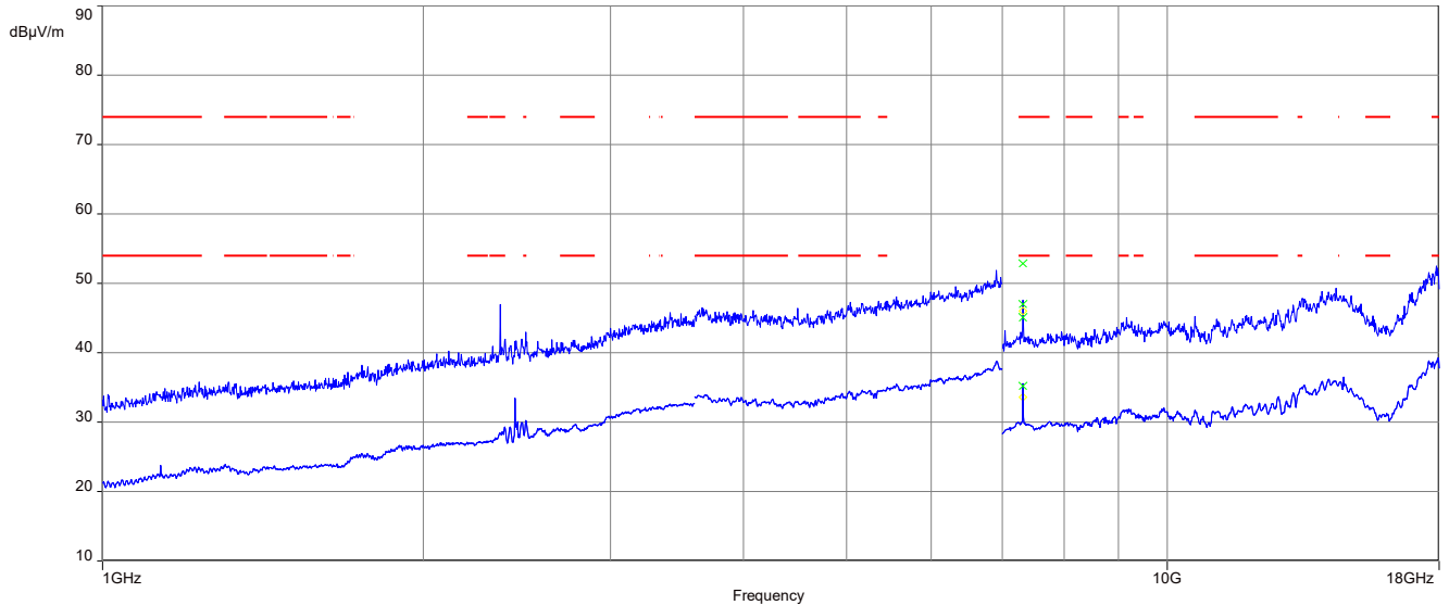
Plot 12: 1 GHz to 18 GHz, TX mode, 2440 MHz, vertical & horizontal polarization, 2 Msps, Horizontal Plane
