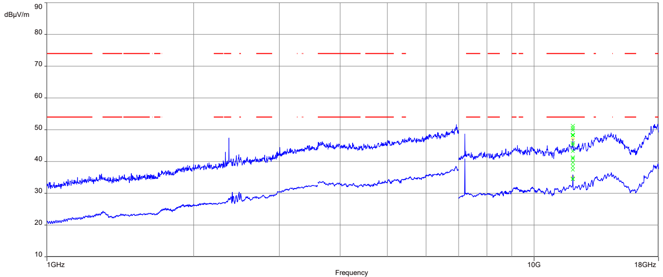
Plot 1: 1 GHz to 18 GHz, TX mode, 2402 MHz, vertical & horizontal polarization, 1 Msps, Vertical Plane
