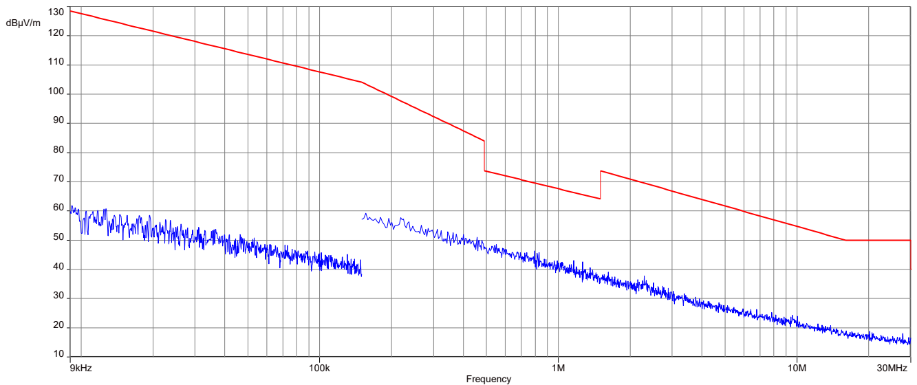
Plot 6: 9 kHz to 30 MHz, 2478 MHz, transmit mode, 2 Msps, Vertical Plane
