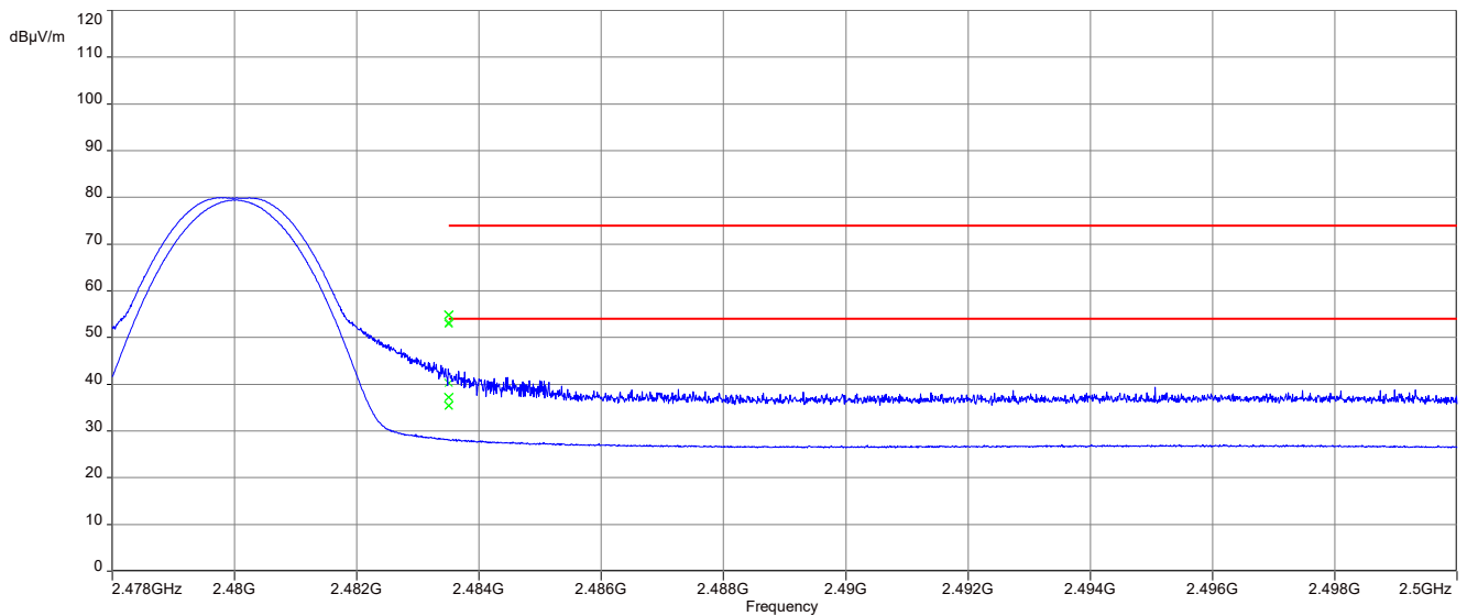
Plot 2: Upper restricted band, 1 Msps, Vertical plane
