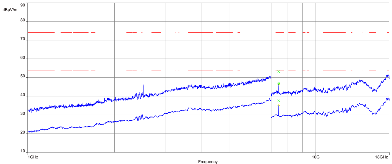
Plot 13: 1 GHz to 18 GHz, TX mode, 2478 MHz, vertical & horizontal polarization, 2 Msps, Horizontal Plane
