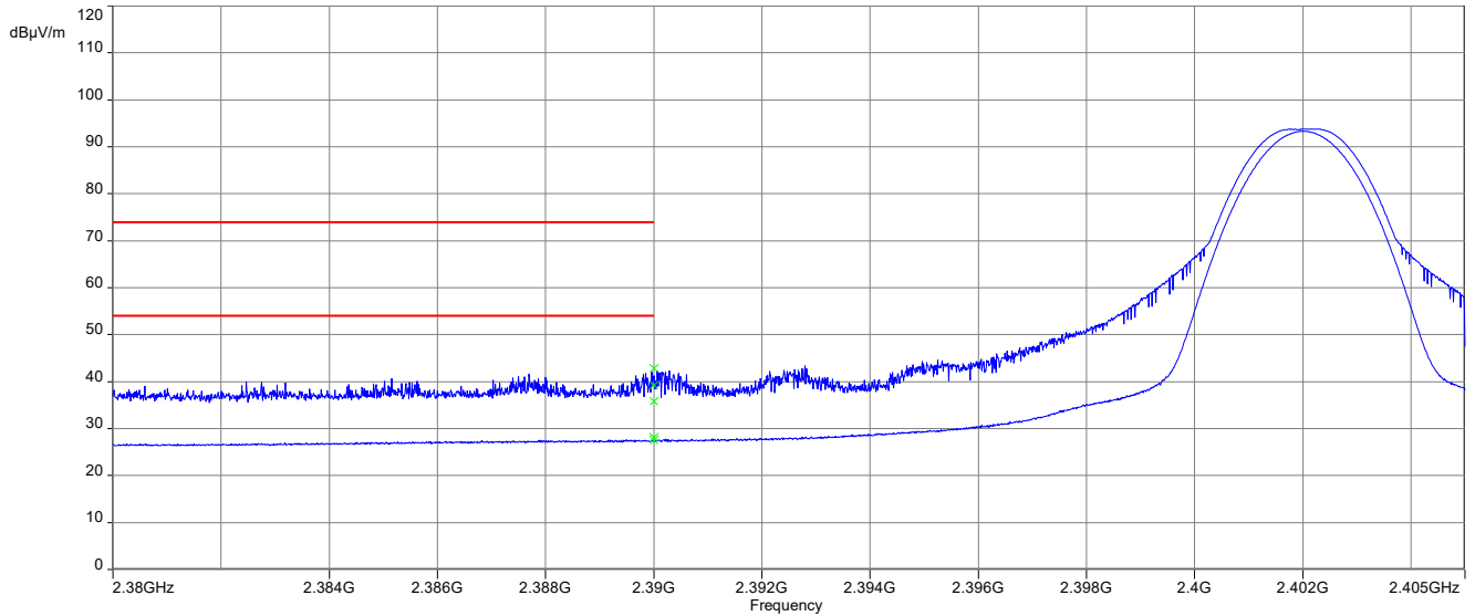
Plot 5: Lower restricted band, 1 Msps, Horizontal plane
