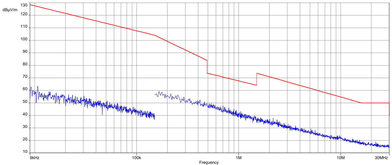
Plot 12: 9 kHz to 30 MHz, 2478 MHz, transmit mode, 2 Msps, Horizontal Plane
