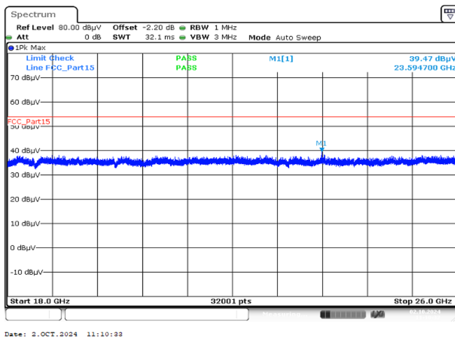
Plot 4: 18 GHz to 26 GHz, TX mode, vertical & horizontal polarization, 1 Msps, valid for all channels and both planes
