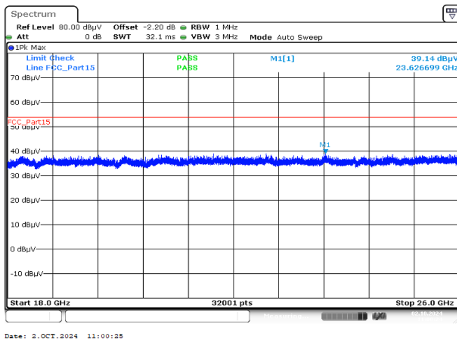
Plot 4: 18 GHz to 26 GHz, TX mode, vertical & horizontal polarization, MSK, valid for all channels and both planes
