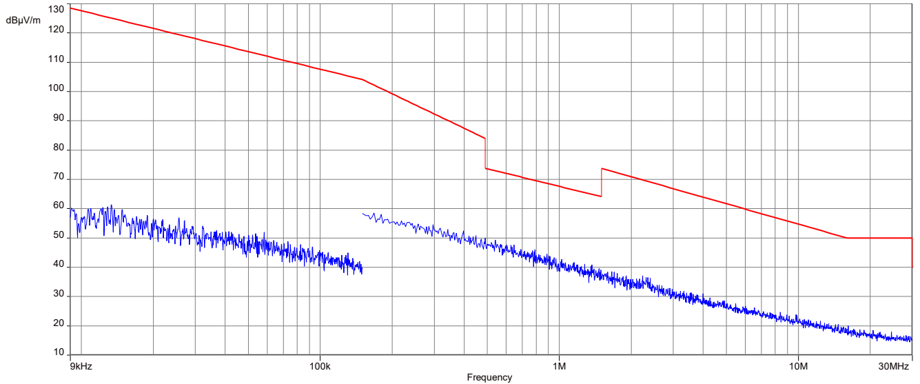
Plot 5: 9 kHz to 30 MHz, 2440 MHz, transmit mode, Horizontal Plane
