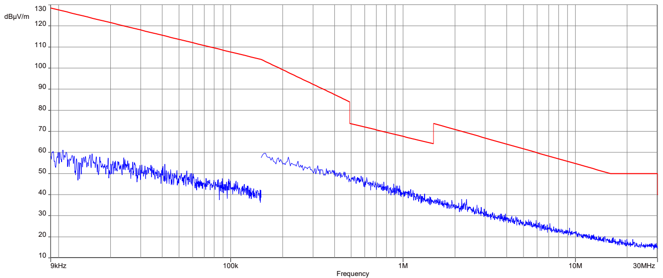
Plot 6: 9 kHz to 30 MHz, 2480 MHz, transmit mode, Horizontal Plane
