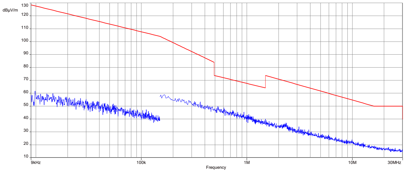
Plot 4: 9 kHz to 30 MHz, 2402 MHz, transmit mode, Horizontal Plane
