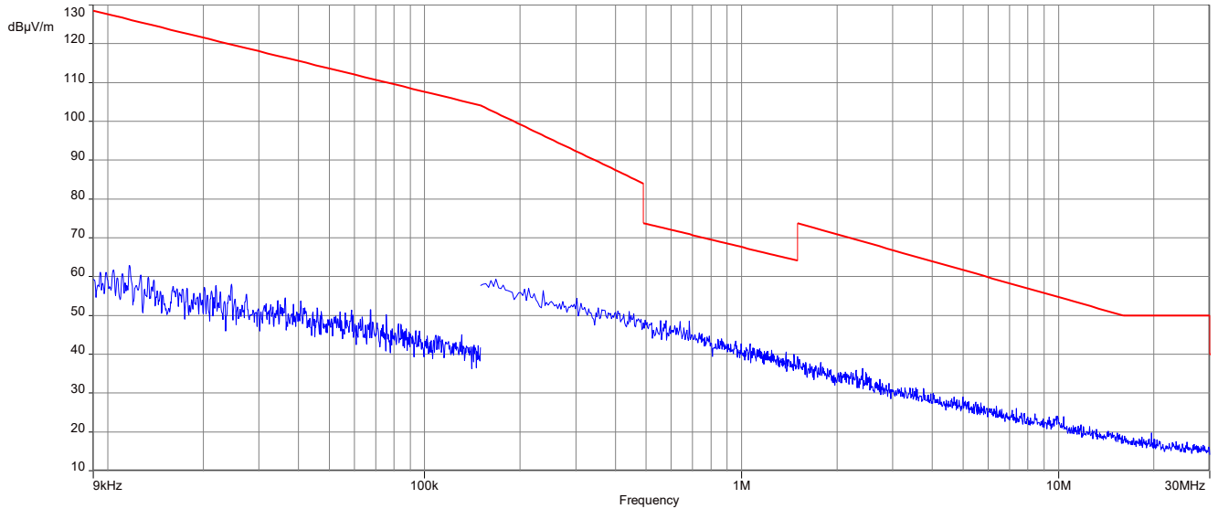
Plot 1: 9 kHz to 30 MHz, 2402 MHz, transmit mode, Vertical Plane
