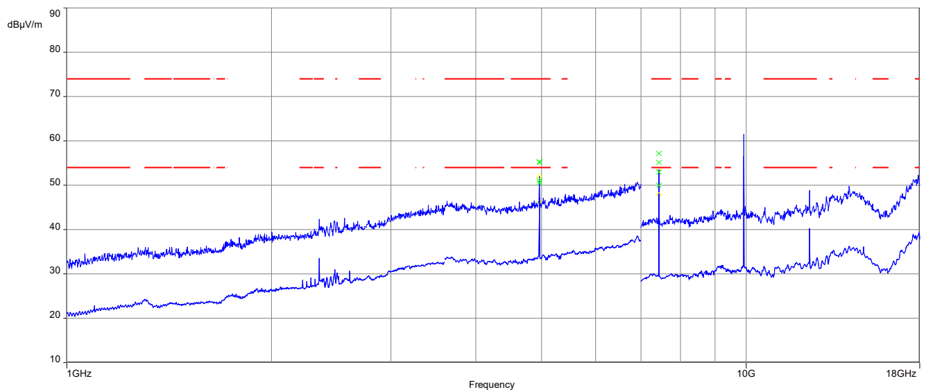
Plot 6: 1 GHz to 18 GHz, TX mode, 2480 MHz, vertical & horizontal polarization, Horizontal Plane
