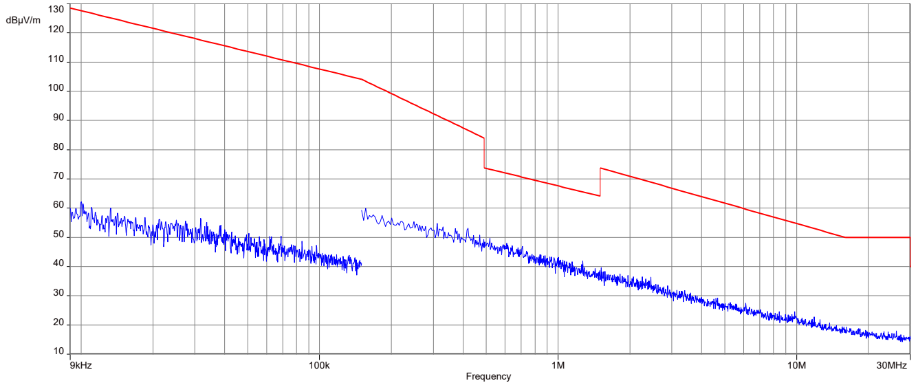
Plot 3: 9 kHz to 30 MHz, 2480 MHz, transmit mode, Vertical Plane
