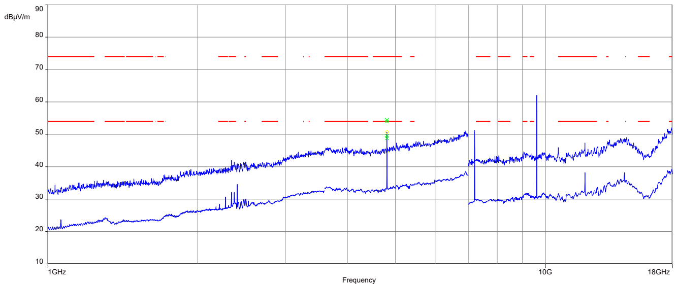
Plot 4: 1 GHz to 18 GHz, TX mode, 2402 MHz, vertical & horizontal polarization, Horizontal Plane
