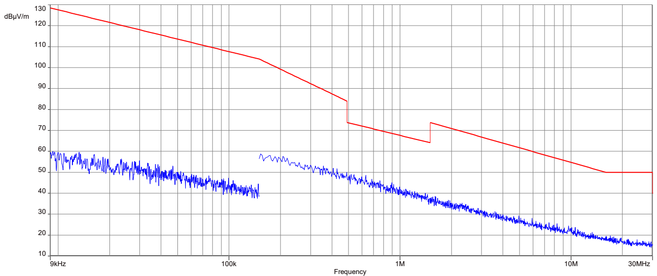
Plot 2: 9 kHz to 30 MHz, 2440 MHz, transmit mode, Vertical Plane
