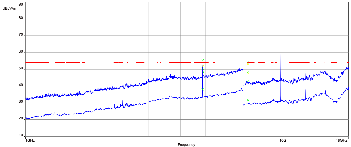
Plot 5: 1 GHz to 18 GHz, TX mode, 2440 MHz, vertical & horizontal polarization, Horizontal Plane
