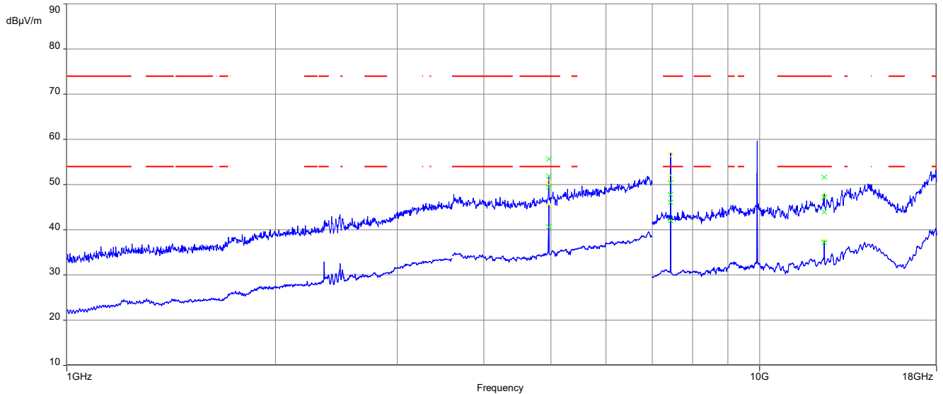
Plot 3: 1 GHz to 18 GHz, TX mode, 2480 MHz, vertical & horizontal polarization, Vertical Plane
