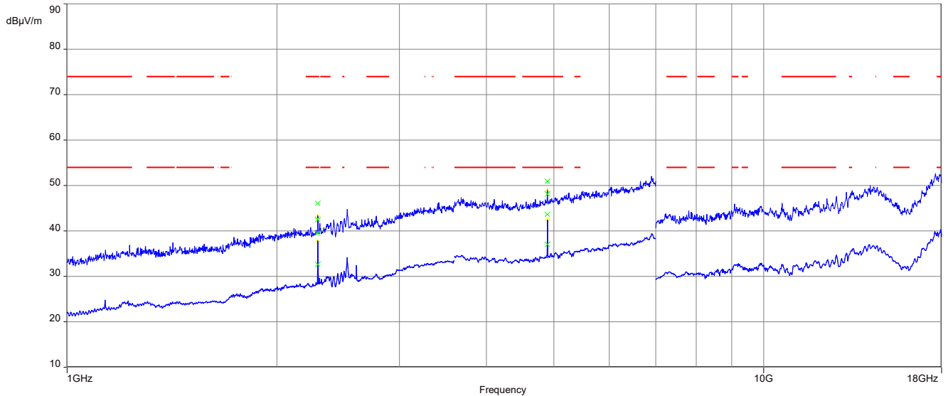
Plot 5: 1 GHz to 18 GHz, TX mode, 2447 MHz, vertical & horizontal polarization, Horizontal Plane
