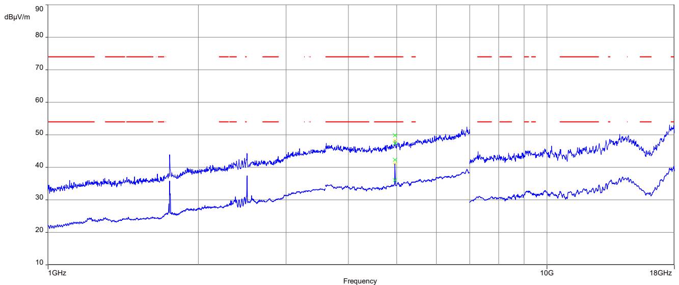
Plot 6: 1 GHz to 18 GHz, TX mode, 2479 MHz, vertical & horizontal polarization, Horizontal Plane
