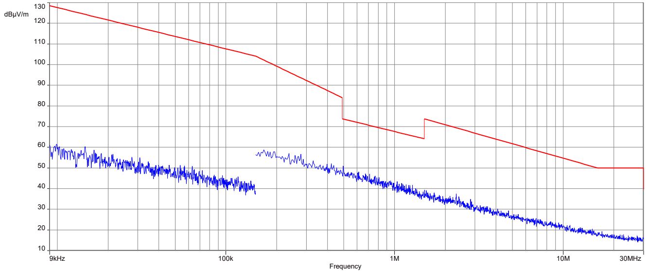
Plot 1: 9 kHz to 30 MHz, 2404 MHz, transmit mode, Vertical Plane
