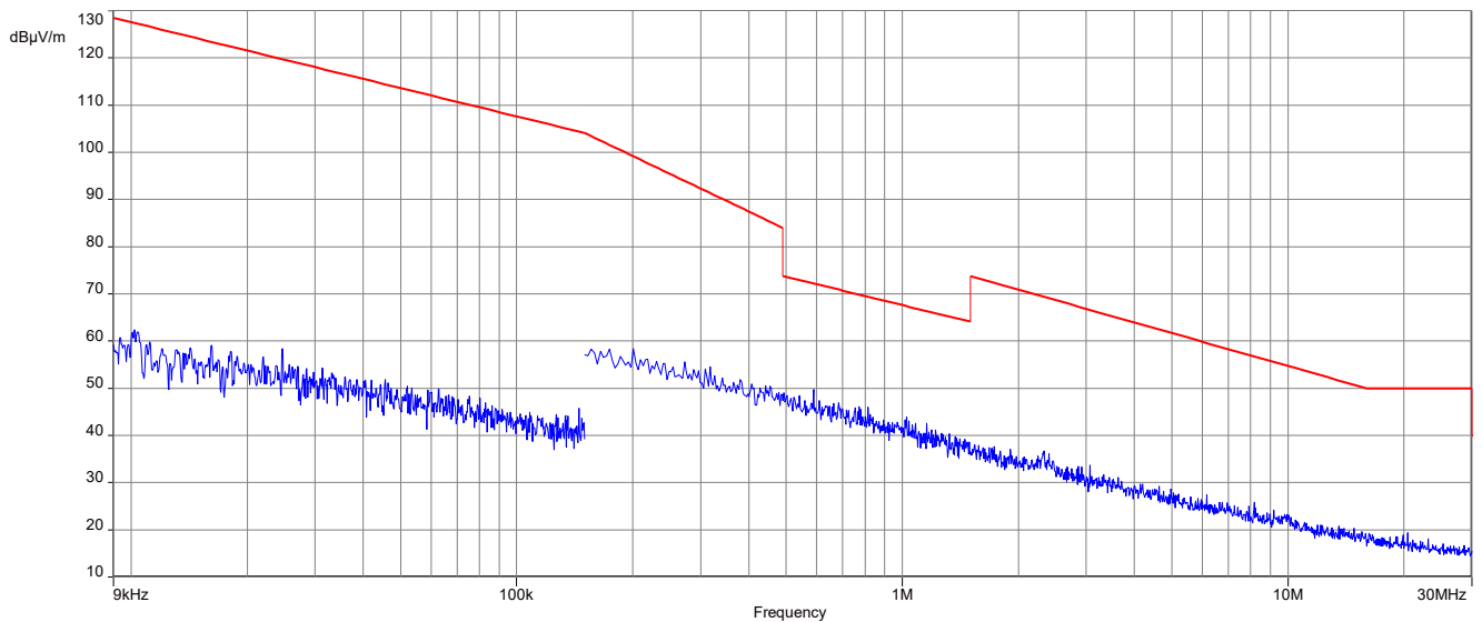
Plot 6: 9 kHz to 30 MHz, 2479 MHz, transmit mode, Horizontal Plane
