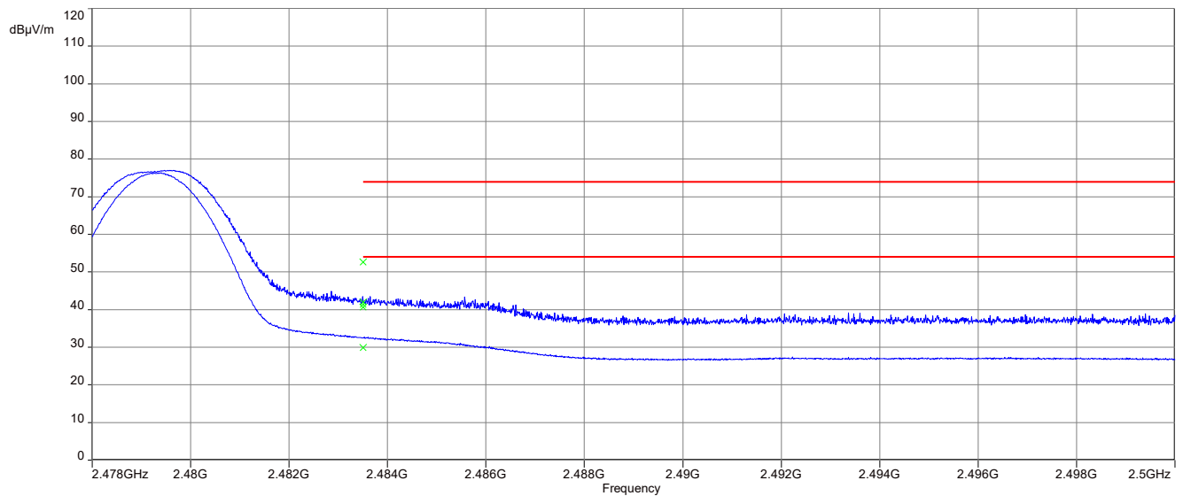
Plot 2: Upper restricted band, Vertical Plane
