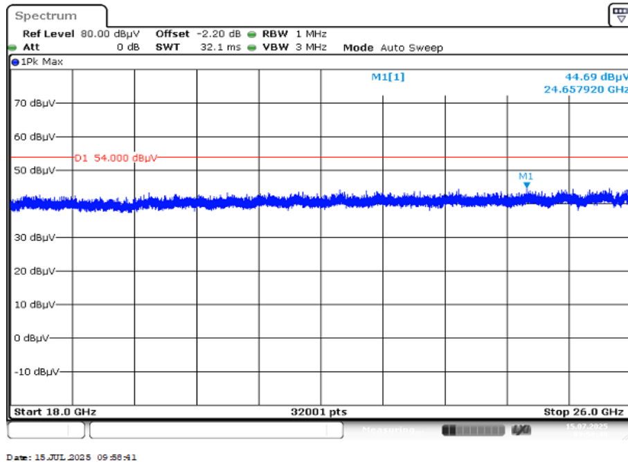
Plot 7: 18 GHz to 26 GHz, TX mode, vertical & horizontal polarization, valid for all channels
