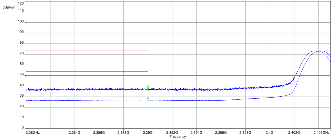
Plot 1: Lower restricted band, Vertical Plane
