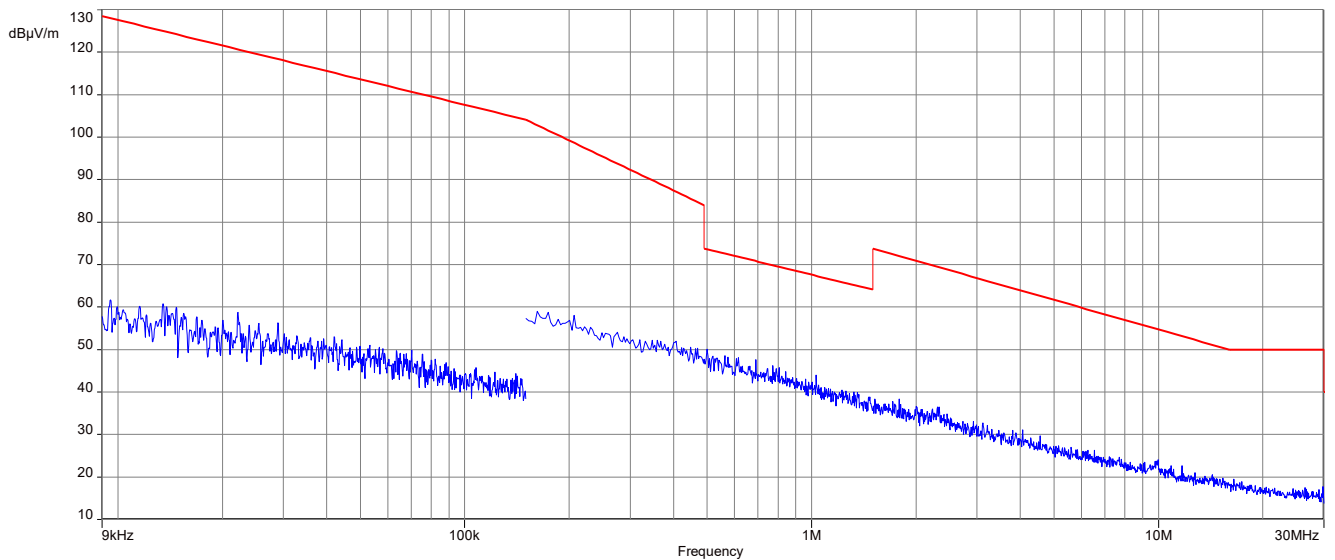
Plot 4: 9 kHz to 30 MHz, 2404 MHz, transmit mode, Horizontal Plane
