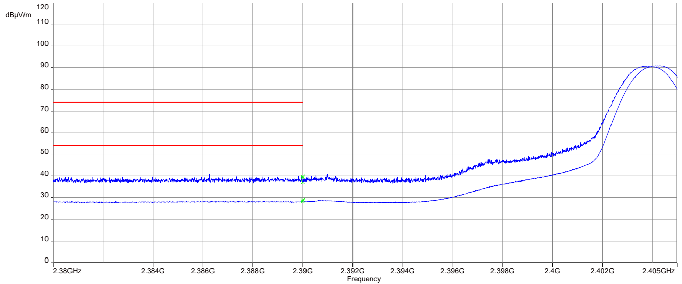
Plot 3: Lower restricted band, Horizontal Plane
