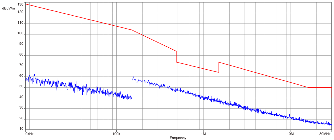
Plot 2: 9 kHz to 30 MHz, 2447 MHz, transmit mode, Vertical Plane
