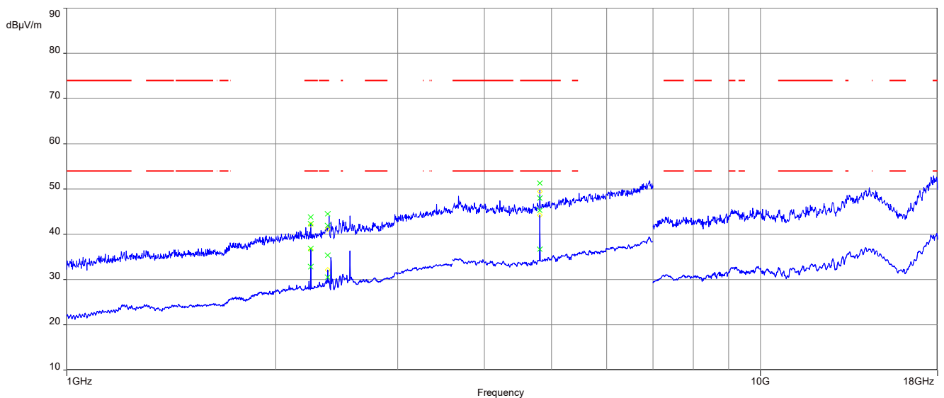
Plot 4: 1 GHz to 18 GHz, TX mode, 2404 MHz, vertical & horizontal polarization, Horizontal Plane
