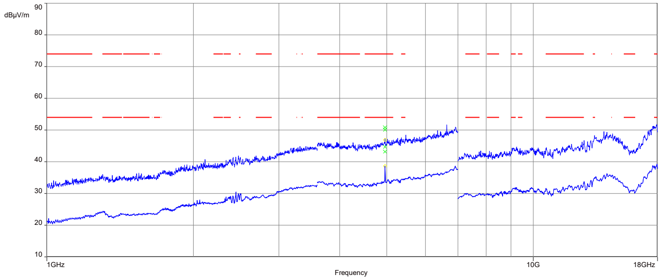
Plot 3: 1 GHz to 18 GHz, TX mode, 2479 MHz, vertical & horizontal polarization, Vertical Plane
