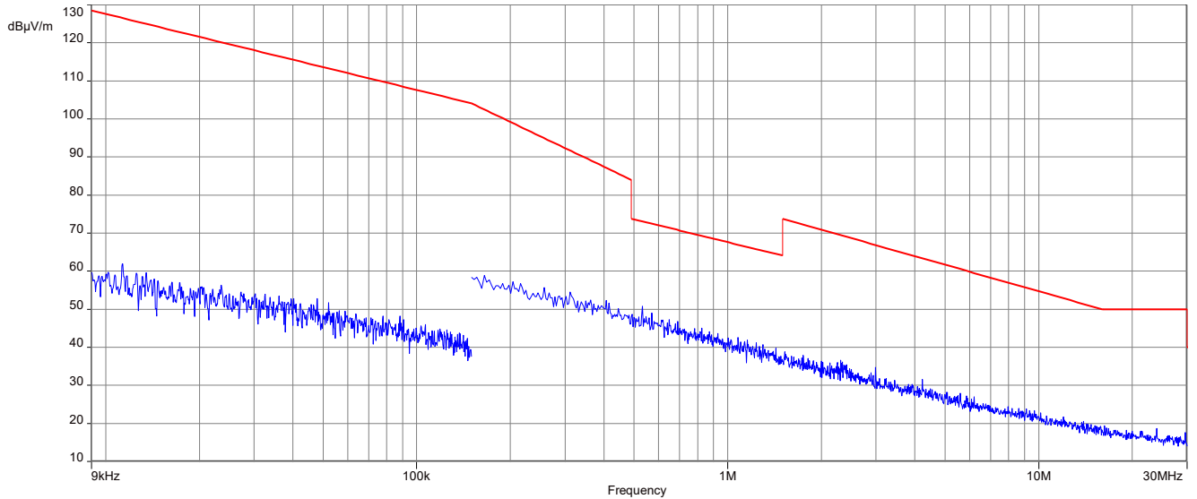
Plot 3: 9 kHz to 30 MHz, 2479 MHz, transmit mode, Vertical Plane
