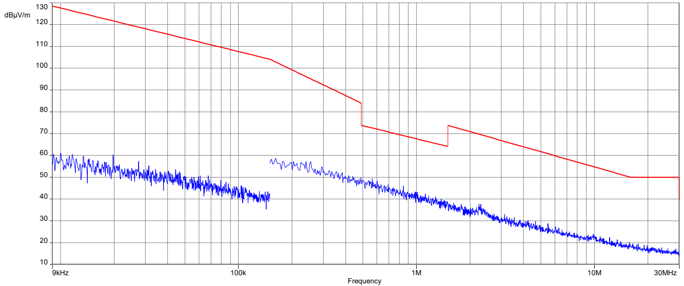
Plot 5: 9 kHz to 30 MHz, 2447 MHz, transmit mode, Horizontal Plane
