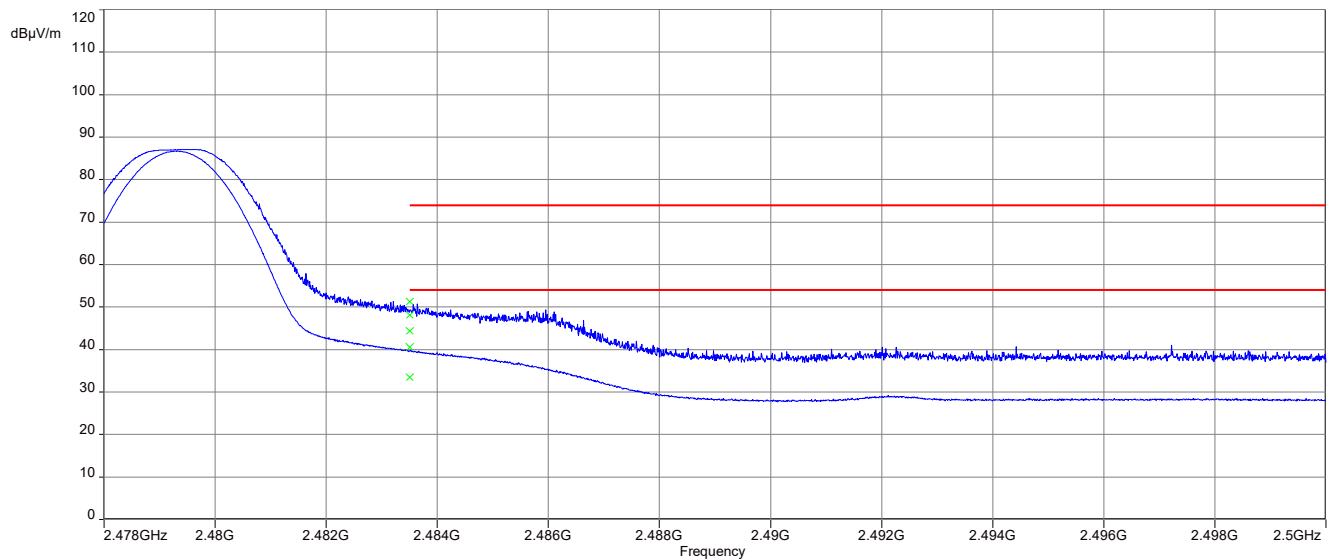
Plot 4: Upper restricted band, Horizontal Plane
