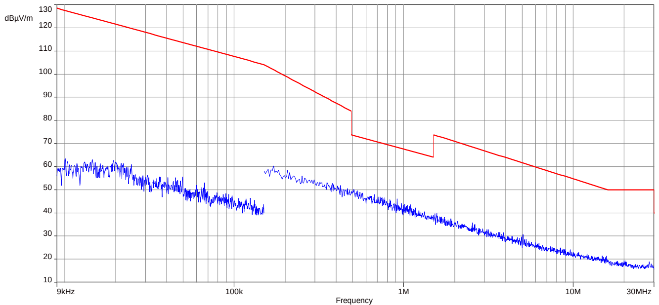
Plot 2: 9 kHz to 30 MHz, 2447 MHz, transmit mode
