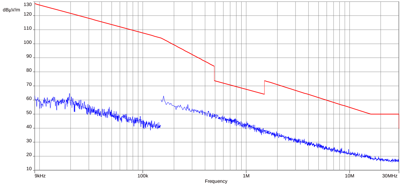
Plot 1: 9 kHz to 30 MHz, 2404 MHz, transmit mode
