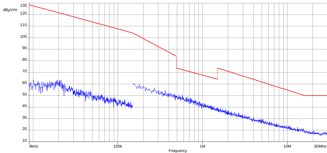
Plot 3: 9 kHz to 30 MHz, 2479 MHz, transmit mode
