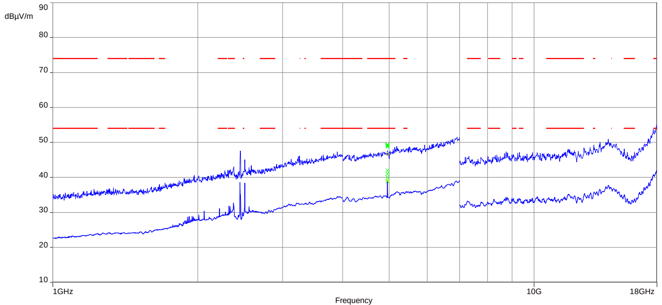
Plot 3 1 GHz to 18 GHz, TX mode, 2479 MHz, vertical & horizontal polarization
