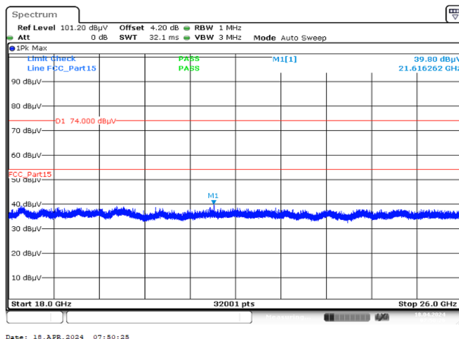
Plot 4: 18 GHz to 26 GHz, TX mode, vertical & horizontal polarization, MSK, valid for all channels
