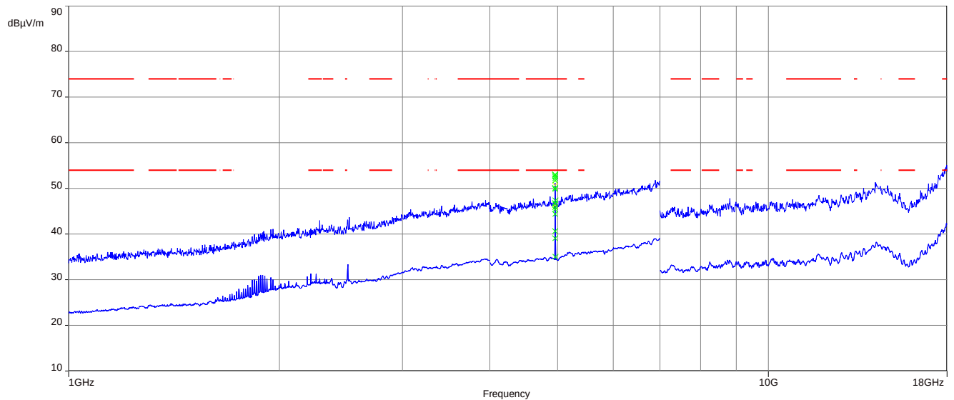
Plot 3: 1 GHz to 18 GHz, TX mode, 2479.3 MHz, vertical & horizontal polarization, MSK
