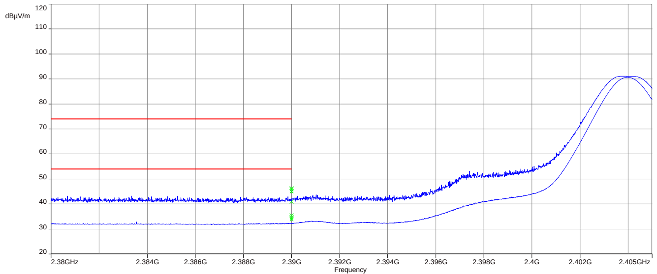
Plot 1: Lower restricted band, MSK
