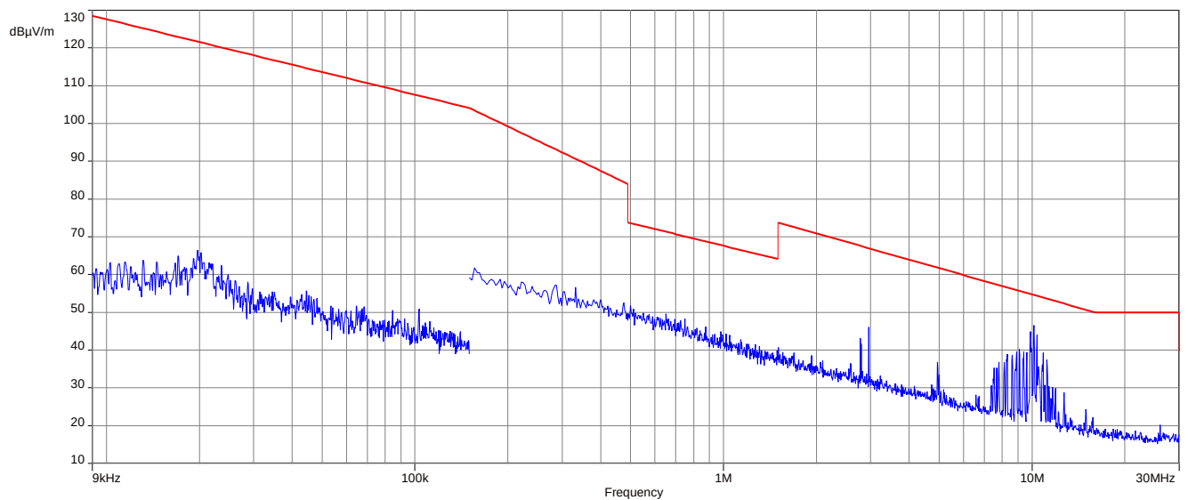
Plot 2: 9 kHz to 30 MHz, 2447 MHz, transmit mode, MSK
