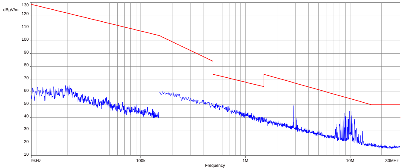
Plot 1: 9 kHz to 30 MHz, 2404 MHz, transmit mode, MSK
