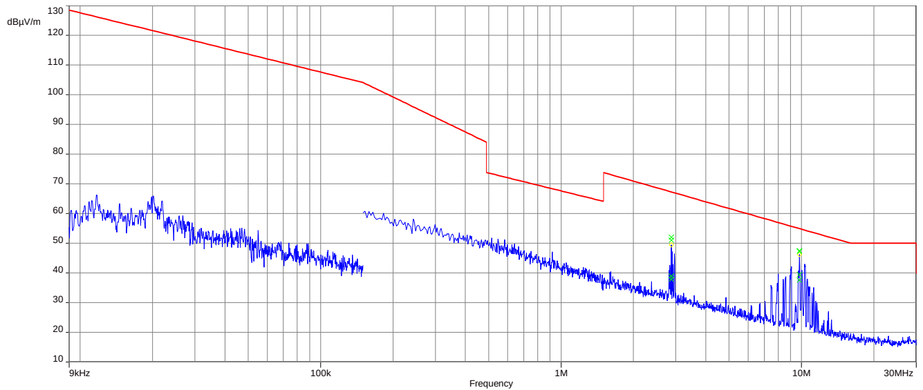
Plot 3: 9 kHz to 30 MHz, 2479.3 MHz, transmit mode, MSK
