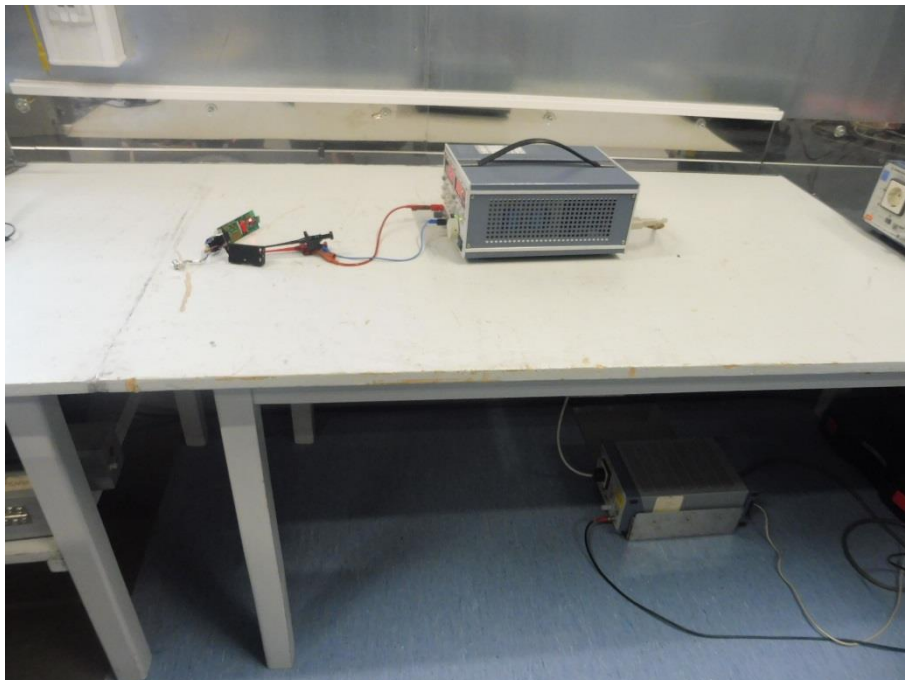
Photo 8: AC conducted test setup
