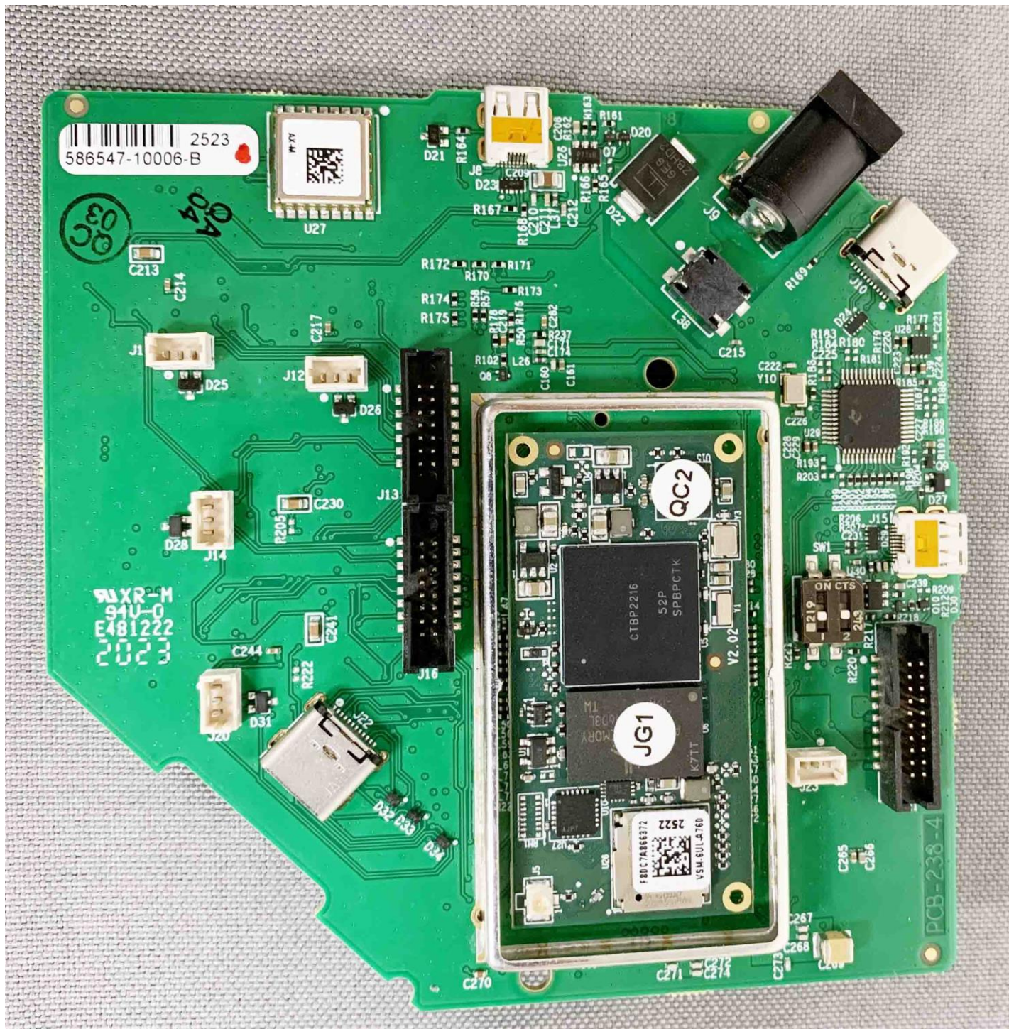
With Daughter Board, Shield removed
