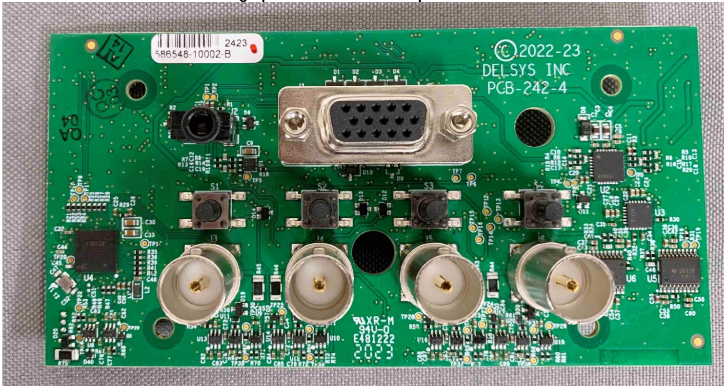
Photograph of PC Board 2: Foil Side
