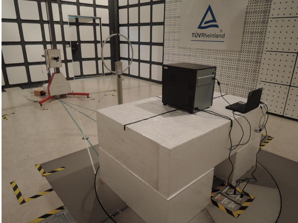
Photograph 2: Set-up for Fundamental Emissions (Back View)
