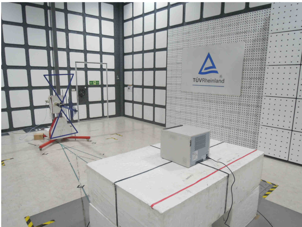
Photograph 3: Set-up for Radiated Emissions (Back View)
