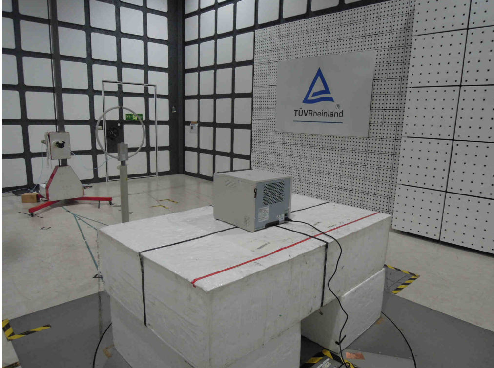
Photograph 2: Set-up for Radiated Emissions (Back View)
