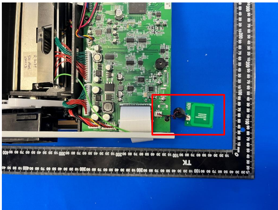
NFC Antenna Location
