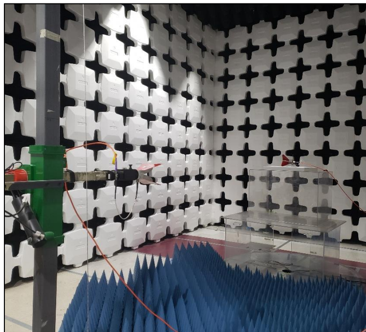
Photograph 4. Radiated Spurious Emissions, Substitution Method Above 1GHz, Test Setup
