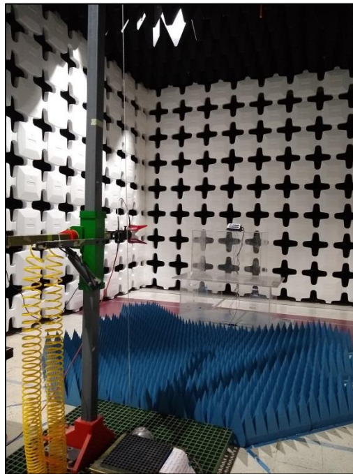
Photograph 2. Radiated Emissions, 1 GHz – 18 GHz, Test Setup
