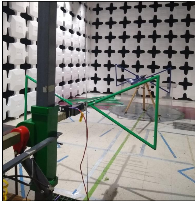
Photograph 3. Radiated Spurious Emissions, Substitution Method Below 1GHz, Test Setup
