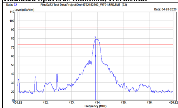
TX, Fundamental 433.92MHz Tx (Ch 1) Radiated Spurious Emission, Horizontal
