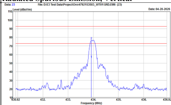
TX, Fundamental 433.92MHz Tx (Ch 1) Radiated Spurious Emission, Vertical
