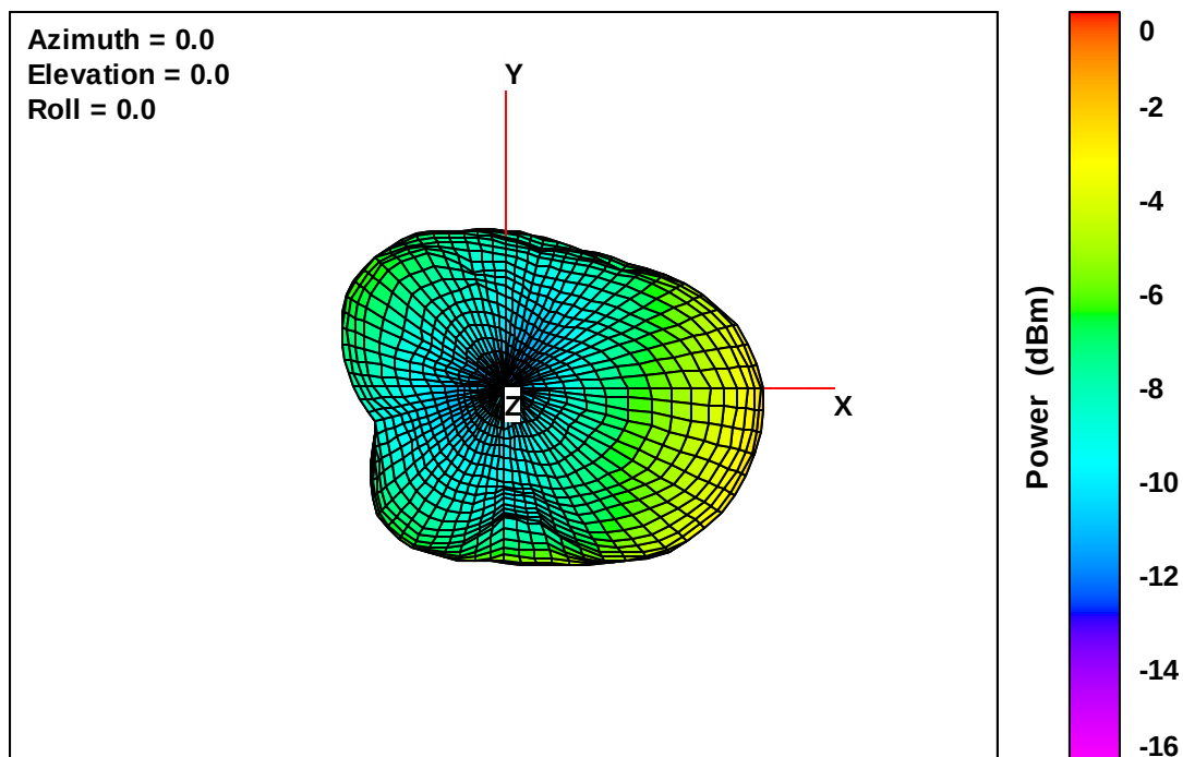
Wearable Defibrillator Free-Space Total EIRP, Top View, 756 MHz
