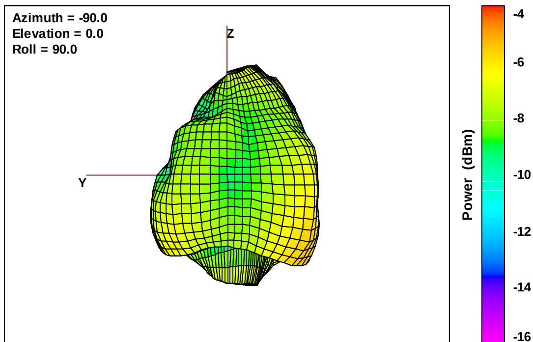
Wearable Defibrillator Free-Space Total EIRP, Back Face View, 869 MHz
