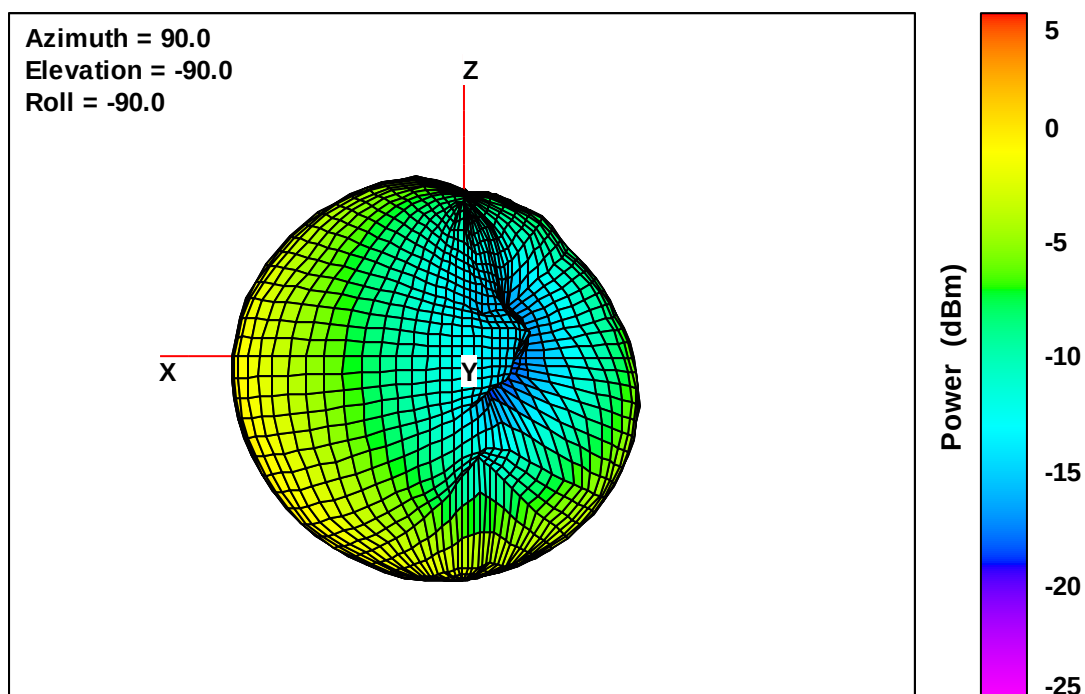
Wearable Defibrillator Free-Space Total EIRP, Right Side View, 713 MHz
