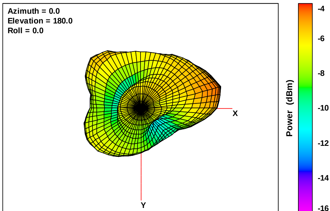
Wearable Defibrillator Free-Space Total EIRP, Bottom View, 869 MHz
