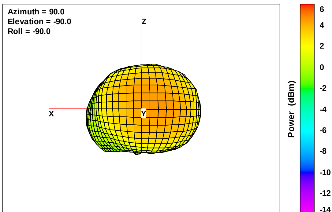
Wearable Defibrillator Free-Space Total EIRP, Right Side View, 1990 MHz
