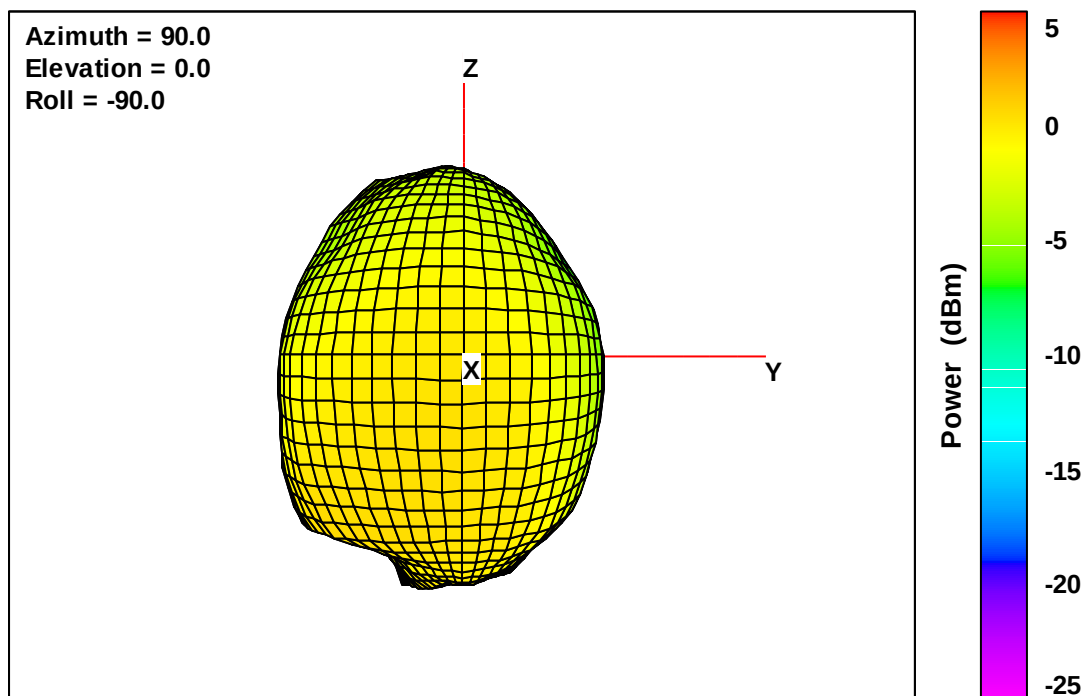
Wearable Defibrillator Free-Space Total EIRP, Front Face View, 713 MHz
