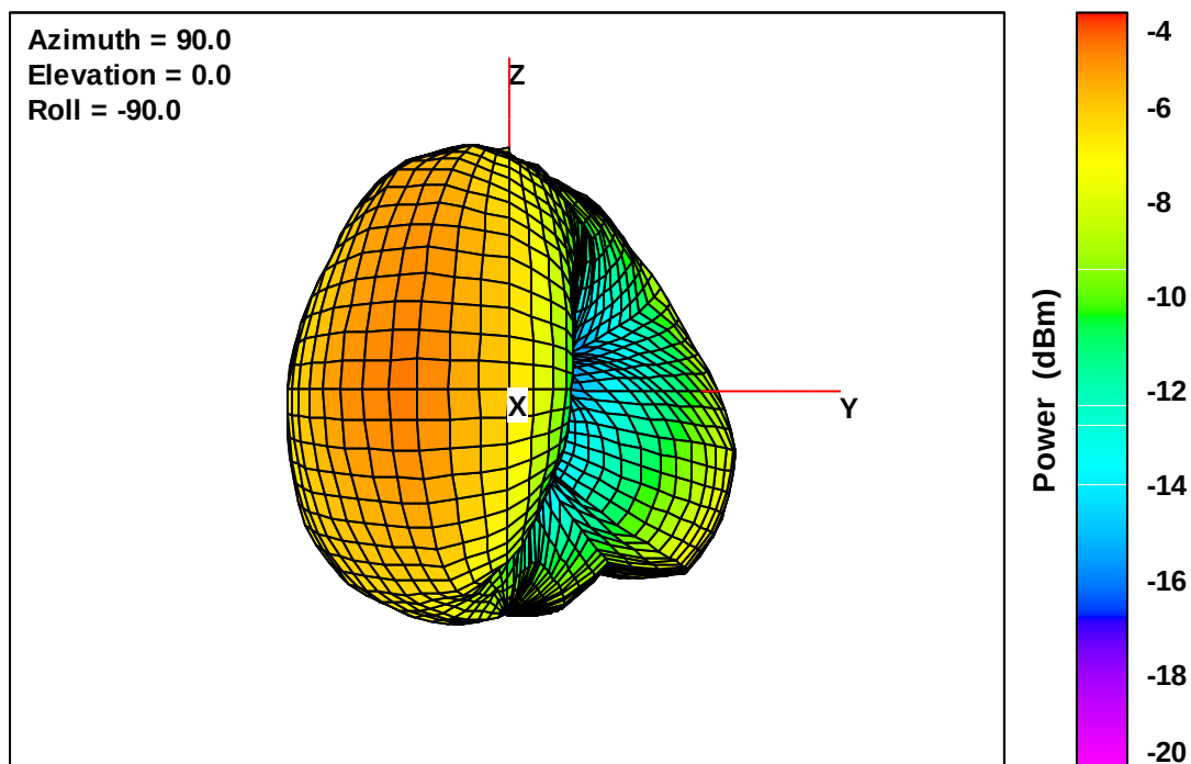
Wearable Defibrillator Free-Space Total EIRP, Front Face View, 915 MHz
