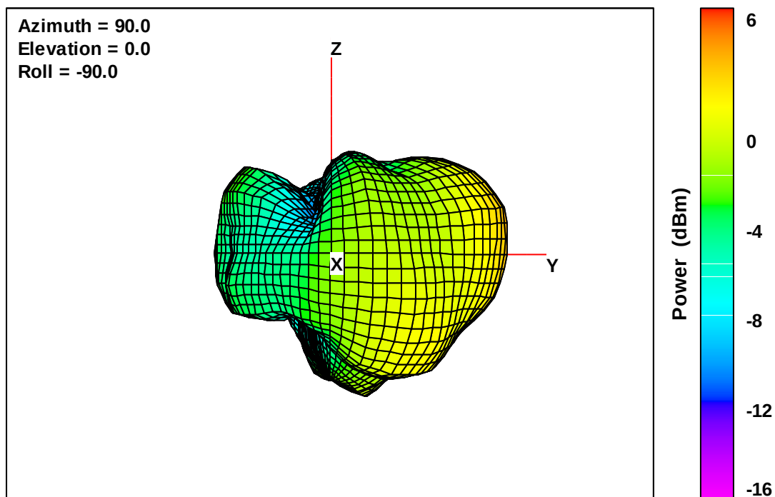
Wearable Defibrillator Free-Space Total EIRP, Front Face View, 1910 MHz
