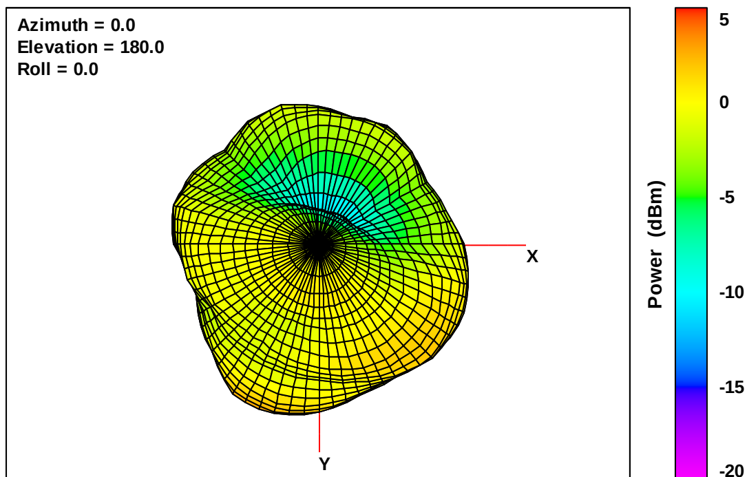
Wearable Defibrillator Free-Space Total EIRP, Bottom View, 1850 MHz
