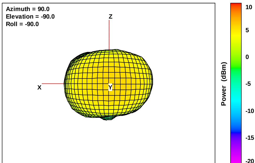
Wearable Defibrillator Free-Space Total EIRP, Right Side View, 2155 MHz
