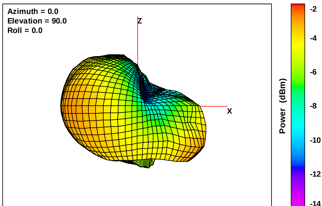
Wearable Defibrillator Free-Space Total EIRP, Left Side View, 787 MHz
