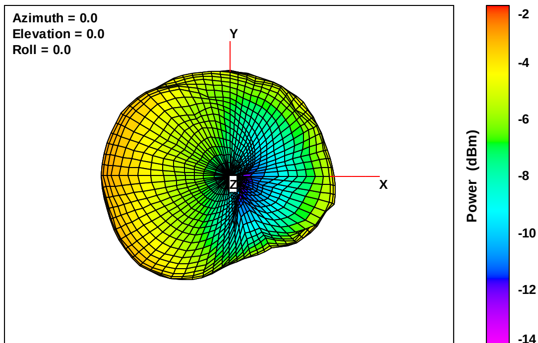
Wearable Defibrillator Free-Space Total EIRP, Top View, 787 MHz
