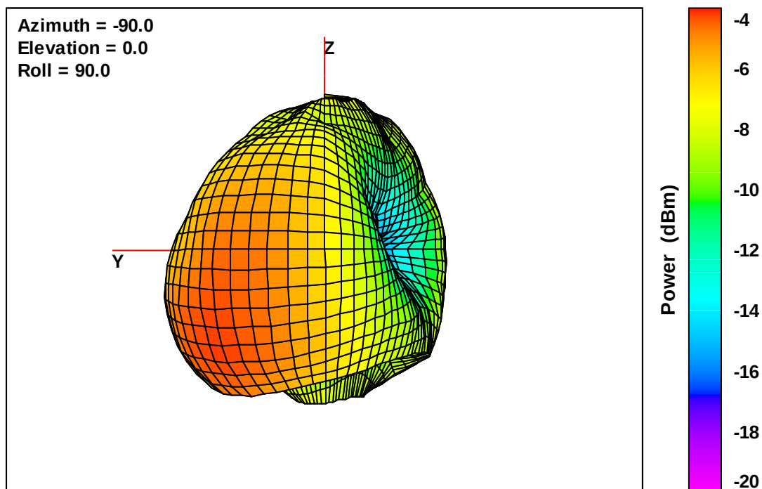
Wearable Defibrillator Free-Space Total EIRP, Back Face View, 915 MHz
