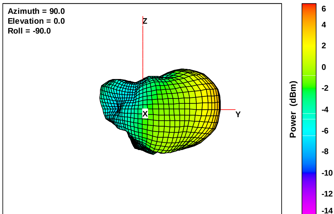
Wearable Defibrillator Free-Space Total EIRP, Front Face View, 1990 MHz
