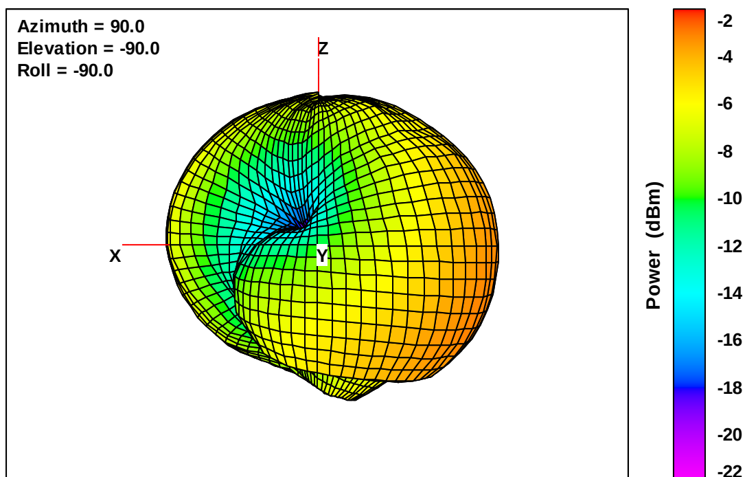
Wearable Defibrillator Free-Space Total EIRP, Right Side View, 960 MHz
