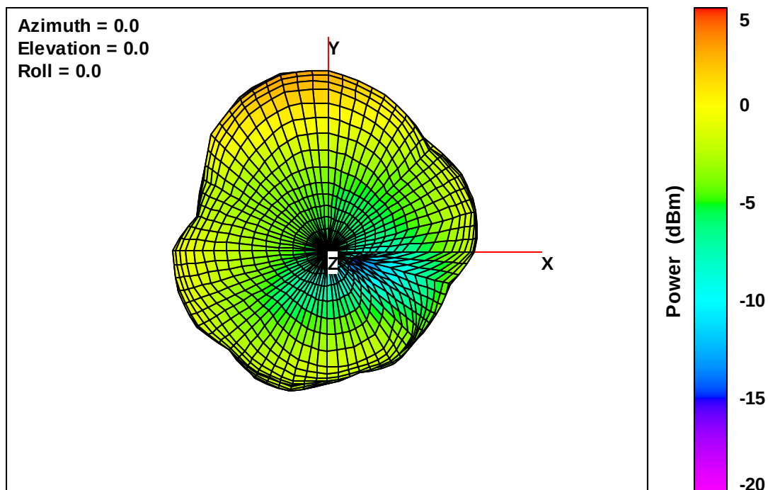
Wearable Defibrillator Free-Space Total EIRP, Top View, 1850 MHz
