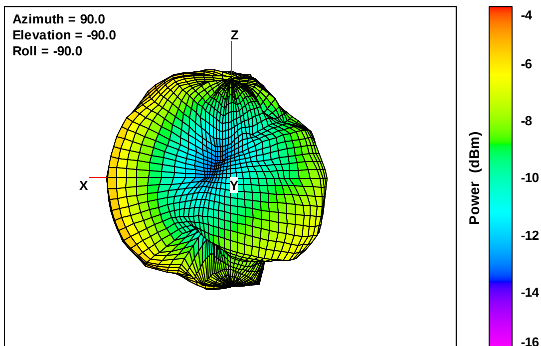
Wearable Defibrillator Free-Space Total EIRP, Right Side View, 869 MHz
