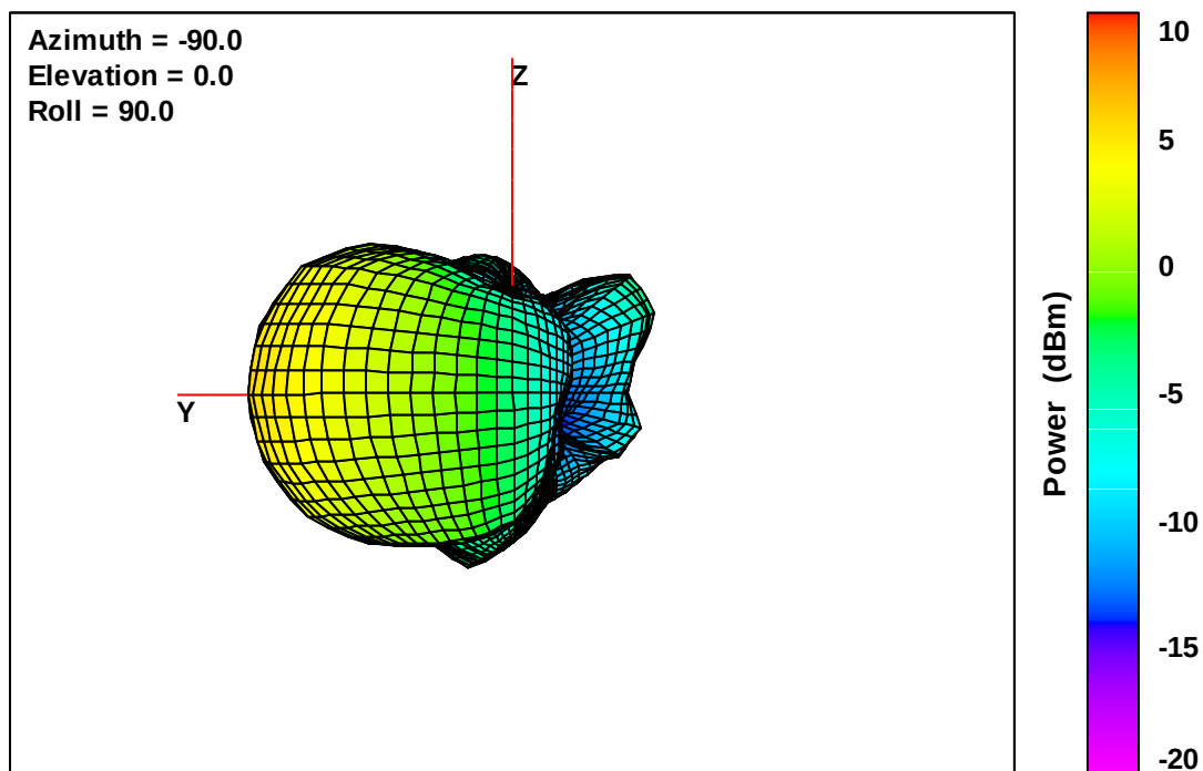
Wearable Defibrillator Free-Space Total EIRP, Back Face View, 2110 MHz
