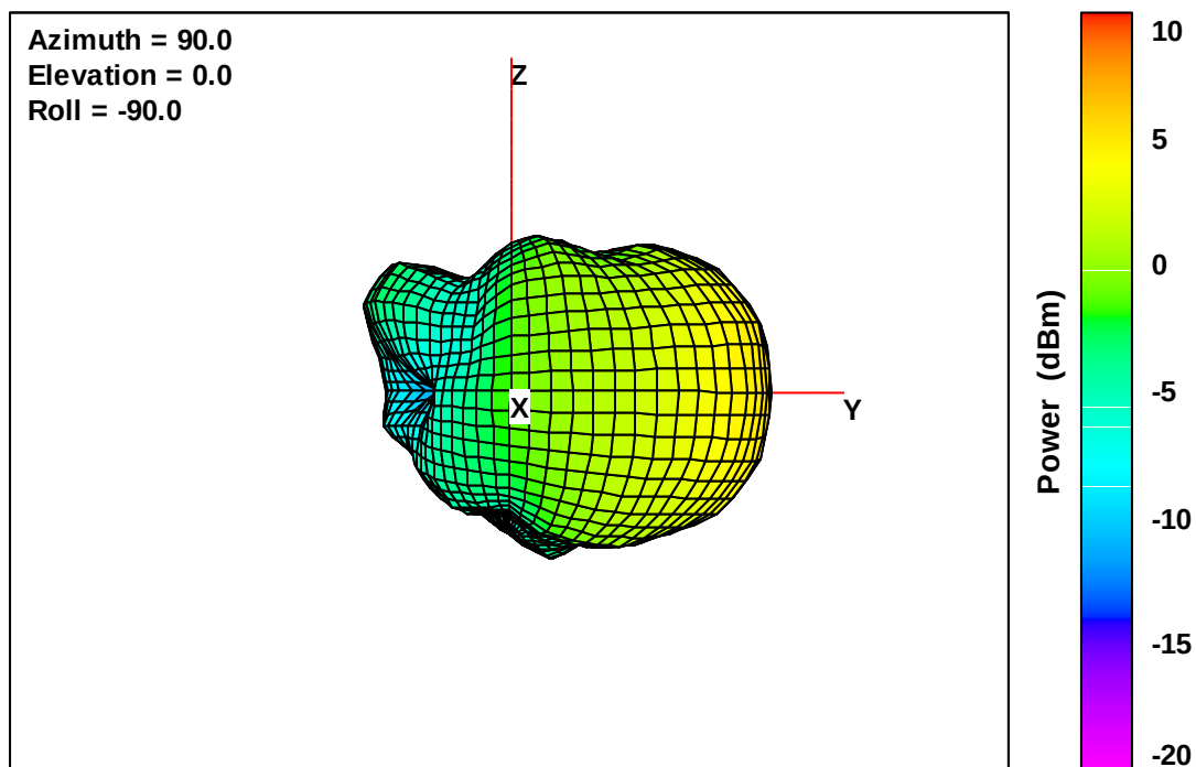
Wearable Defibrillator Free-Space Total EIRP, Front Face View, 2155 MHz
