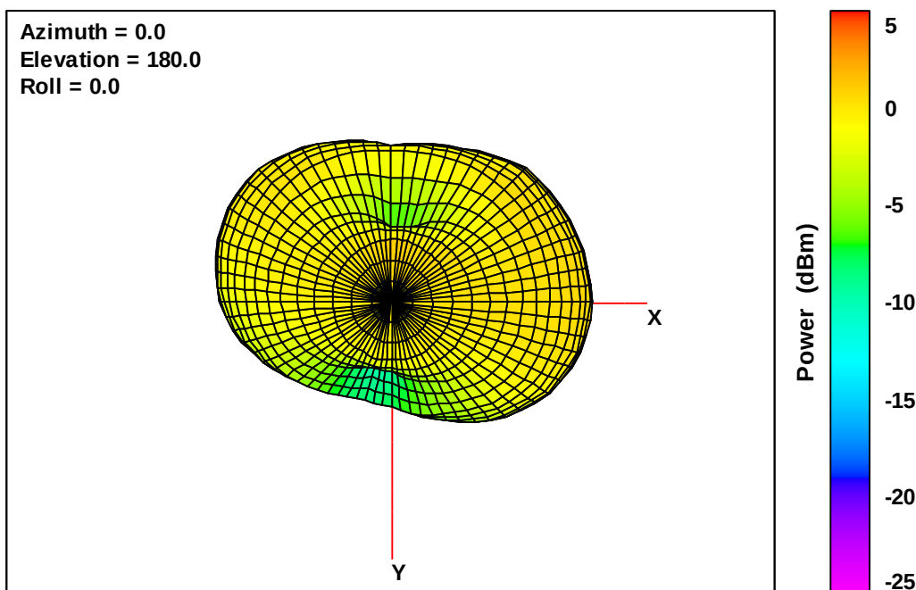
Wearable Defibrillator Free-Space Total EIRP, Bottom View, 699 MHz
