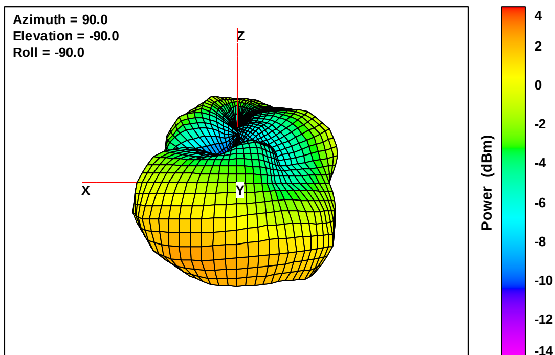
Wearable Defibrillator Free-Space Total EIRP, Right Side View, 1755 MHz
