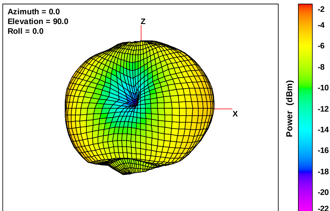
Wearable Defibrillator Free-Space Total EIRP, Left Side View, 960 MHz
