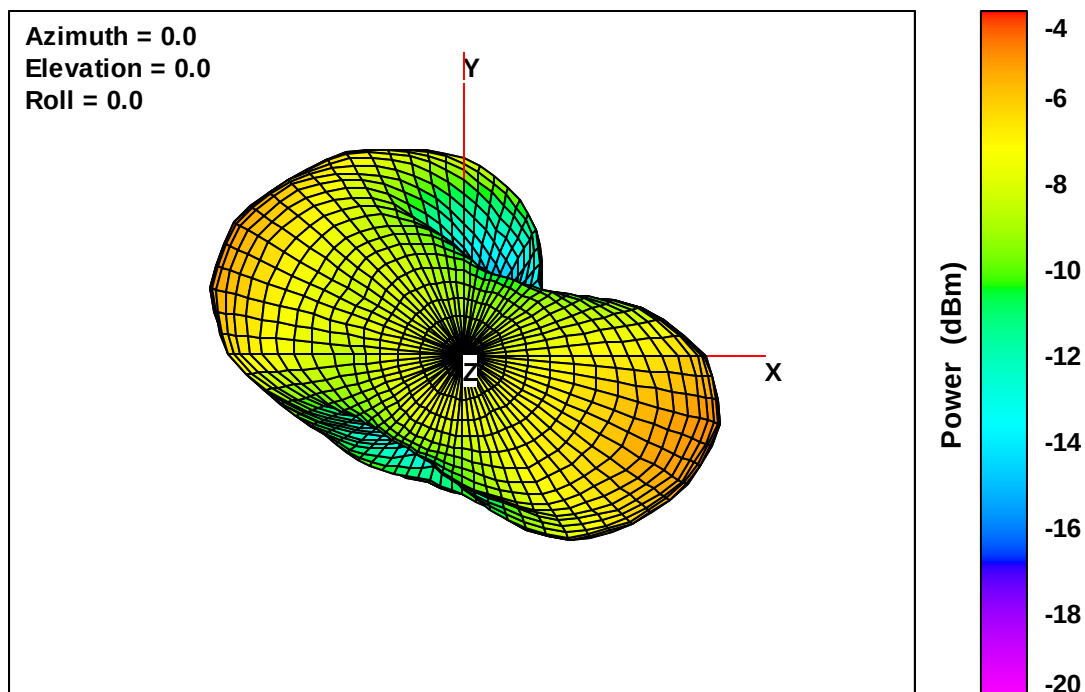
Wearable Defibrillator Free-Space Total EIRP, Top View, 915 MHz
