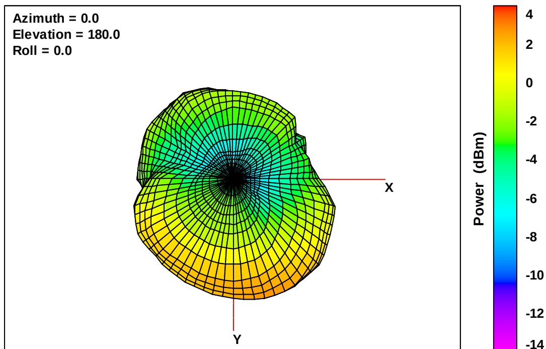
Wearable Defibrillator Free-Space Total EIRP, Bottom View, 1755 MHz
