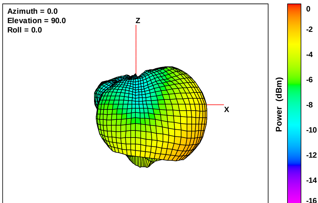
Wearable Defibrillator Free-Space Total EIRP, Left Side View, 756 MHz
