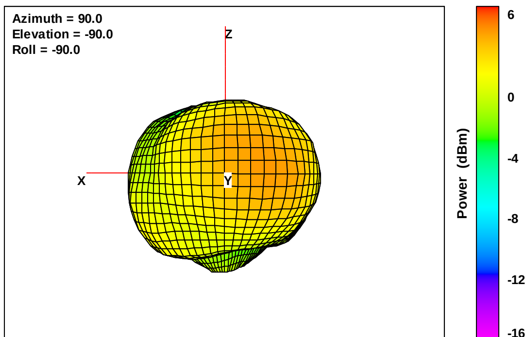
Wearable Defibrillator Free-Space Total EIRP, Right Side View, 1910 MHz
