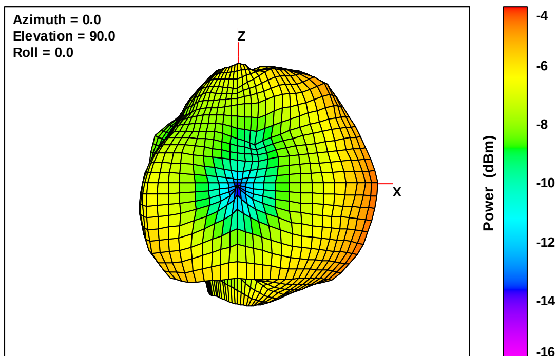
Wearable Defibrillator Free-Space Total EIRP, Left Side View, 869 MHz
