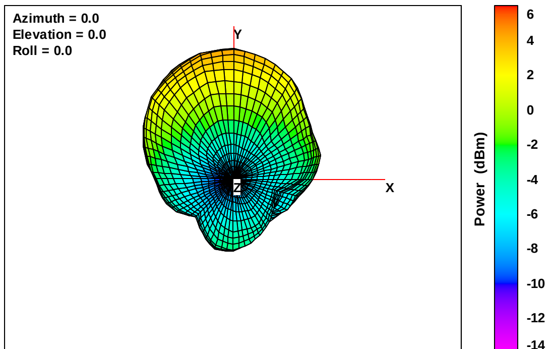
Wearable Defibrillator Free-Space Total EIRP, Top View, 1990 MHz
