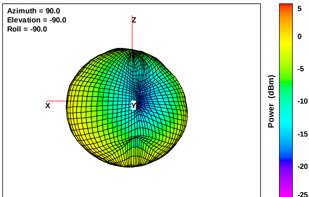
Wearable Defibrillator Free-Space Total EIRP, Right Side View, 699 MHz
