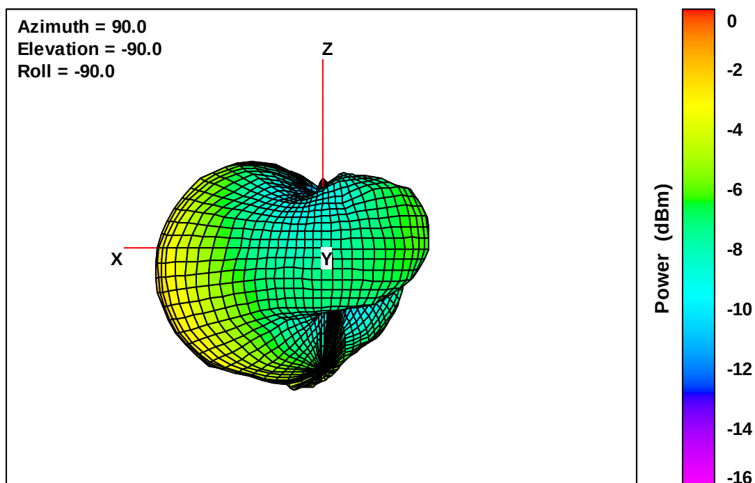
Wearable Defibrillator Free-Space Total EIRP, Right Side View, 756 MHz
