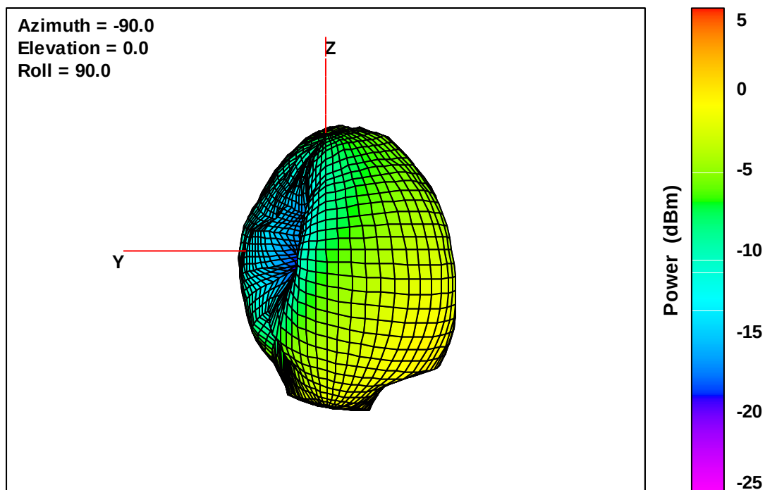
Wearable Defibrillator Free-Space Total EIRP, Back Face View, 713 MHz
