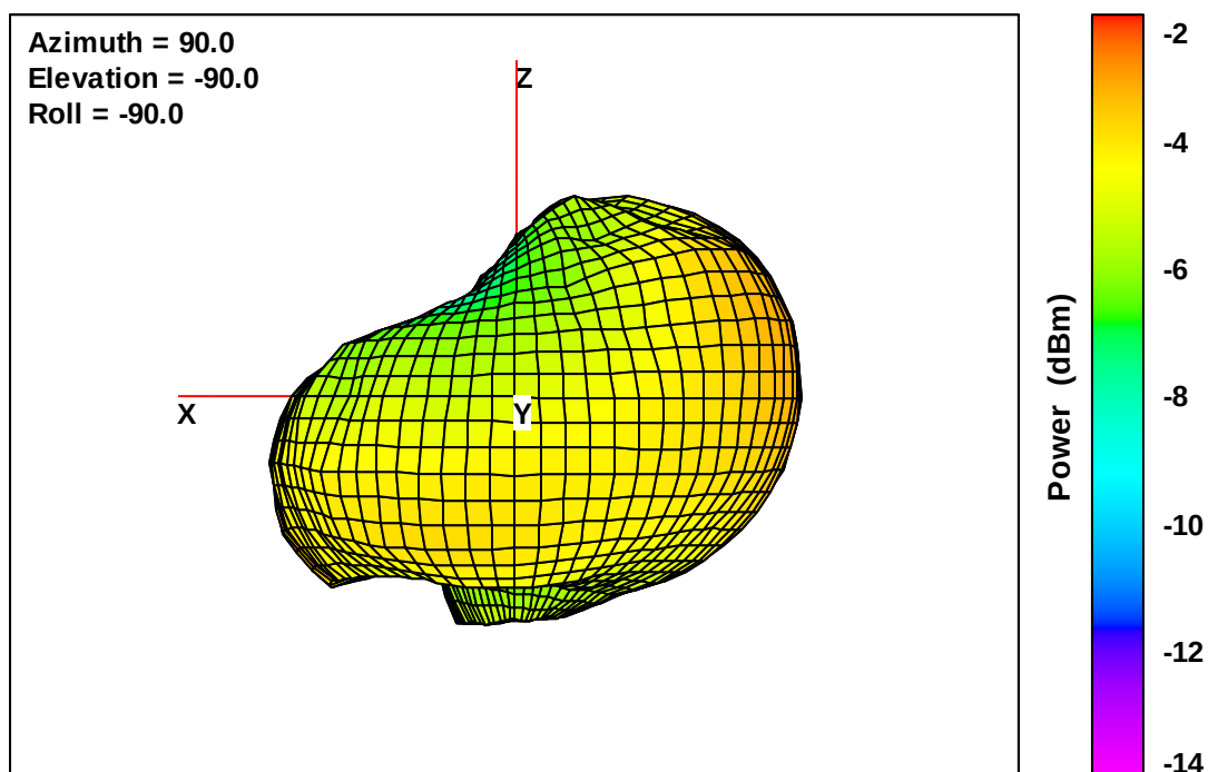
Wearable Defibrillator Free-Space Total EIRP, Right Side View, 787 MHz
