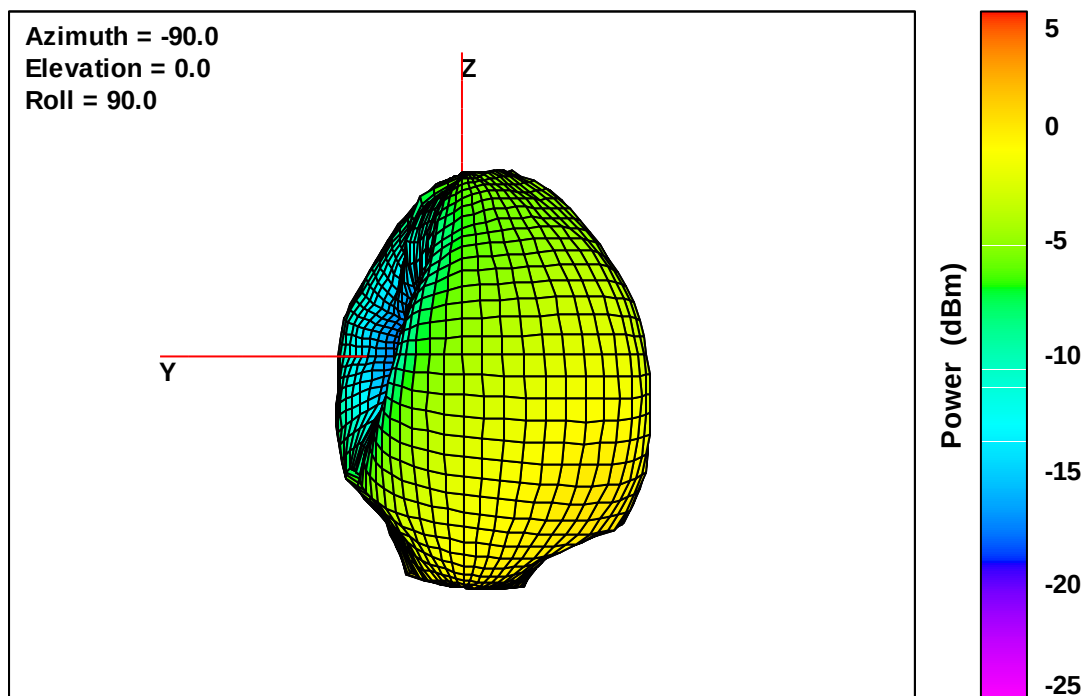
Wearable Defibrillator Free-Space Total EIRP, Back Face View, 699 MHz
