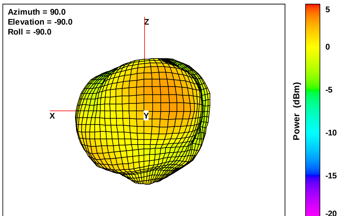
Wearable Defibrillator Free-Space Total EIRP, Right Side View, 1850 MHz
