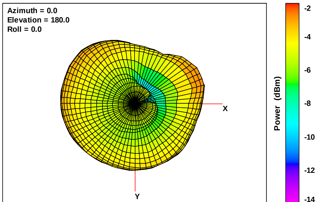
Wearable Defibrillator Free-Space Total EIRP, Bottom View, 787 MHz
