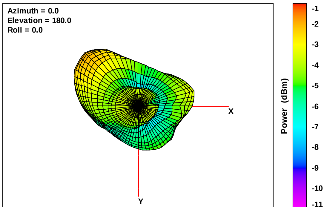
Wearable Defibrillator Free-Space Total EIRP, Bottom View, 824 MHz
