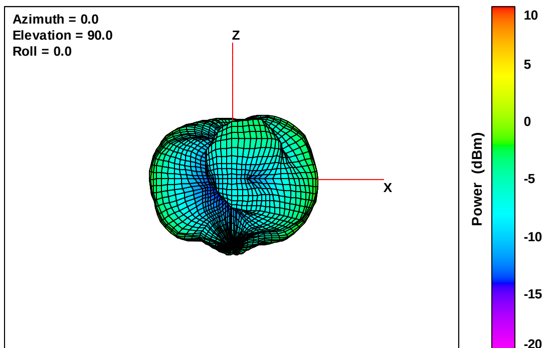
Wearable Defibrillator Free-Space Total EIRP, Left Side View, 2110 MHz
