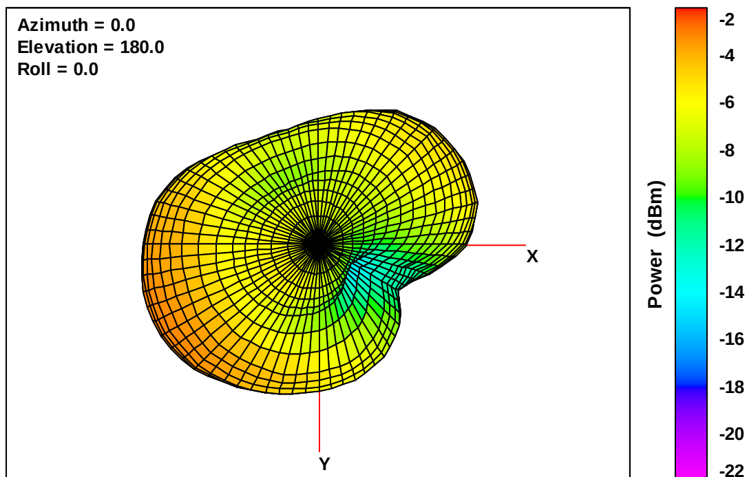
Wearable Defibrillator Free-Space Total EIRP, Bottom View, 960 MHz
