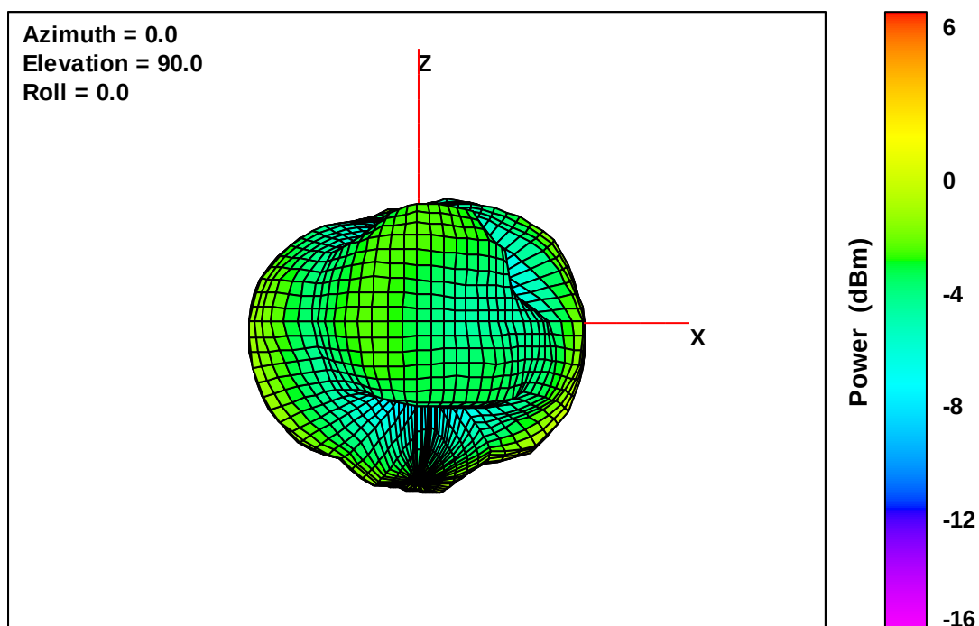
Wearable Defibrillator Free-Space Total EIRP, Left Side View, 1910 MHz
