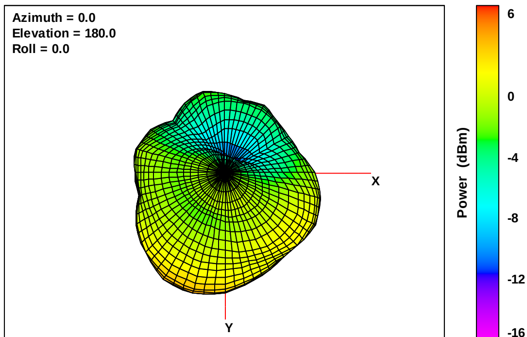
Wearable Defibrillator Free-Space Total EIRP, Bottom View, 1910 MHz
