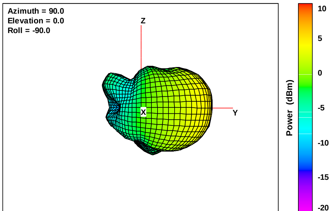
Wearable Defibrillator Free-Space Total EIRP, Front Face View, 2110 MHz
