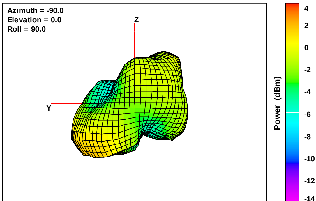
Wearable Defibrillator Free-Space Total EIRP, Back Face View, 1755 MHz
