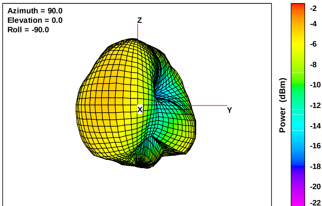
Wearable Defibrillator Free-Space Total EIRP, Front Face View, 960 MHz
