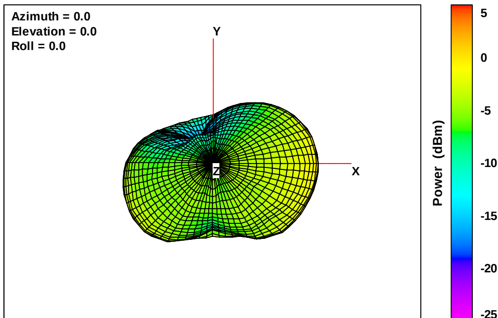
Wearable Defibrillator Free-Space Total EIRP, Top View, 699 MHz
