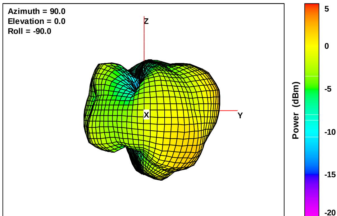
Wearable Defibrillator Free-Space Total EIRP, Front Face View, 1850 MHz
