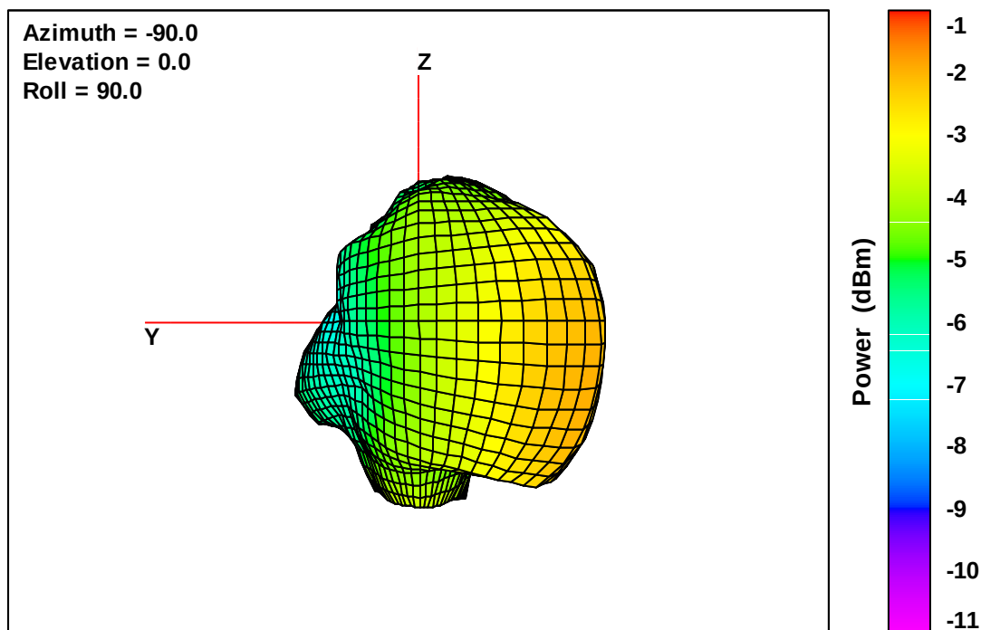
Wearable Defibrillator Free-Space Total EIRP, Back Face View, 824 MHz
