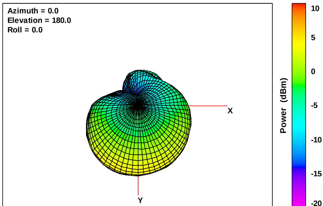
Wearable Defibrillator Free-Space Total EIRP, Bottom View, 2110 MHz
