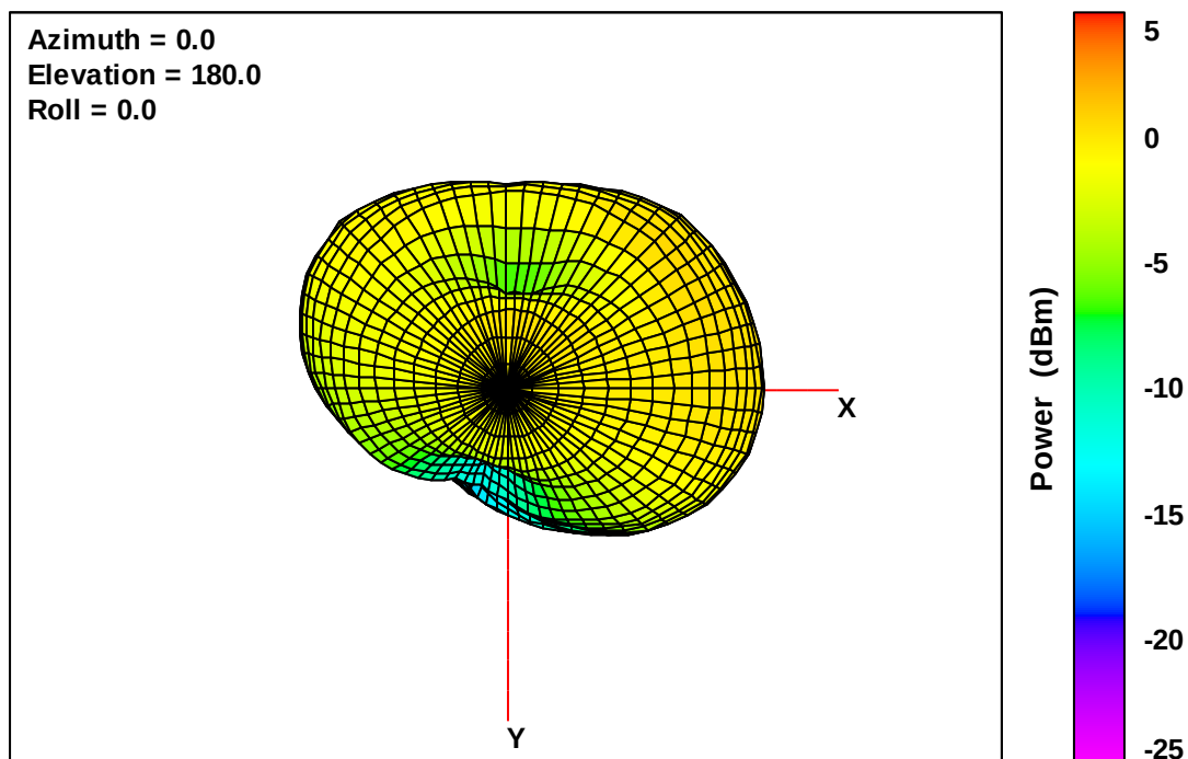
Wearable Defibrillator Free-Space Total EIRP, Bottom View, 713 MHz
