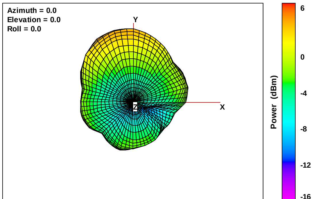
Wearable Defibrillator Free-Space Total EIRP, Top View, 1910 MHz
