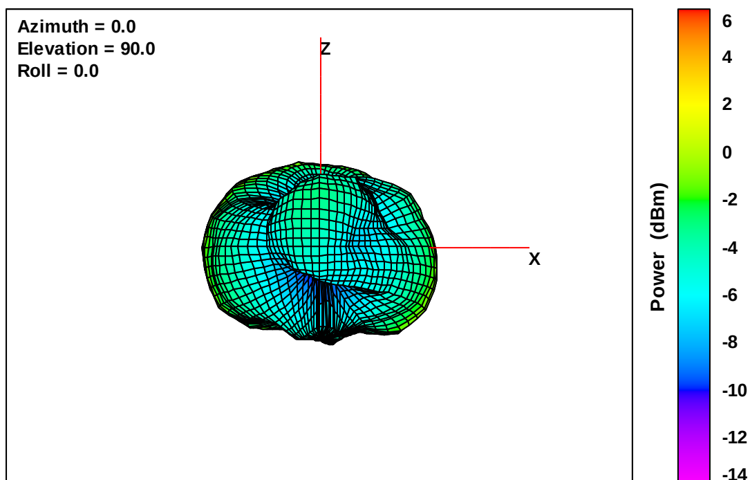
Wearable Defibrillator Free-Space Total EIRP, Left Side View, 1990 MHz
