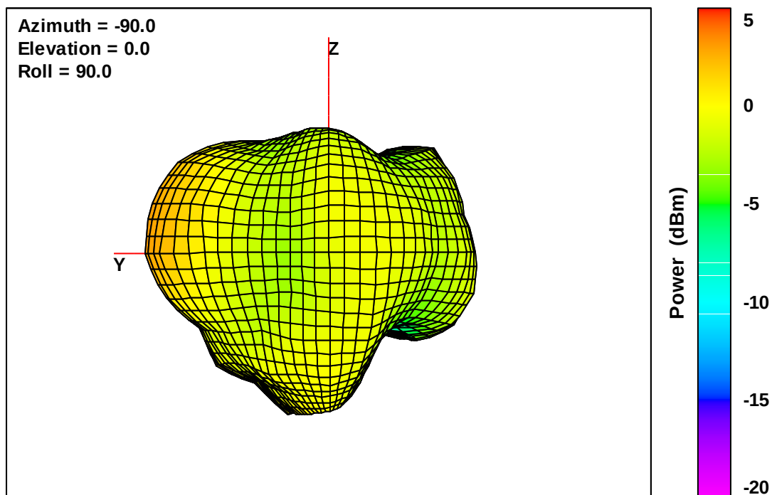
Wearable Defibrillator Free-Space Total EIRP, Back Face View, 1850 MHz
