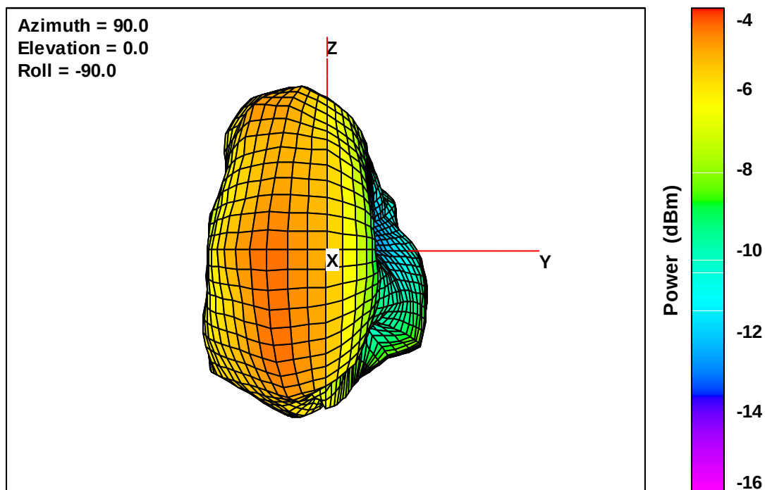
Wearable Defibrillator Free-Space Total EIRP, Front Face View, 869 MHz
