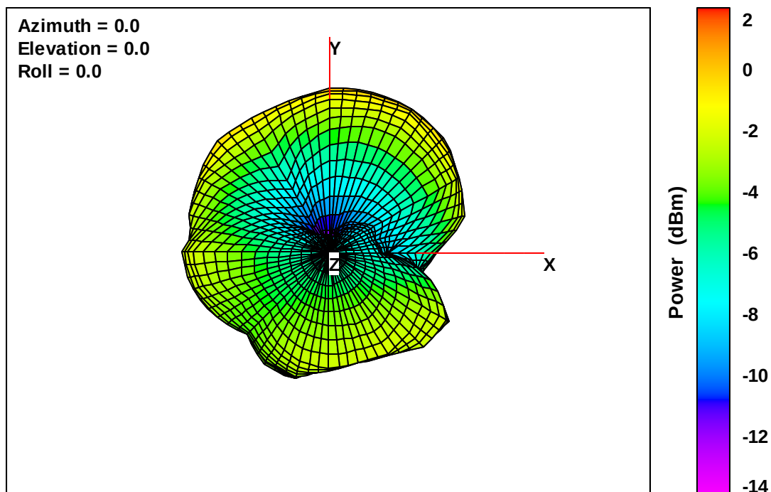
Wearable Defibrillator Free-Space Total EIRP, Top View, 1710 MHz
