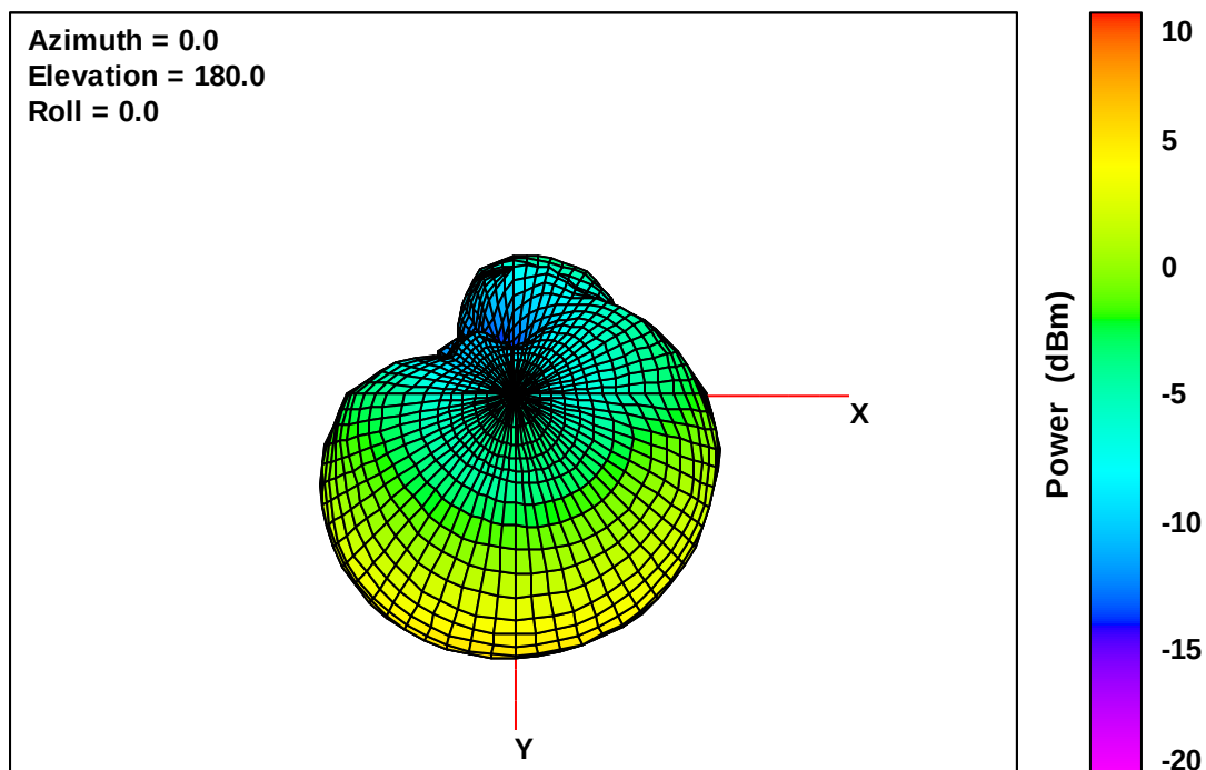
Wearable Defibrillator Free-Space Total EIRP, Bottom View, 2155 MHz
