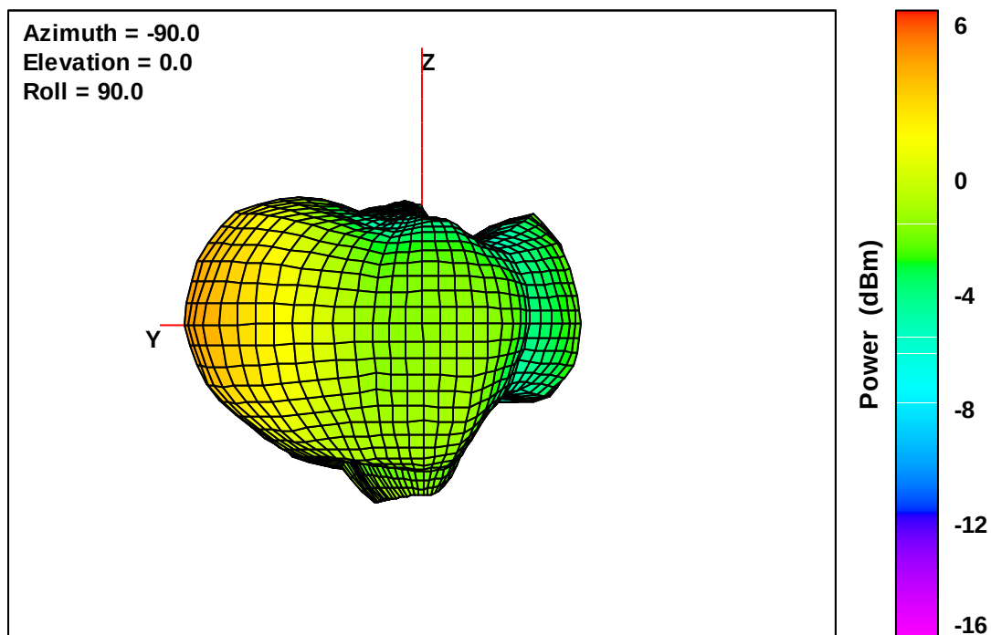
Wearable Defibrillator Free-Space Total EIRP, Back Face View, 1910 MHz
