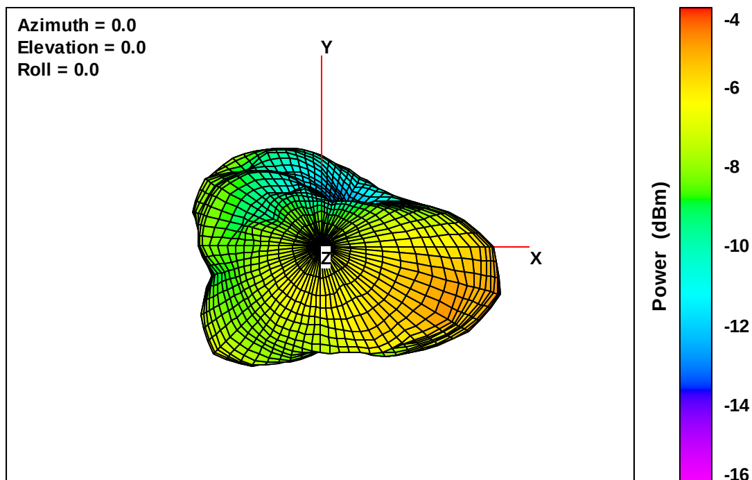
Wearable Defibrillator Free-Space Total EIRP, Top View, 869 MHz
