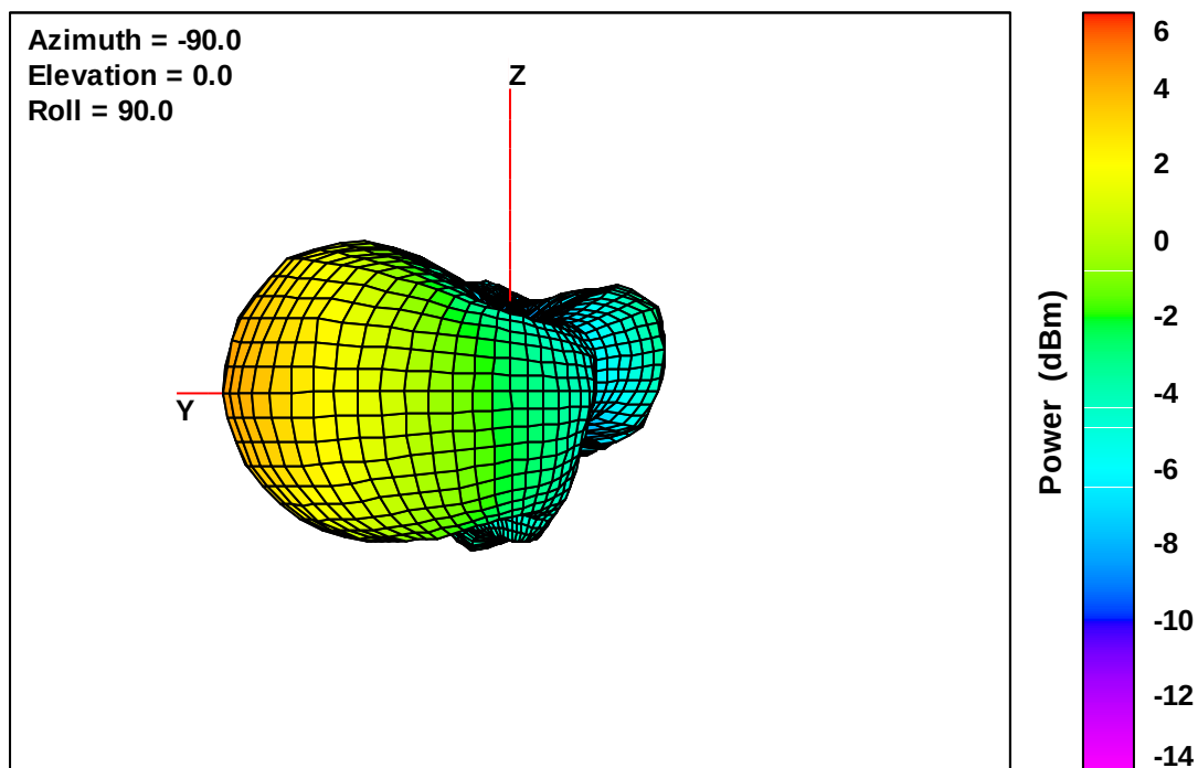
Wearable Defibrillator Free-Space Total EIRP, Back Face View, 1990 MHz
