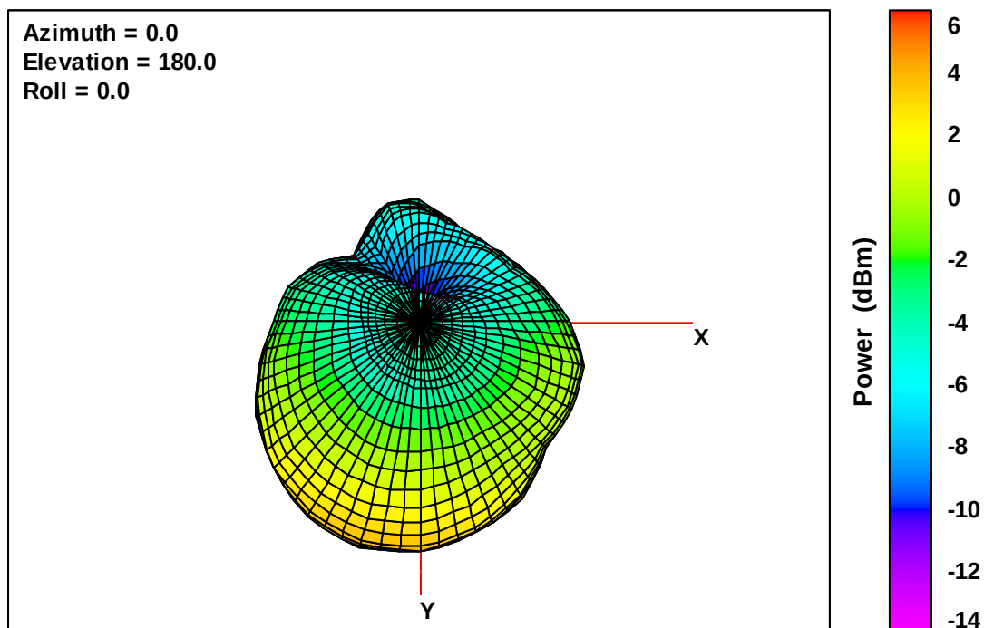
Wearable Defibrillator Free-Space Total EIRP, Bottom View, 1990 MHz
