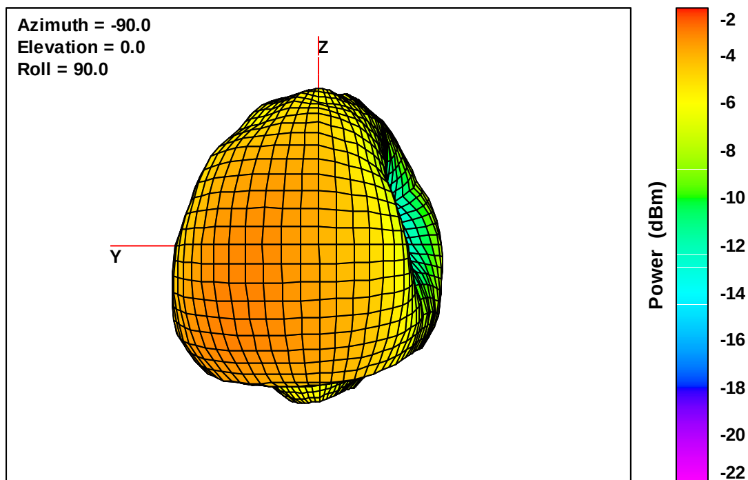
Wearable Defibrillator Free-Space Total EIRP, Back Face View, 960 MHz
