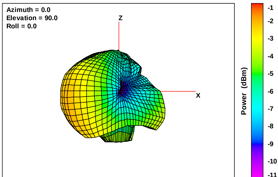
Wearable Defibrillator Free-Space Total EIRP, Left Side View, 824 MHz
