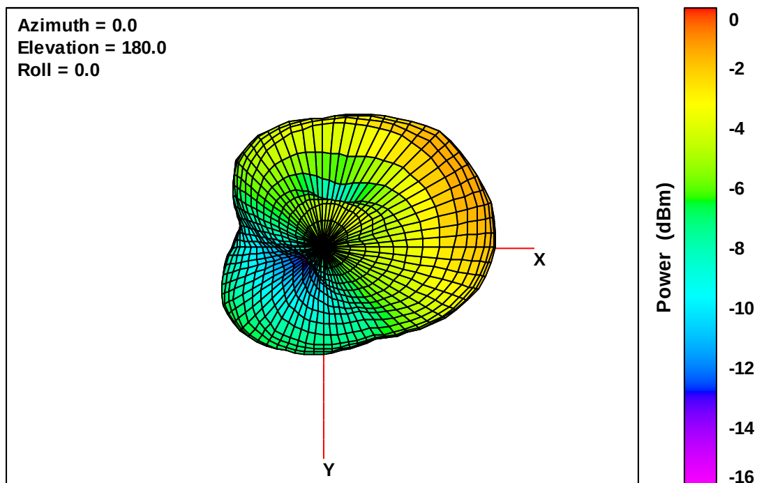
Wearable Defibrillator Free-Space Total EIRP, Bottom View, 756 MHz
