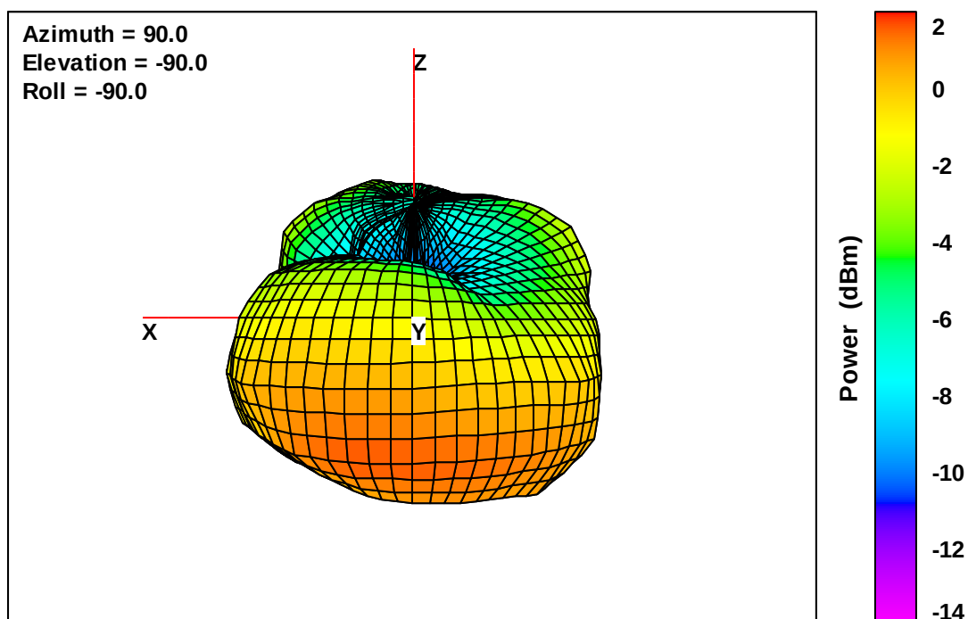
Wearable Defibrillator Free-Space Total EIRP, Right Side View, 1710 MHz
