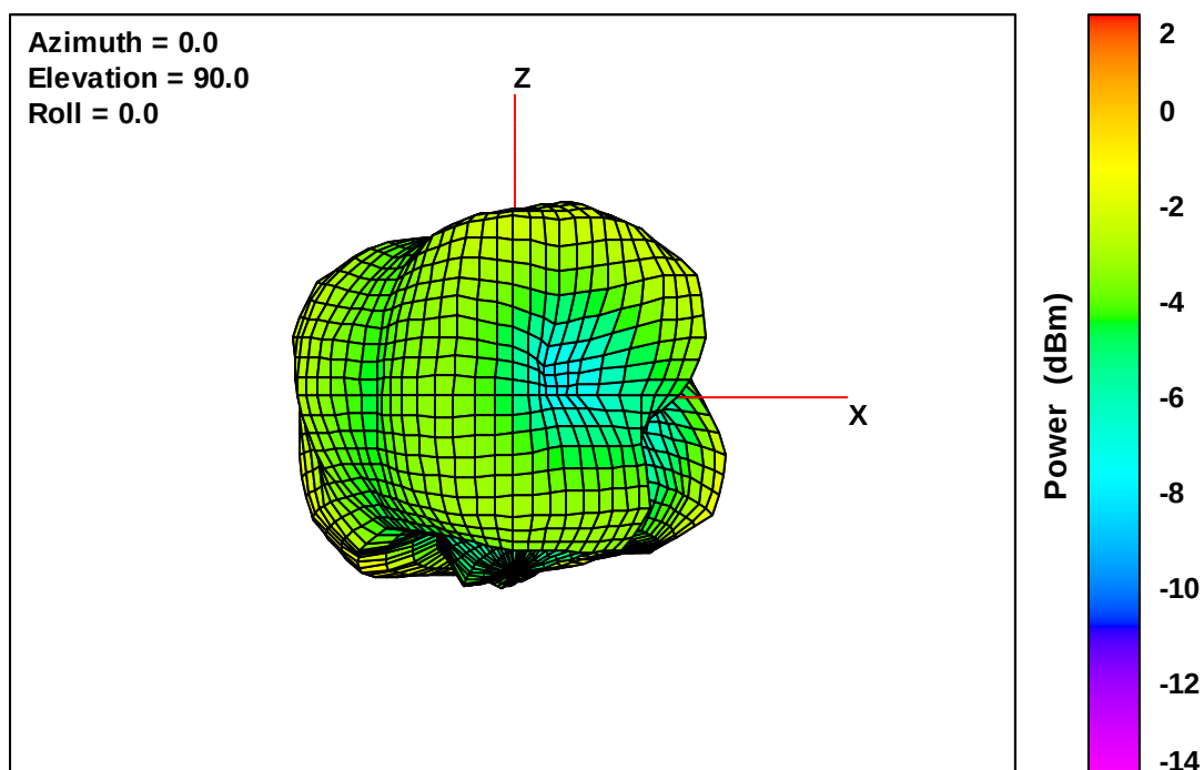
Wearable Defibrillator Free-Space Total EIRP, Left Side View, 1710 MHz
