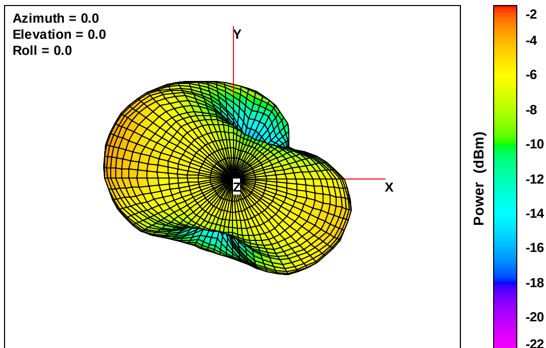
Wearable Defibrillator Free-Space Total EIRP, Top View, 960 MHz
