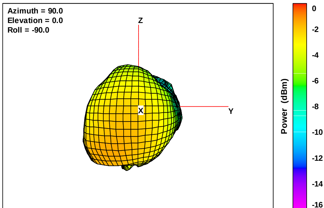
Wearable Defibrillator Free-Space Total EIRP, Front Face View, 756 MHz
