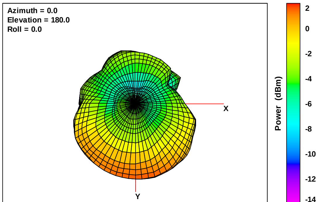
Wearable Defibrillator Free-Space Total EIRP, Bottom View, 1710 MHz
