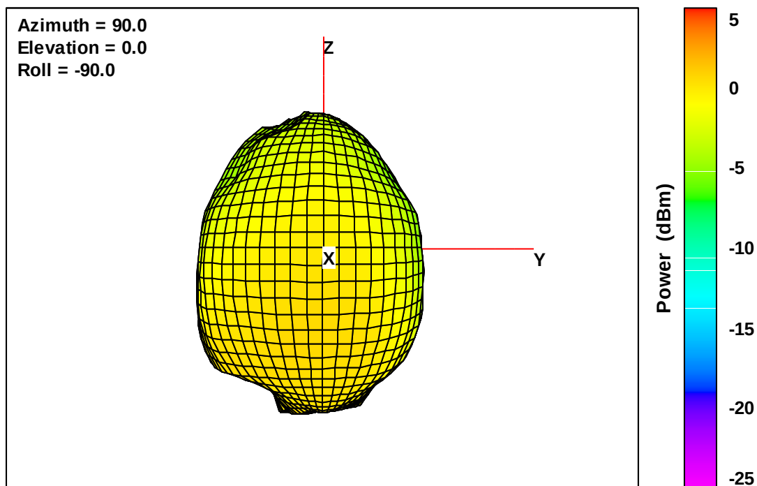
Wearable Defibrillator Free-Space Total EIRP, Front Face View, 699 MHz
