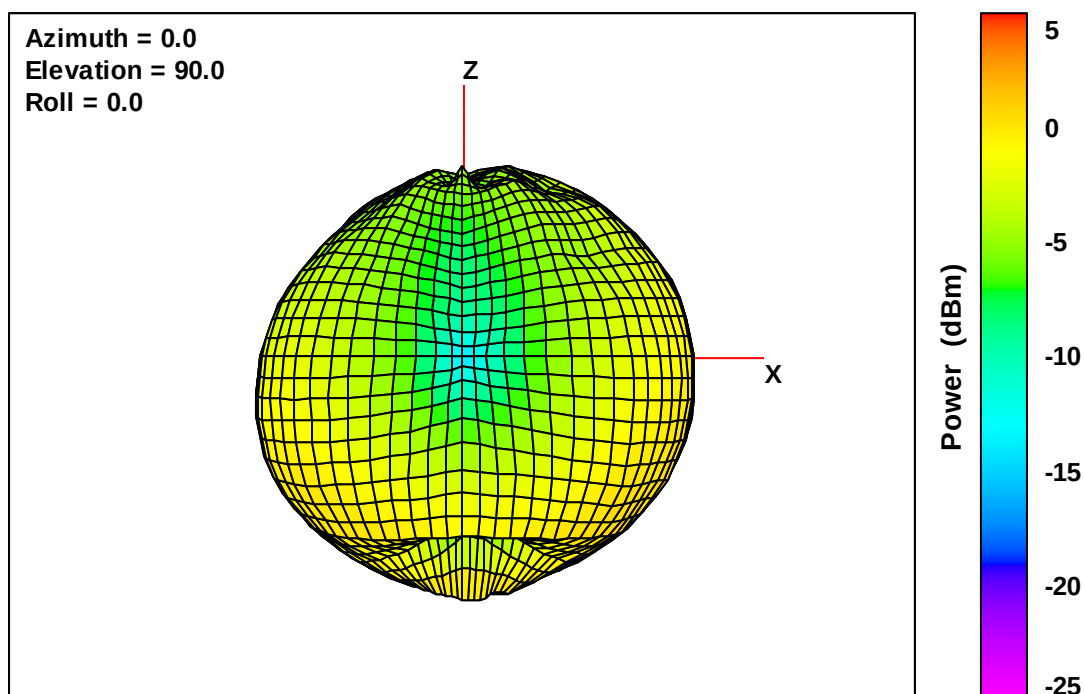
Wearable Defibrillator Free-Space Total EIRP, Left Side View, 699 MHz
