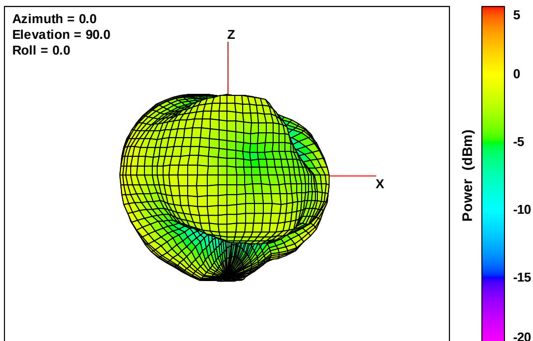
Wearable Defibrillator Free-Space Total EIRP, Left Side View, 1850 MHz
