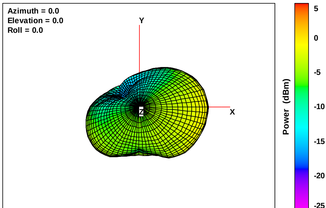
Wearable Defibrillator Free-Space Total EIRP, Top View, 713 MHz
