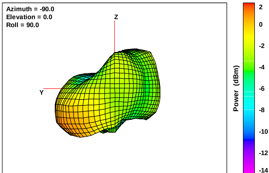
Wearable Defibrillator Free-Space Total EIRP, Back Face View, 1710 MHz
