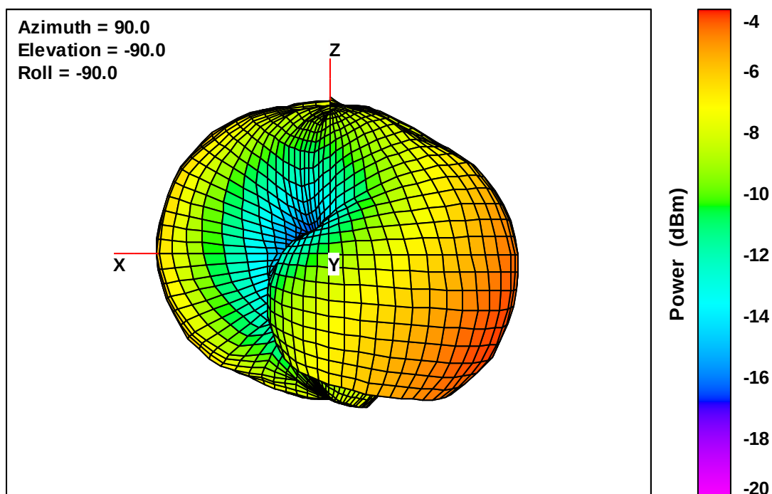
Wearable Defibrillator Free-Space Total EIRP, Right Side View, 915 MHz
