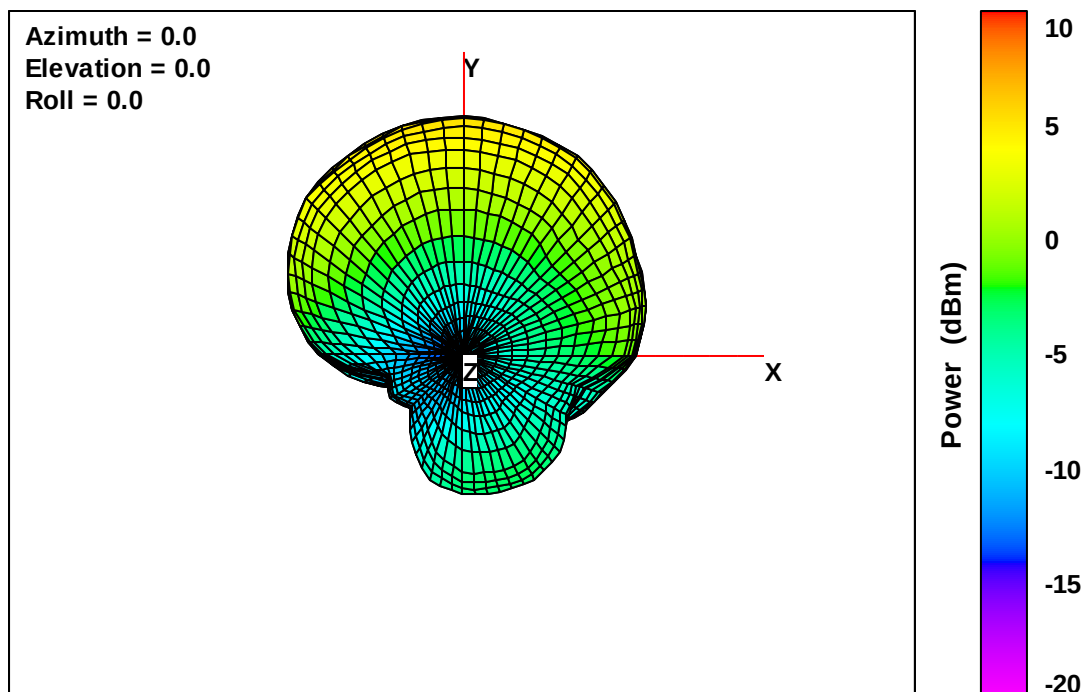
Wearable Defibrillator Free-Space Total EIRP, Top View, 2155 MHz
