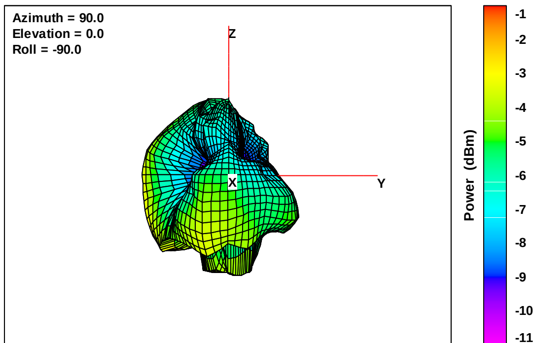
Wearable Defibrillator Free-Space Total EIRP, Front Face View, 824 MHz
