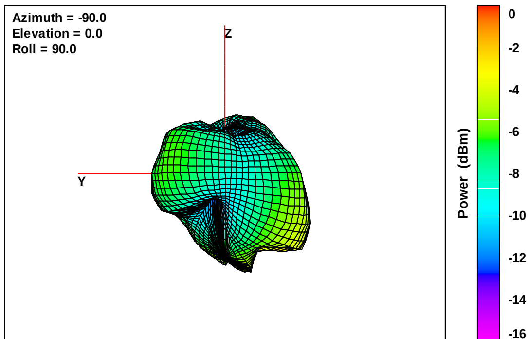
Wearable Defibrillator Free-Space Total EIRP, Back Face View, 756 MHz
