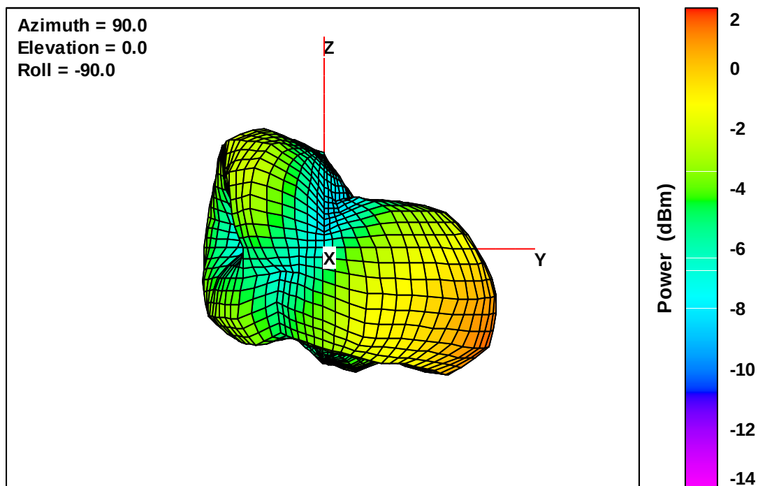
Wearable Defibrillator Free-Space Total EIRP, Front Face View, 1710 MHz
