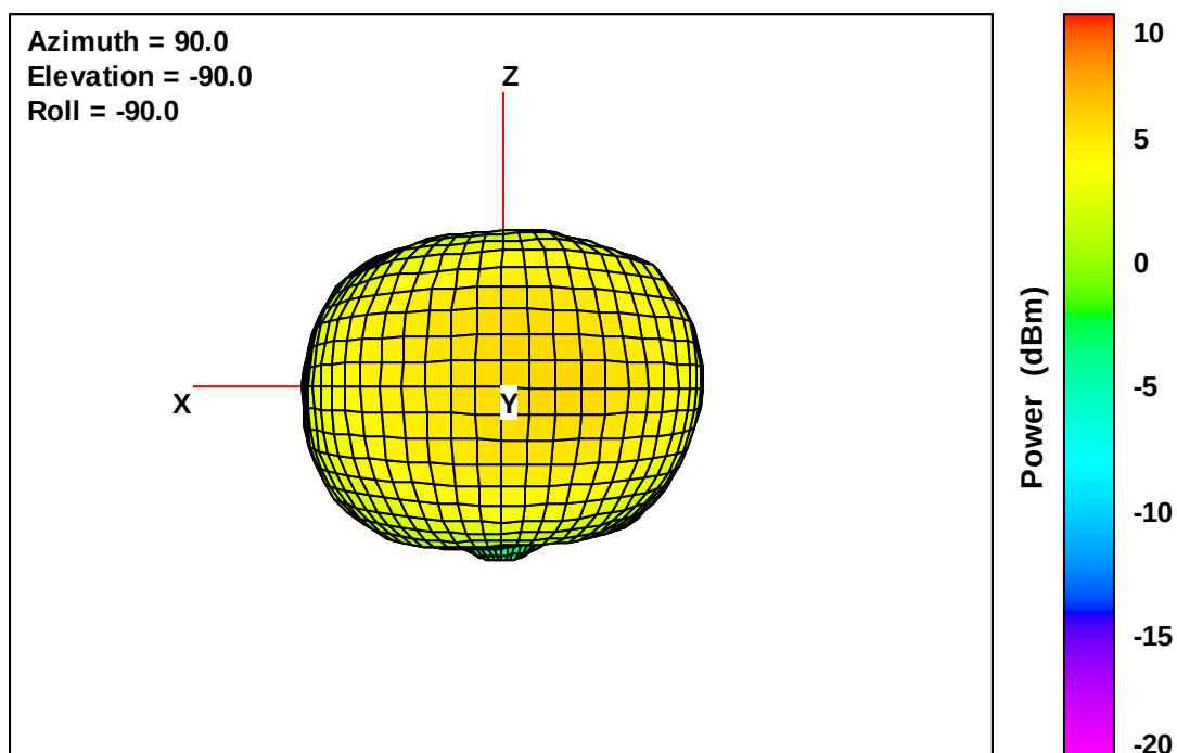
Wearable Defibrillator Free-Space Total EIRP, Right Side View, 2110 MHz
