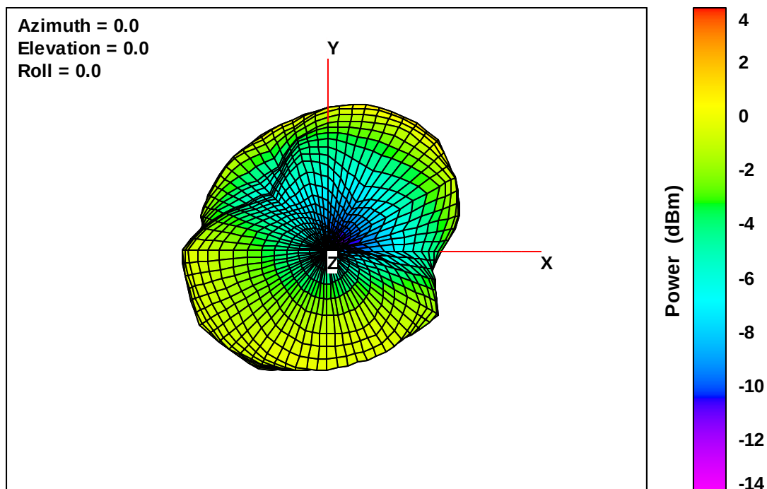
Wearable Defibrillator Free-Space Total EIRP, Top View, 1755 MHz
