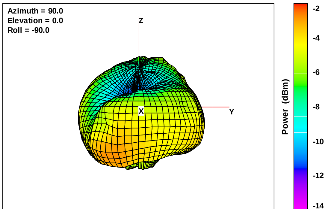
Wearable Defibrillator Free-Space Total EIRP, Front Face View, 787 MHz
