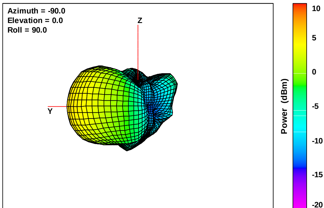
Wearable Defibrillator Free-Space Total EIRP, Back Face View, 2155 MHz
