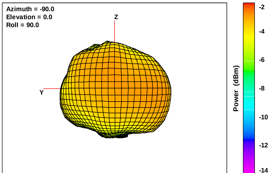
Wearable Defibrillator Free-Space Total EIRP, Back Face View, 787 MHz
