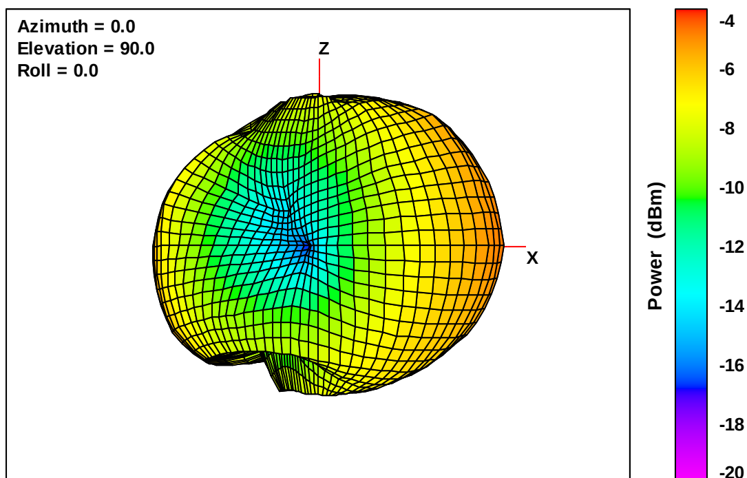
Wearable Defibrillator Free-Space Total EIRP, Left Side View, 915 MHz
