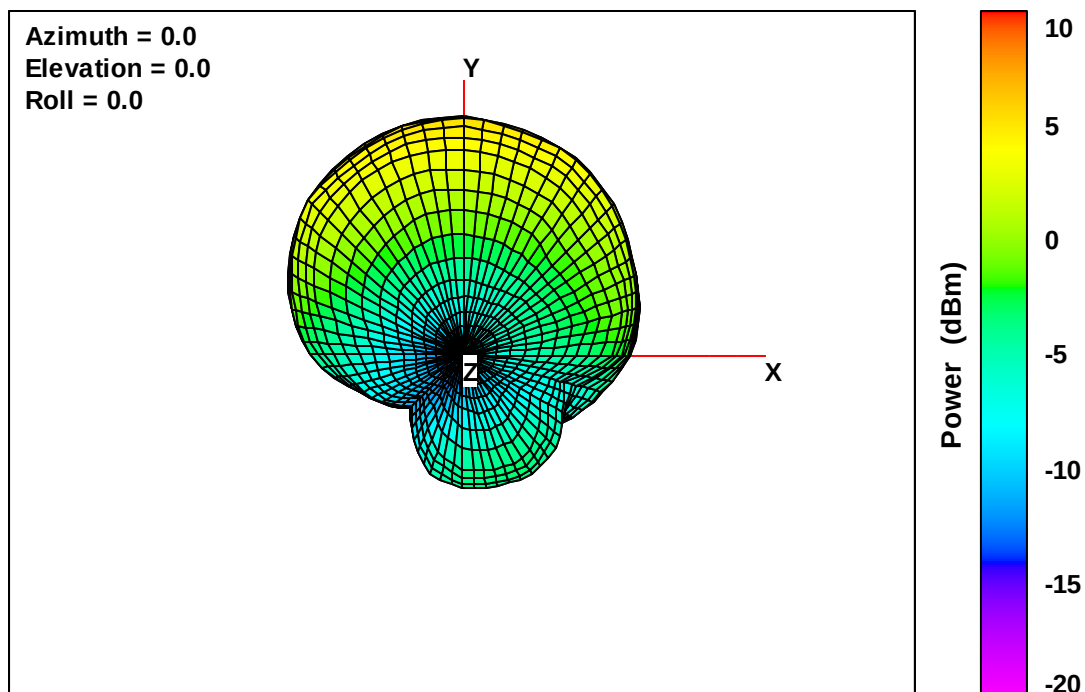
Wearable Defibrillator Free-Space Total EIRP, Top View, 2110 MHz
