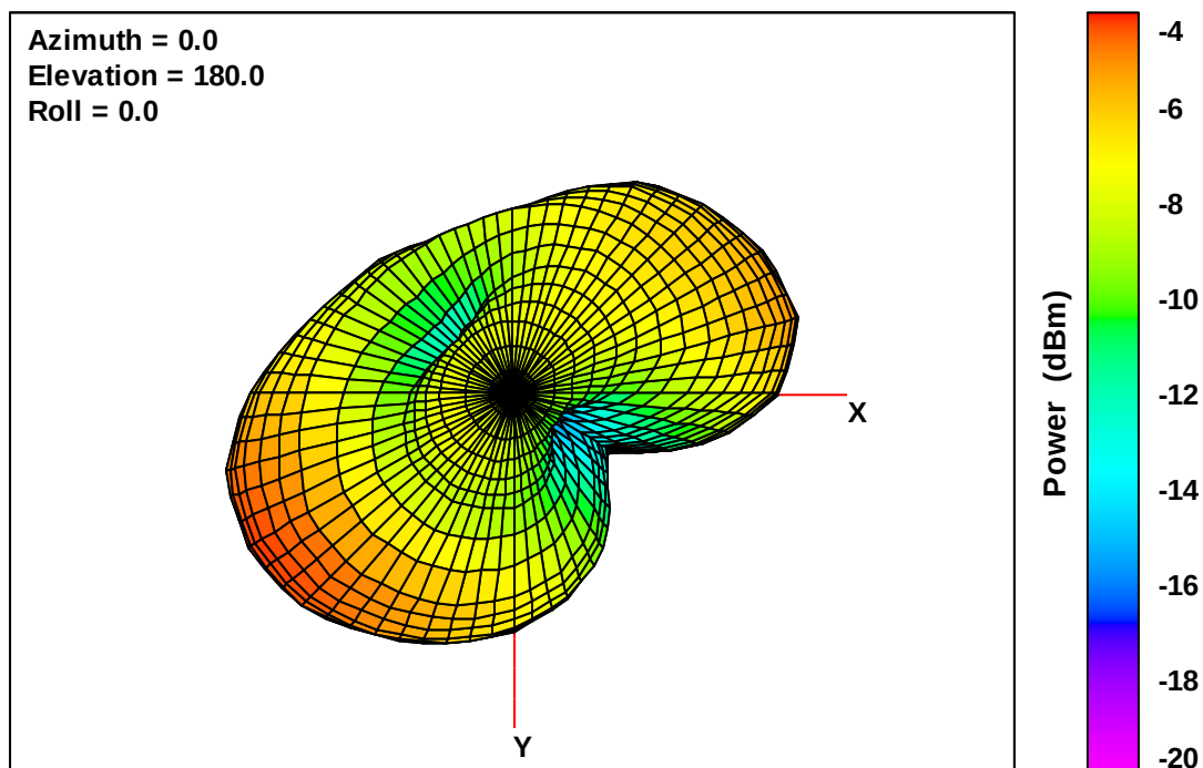
Wearable Defibrillator Free-Space Total EIRP, Bottom View, 915 MHz
