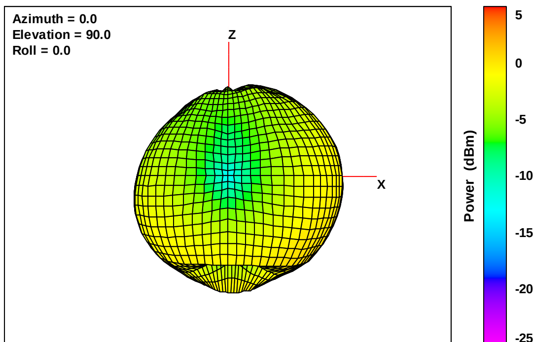
Wearable Defibrillator Free-Space Total EIRP, Left Side View, 713 MHz
