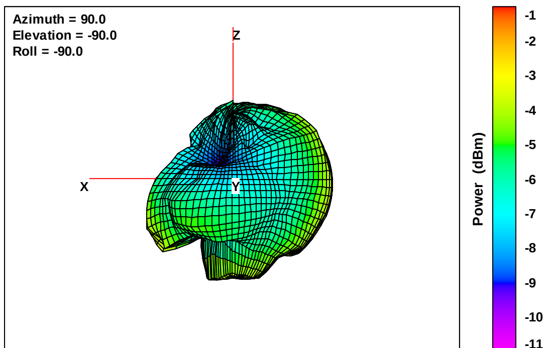
Wearable Defibrillator Free-Space Total EIRP, Right Side View, 824 MHz
