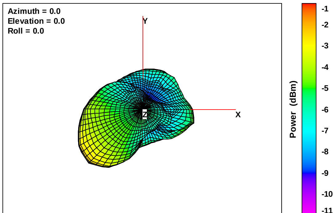
Wearable Defibrillator Free-Space Total EIRP, Top View, 824 MHz
