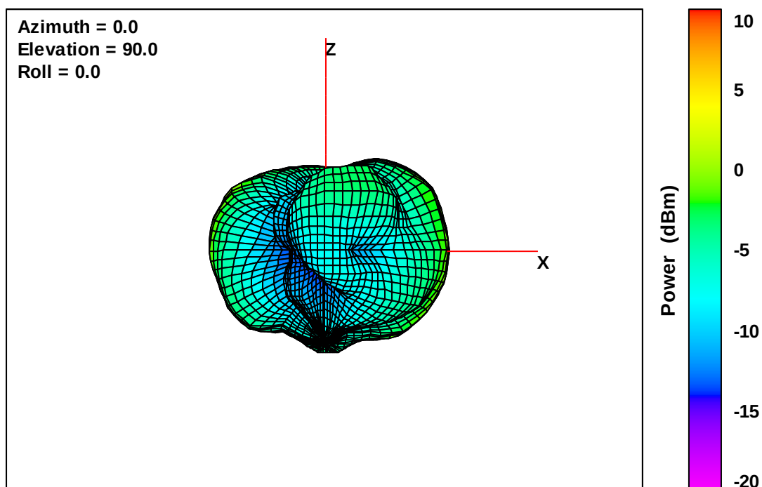
Wearable Defibrillator Free-Space Total EIRP, Left Side View, 2155 MHz
