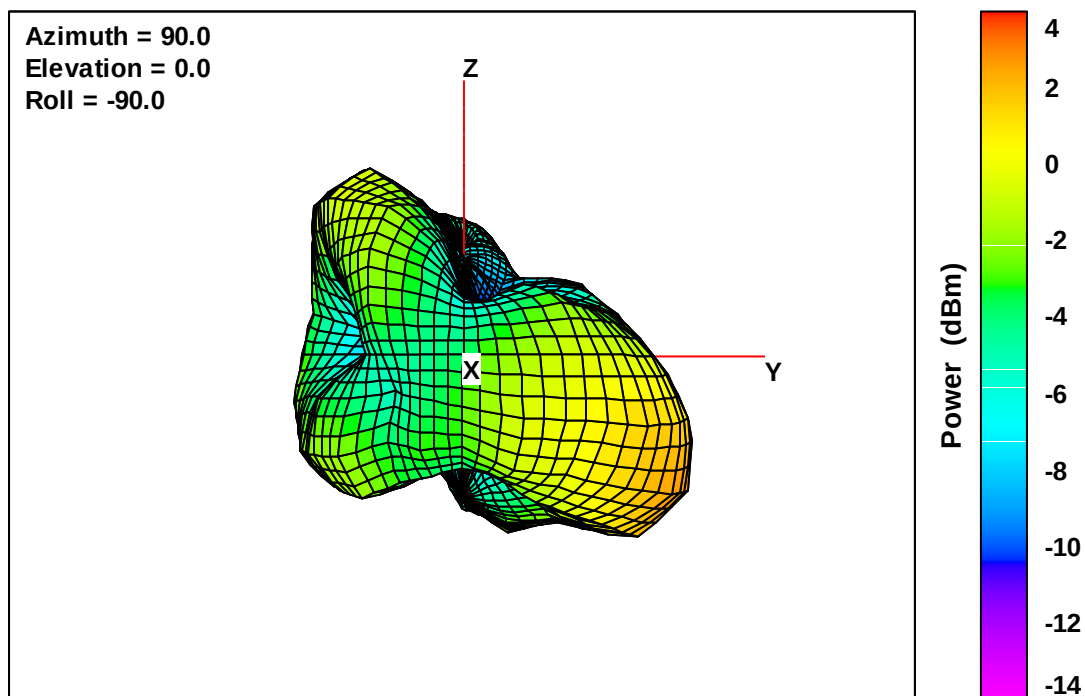
Wearable Defibrillator Free-Space Total EIRP, Front Face View, 1755 MHz
