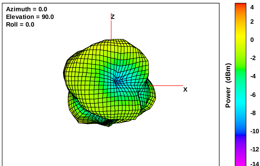
Wearable Defibrillator Free-Space Total EIRP, Left Side View, 1755 MHz
