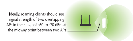
XAP-1240 Multiple AP Coverage and Overlap
