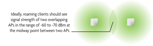
XAP-810 Multiple AP Coverage and Overlap
