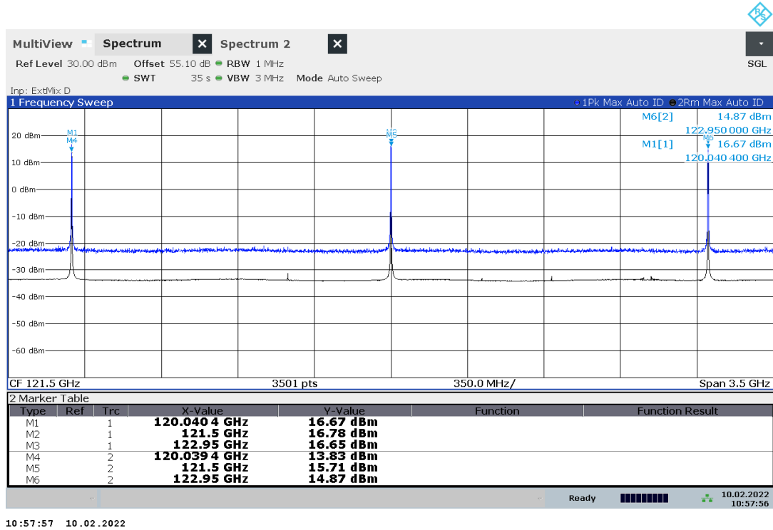
Plot no. 5: Peak power / Average power, Master, 3 GHz mode, BMT (informative plot)
