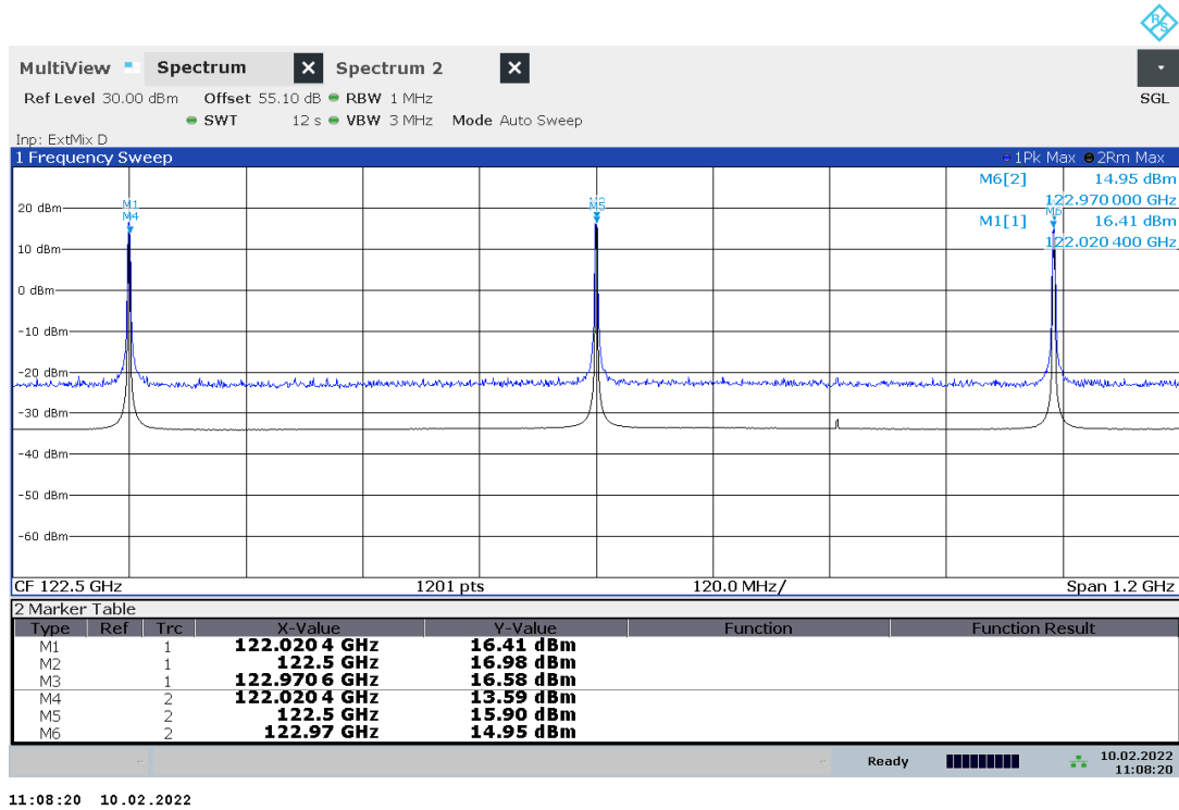
Plot no. 6: Peak power / Average power, Master, 1 GHz mode, BMT (informative plot)
