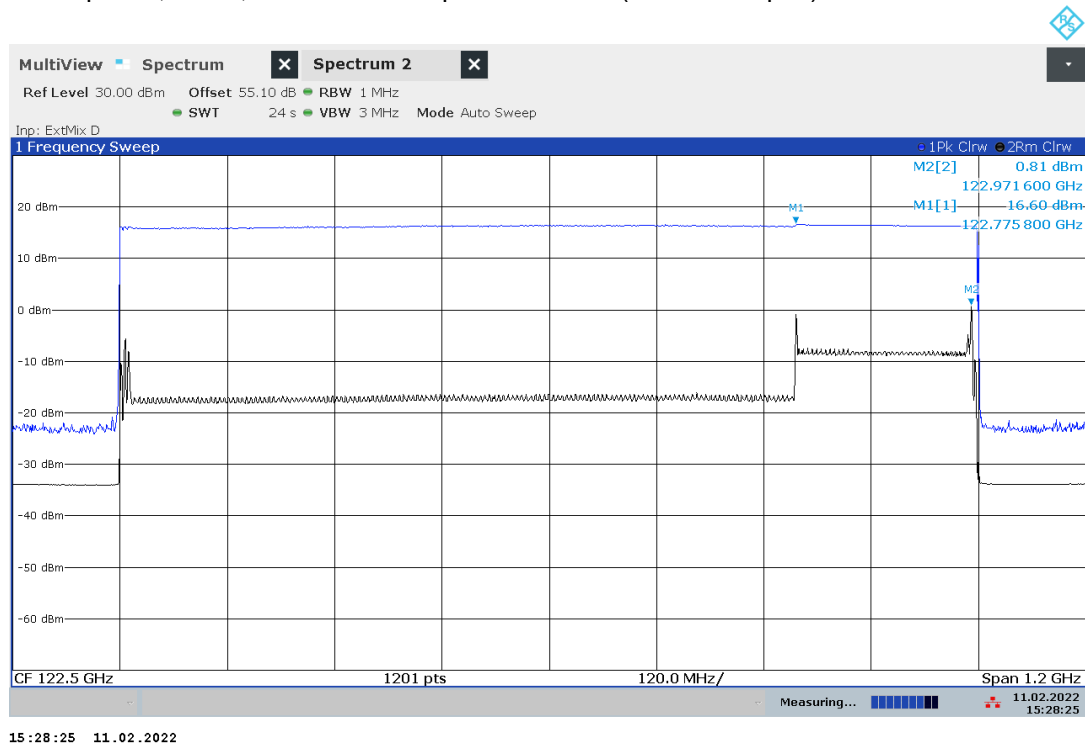
Plot no. 17: Peak power, Slave, 1 GHz normal operation mode (informative plot)
