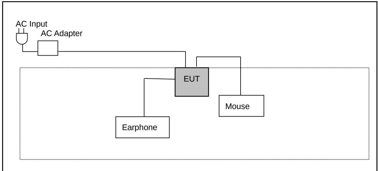
AC Power Conducted Emission
