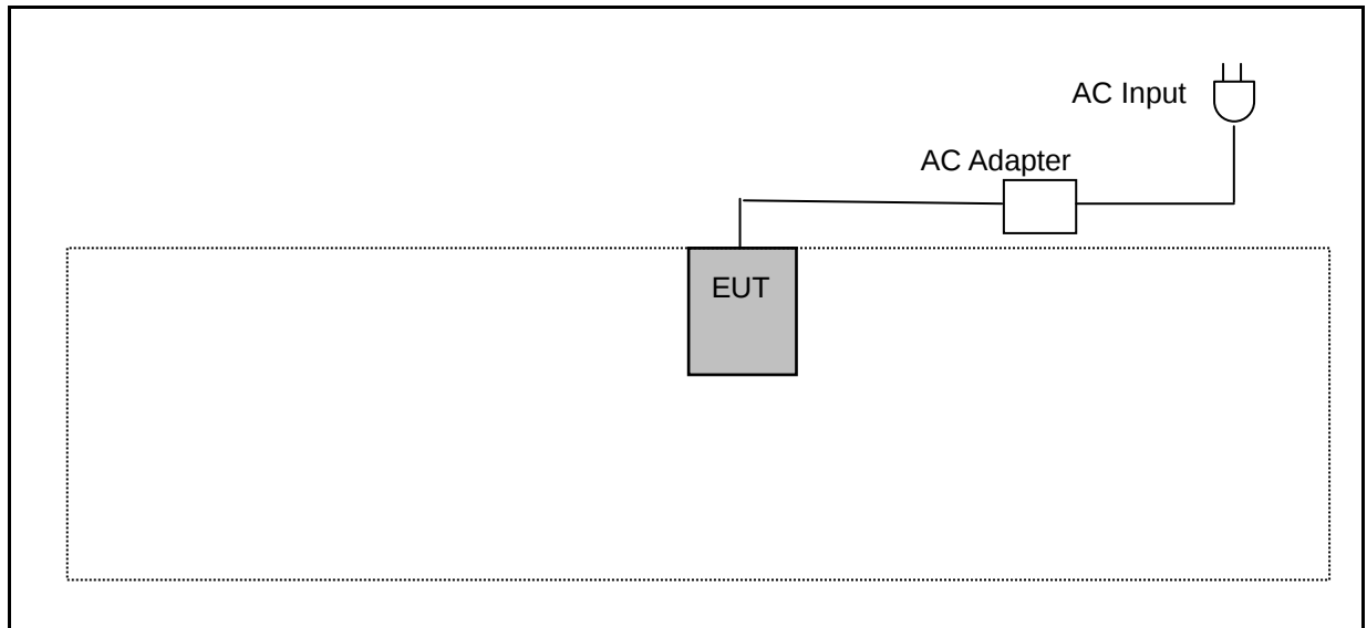
Radiated Emissions
