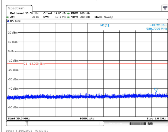
1882.5 MHz_3M_1RB_QPSK_Below 1GHz
