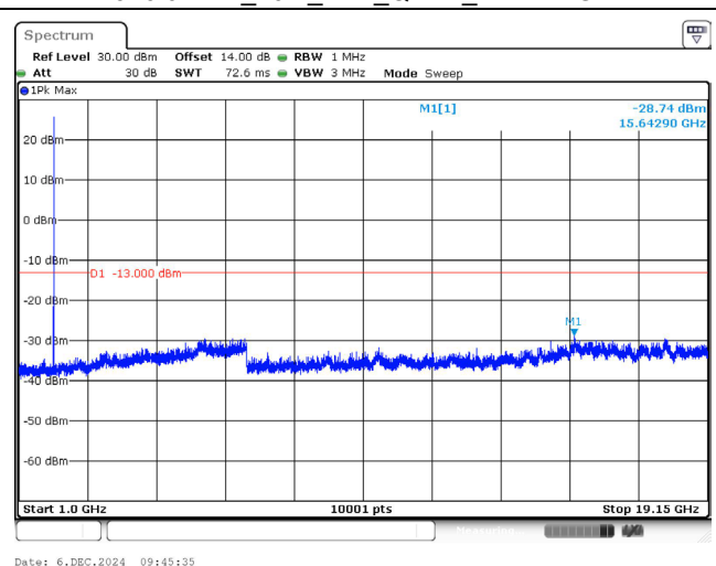
1910.0 MHz_10M_1RB_QPSK_Above 1GHz
