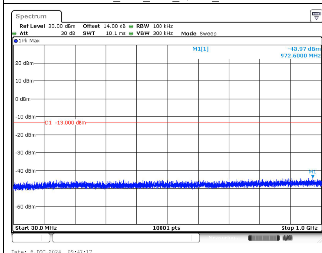
1882.5 MHz_15M_1RB_QPSK_Below 1GHz
