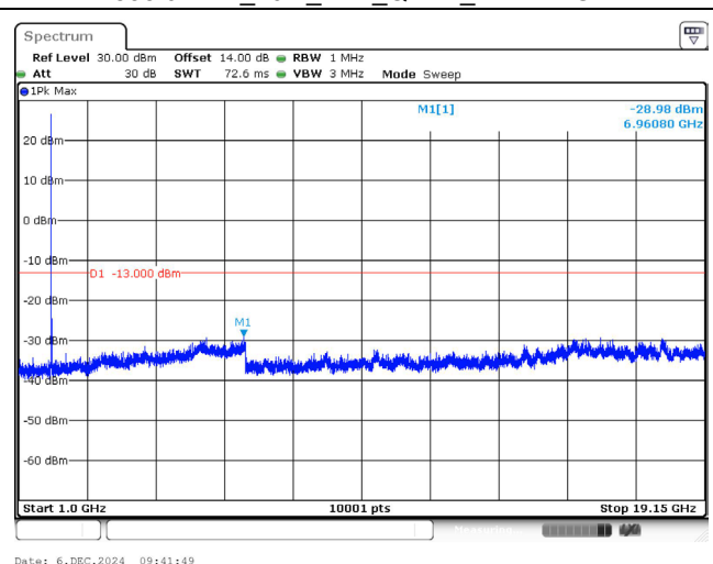
1855.0 MHz_10M_1RB_QPSK_Above 1GHz
