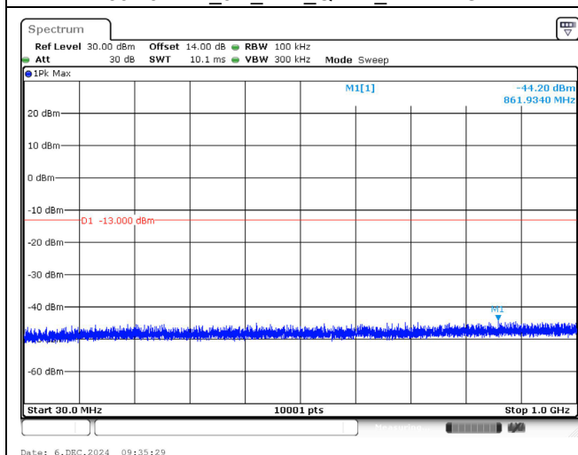
1852.5 MHz_5M_1RB_QPSK_Below 1GHz
