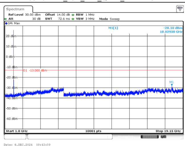
1882.5 MHz_10M_1RB_QPSK_Above 1GHz
