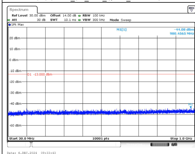
1913.5 MHz_3M_1RB_QPSK_Below 1GHz
