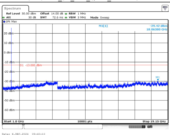
1912.5 MHz_5M_1RB_QPSK_Above 1GHz
