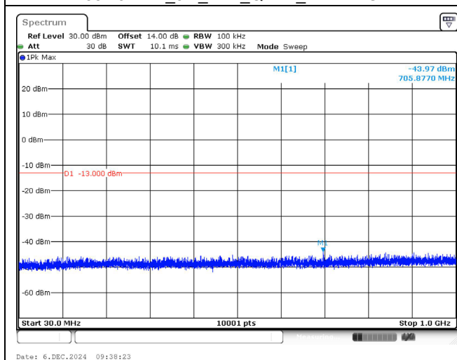
1882.5 MHz_5M_1RB_QPSK_Below 1GHz
