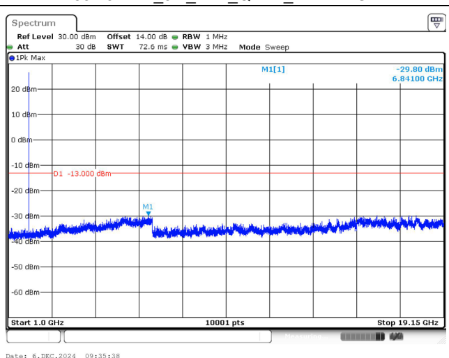
1852.5 MHz_5M_1RB_QPSK_Above 1GHz
