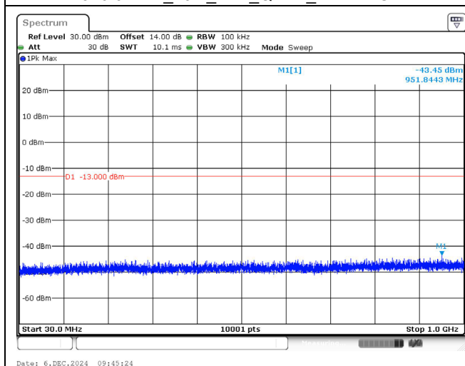
1910.0 MHz_10M_1RB_QPSK_Below 1GHz
