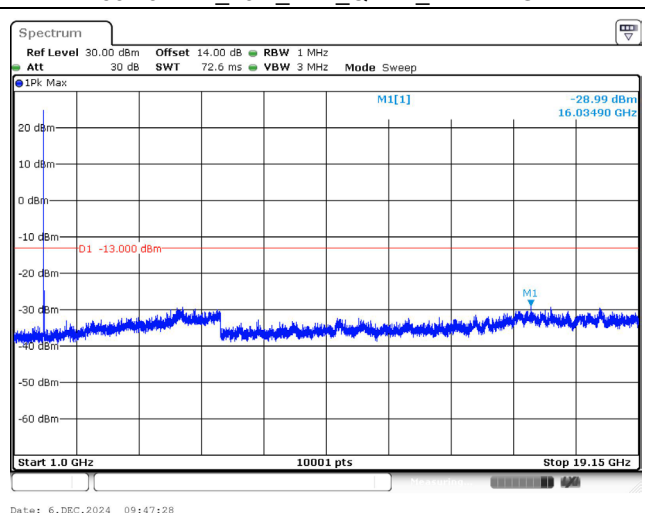
1882.5 MHz_15M_1RB_QPSK_Above 1GHz
