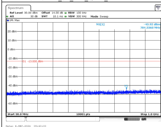
1912.5 MHz_5M_1RB_QPSK_Below 1GHz
