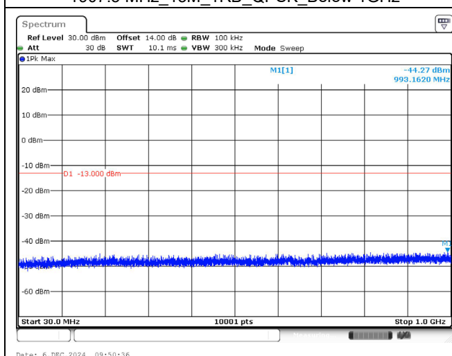
1907.5 MHz_15M_1RB_QPSK_Below 1GHz
