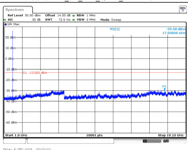
1851.5 MHz_3M_1RB_QPSK_Above 1GHz
