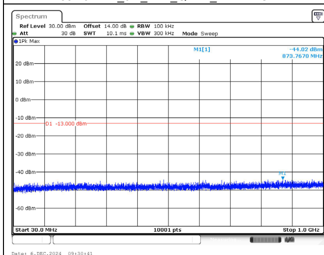
1851.5 MHz_3M_1RB_QPSK_Below 1GHz
