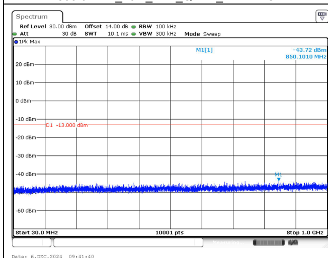
1855.0 MHz_10M_1RB_QPSK_Below 1GHz
