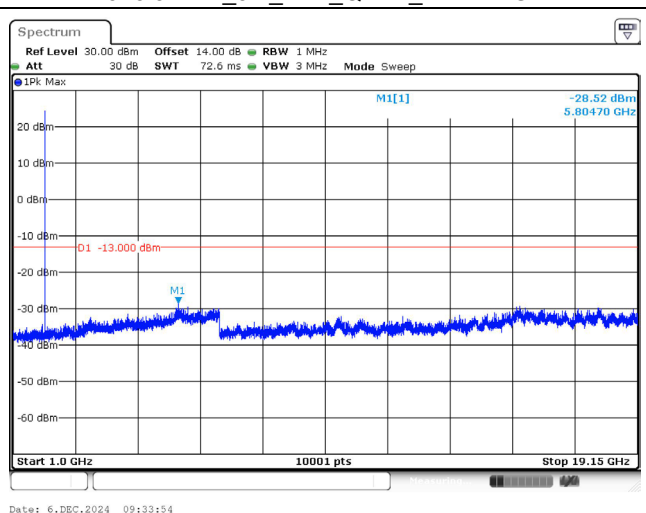
1913.5 MHz_3M_1RB_QPSK_Above 1GHz
