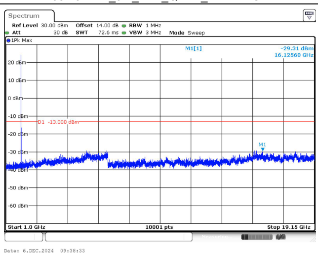
1882.5 MHz_5M_1RB_QPSK_Above 1GHz
