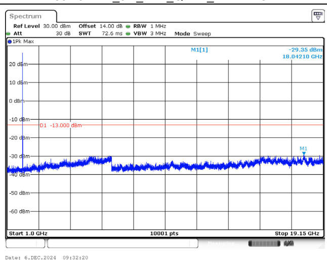
1882.5 MHz_3M_1RB_QPSK_Above 1GHz
