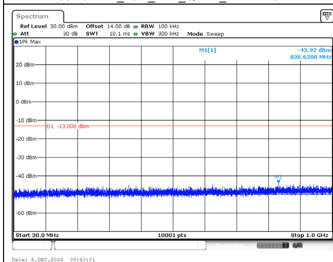
1882.5 MHz_10M_1RB_QPSK_Below 1GHz
