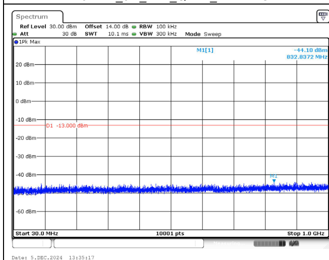
1745.0 MHz_5M_1RB_QPSK_Below 1GHz
