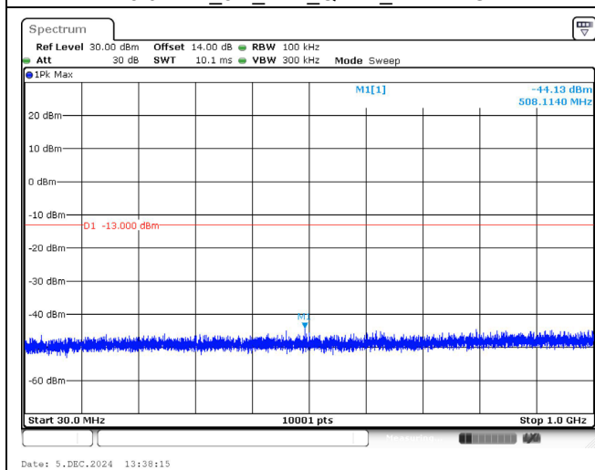
1777.5 MHz_5M_1RB_QPSK_Below 1GHz
