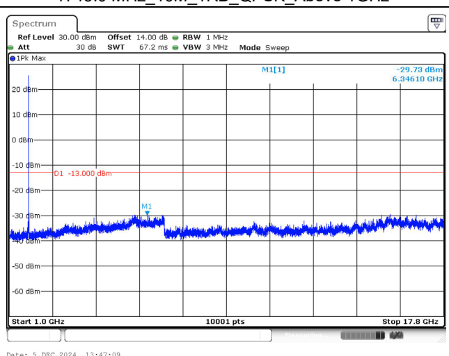
1775.0MHz_10M_1RB_QPSK_Above 1GHz
