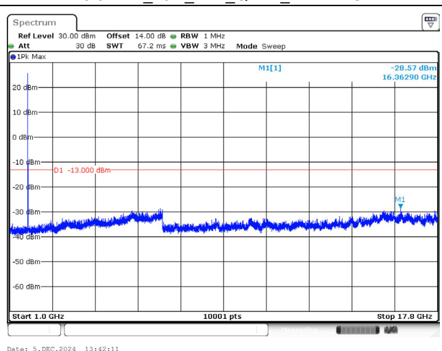
1745.0 MHz_10M_1RB_QPSK_Above 1GHz
