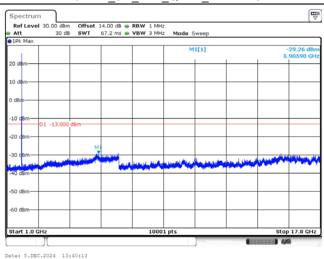
1777.5 MHz_5M_1RB_QPSK_Above 1GHz
