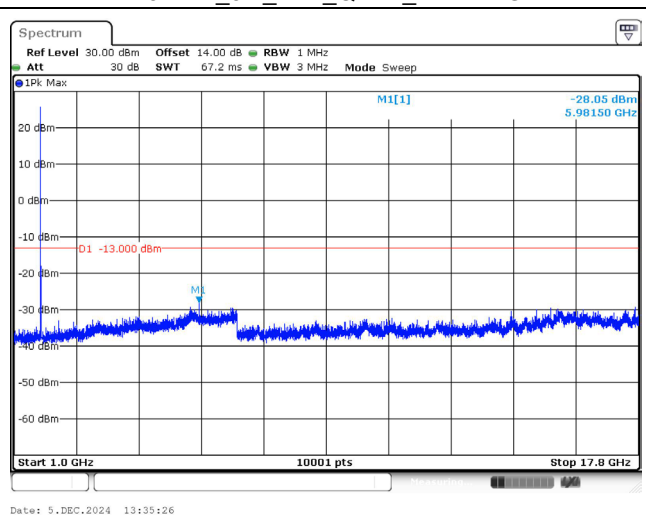
1745.0 MHz_5M_1RB_QPSK_Above 1GHz
