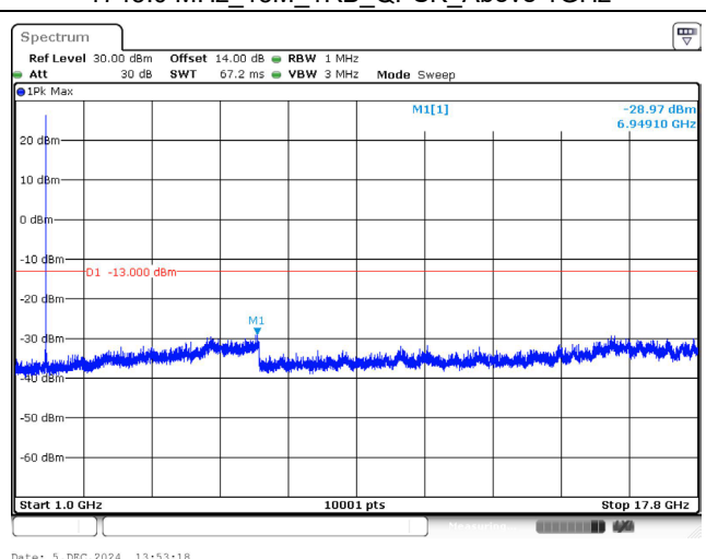
1772.5 MHz_15M_1RB_QPSK_Above 1GHz
