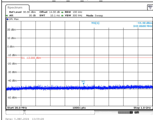
1745.0 MHz_20M_1RB_QPSK_Below 1GHz
