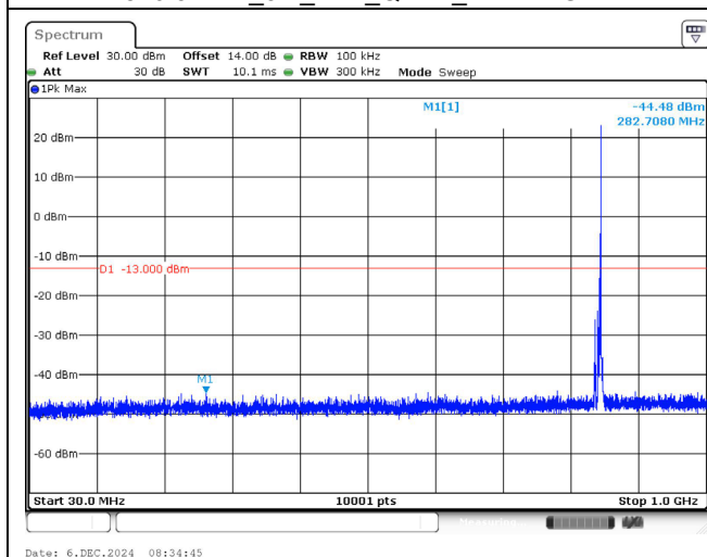
846.5 MHz_5M_1RB_QPSK_Below 1GHz
