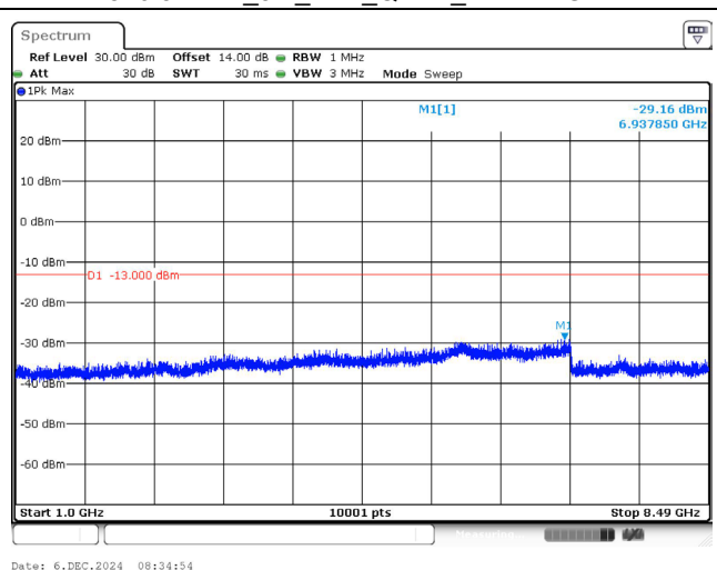
846.5 MHz_5M_1RB_QPSK_Above 1GHz
