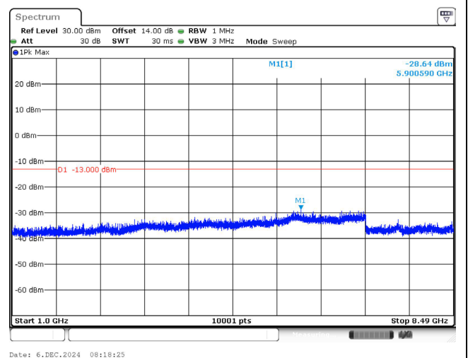
824.7 MHz_1.4M_1RB_QPSK_Above 1GHz
