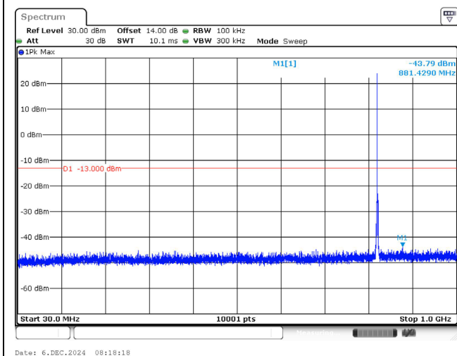
824.7 MHz_1.4M_1RB_QPSK_Below 1GHz
