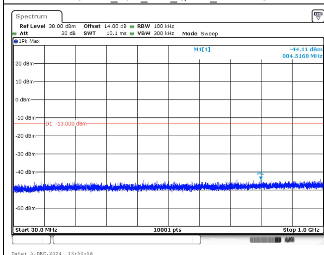
1745.0 MHz_15M_1RB_QPSK_Below 1GHz
