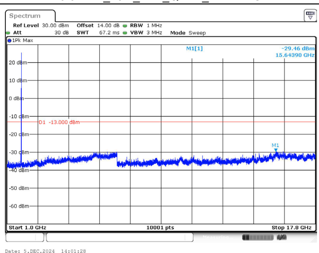
1770.0 MHz_20M_1RB_QPSK_Above 1GHz
