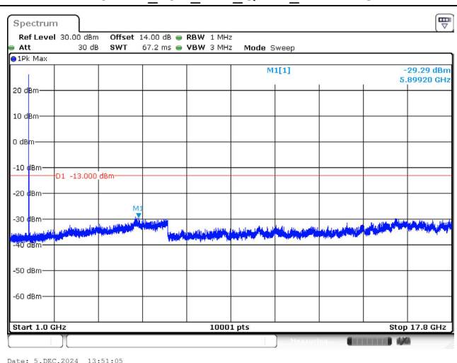
1745.0 MHz_15M_1RB_QPSK_Above 1GHz
