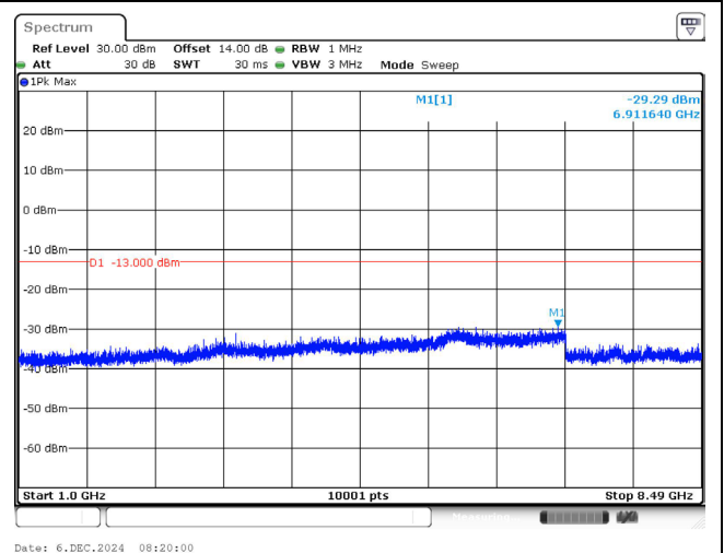
848.3 MHz_1.4M_1RB_QPSK_Above 1GHz
