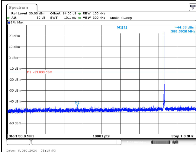
848.3 MHz_1.4M_1RB_QPSK_Below 1GHz
