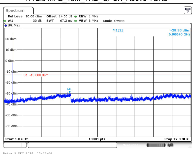
1772.5 MHz_15M_1RB_QPSK_Above 1GHz
