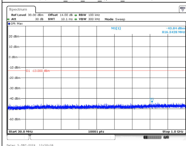
1720.0 MHz_20M_1RB_QPSK_Below 1GHz
