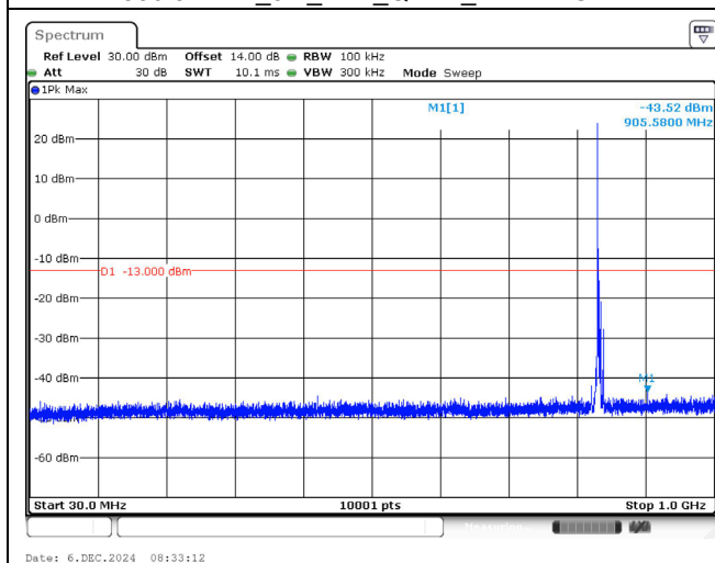
836.5 MHz_5M_1RB_QPSK_Below 1GHz
