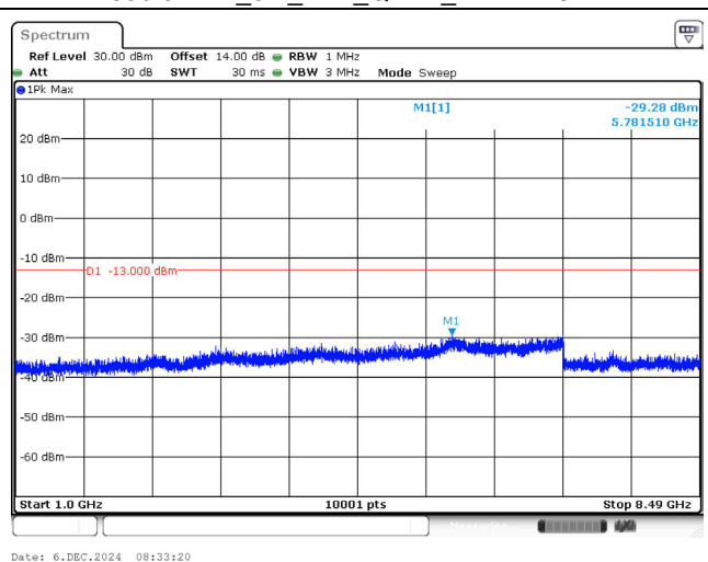
836.5 MHz_5M_1RB_QPSK_Above 1GHz
