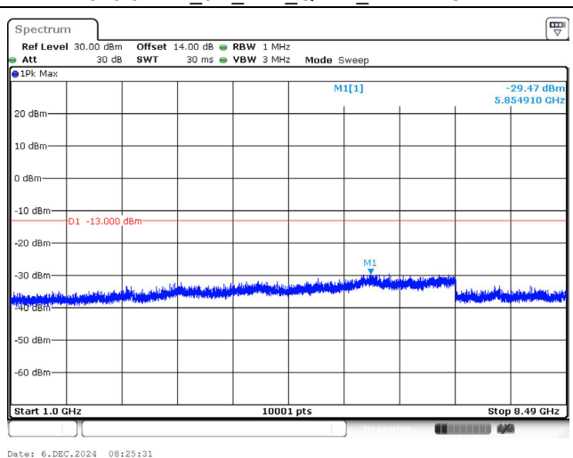
836.5 MHz_3M_1RB_QPSK_Above 1GHz
