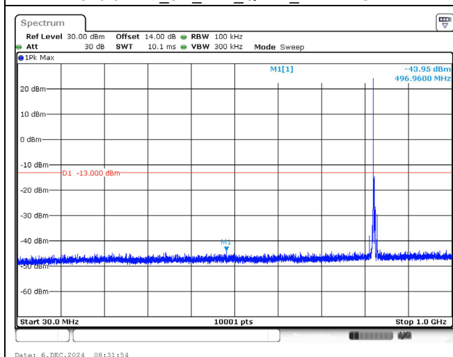
826.5 MHz_5M_1RB_QPSK_Below 1GHz
