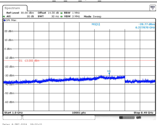
826.5 MHz_5M_1RB_QPSK_Above 1GHz
