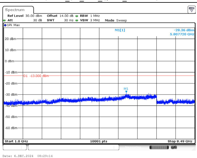
847.5 MHz_3M_1RB_QPSK_Above 1GHz
