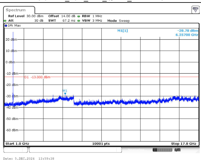
1745.0 MHz_20M_1RB_QPSK_Above 1GHz
