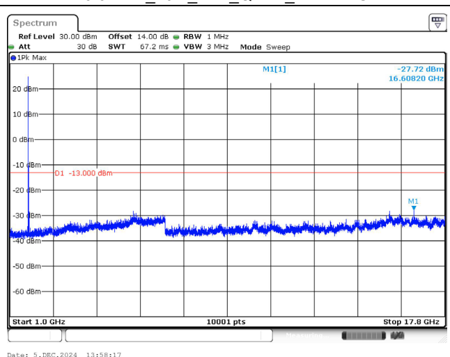
1720.0 MHz_20M_1RB_QPSK_Above 1GHz
