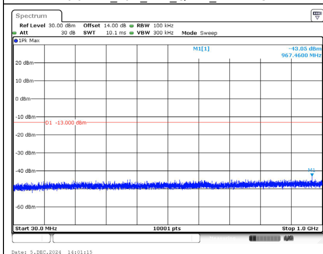
1770.0 MHz_20M_1RB_QPSK_Below 1GHz
