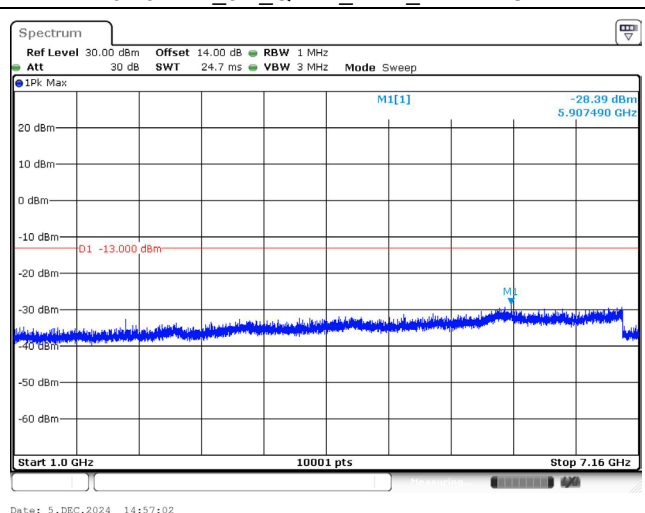
707.5 MHz_5M_QPSK_1RB_Above 1GHz
