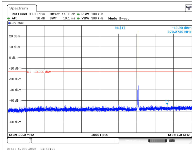
715.3 MHz_1.4M_QPSK_1RB_Below 1GHz
