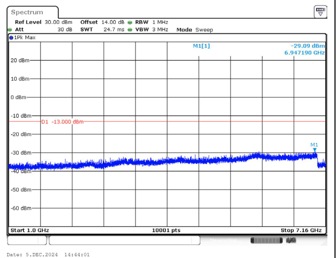
707.5 MHz_1.4M_QPSK_1RB_Above 1GHz
