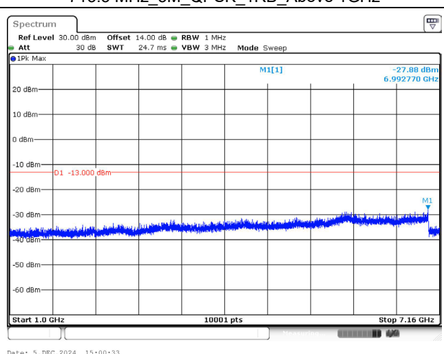
713.5 MHz_5M_QPSK_1RB_Above 1GHz
