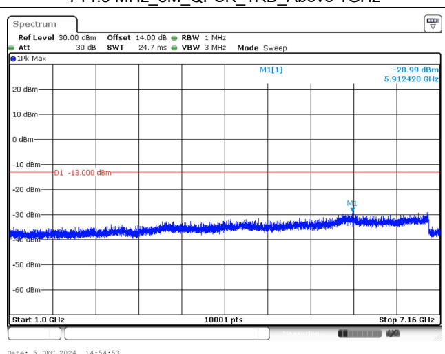
714.5 MHz_3M_QPSK_1RB_Above 1GHz
