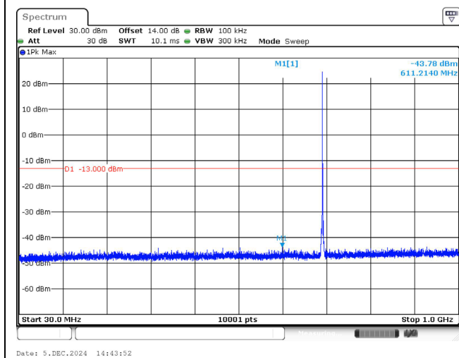
707.5 MHz_1.4M_QPSK_1RB_Below 1GHz
