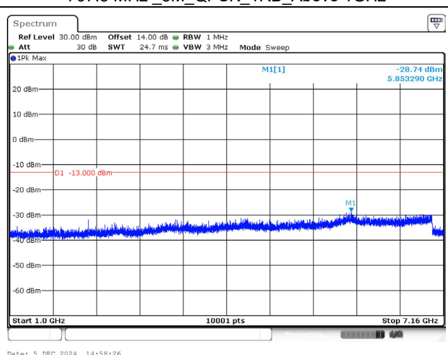
713.5 MHz_5M_QPSK_1RB_Above 1GHz
