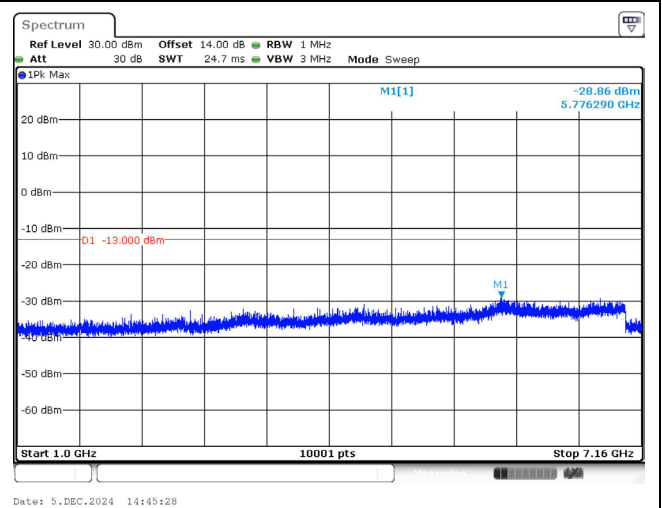
715.3 MHz_1.4M_QPSK_1RB_Above 1GHz
