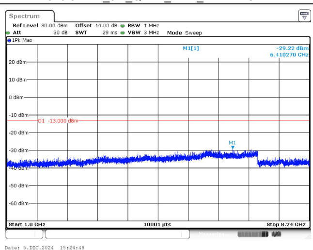
819.0 MHz_3M_QPSK_1RB_Above 1GHz
