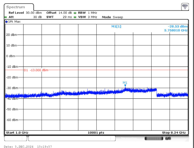
814.7 MHz_1.4M_QPSK_1RB_Above 1GHz
