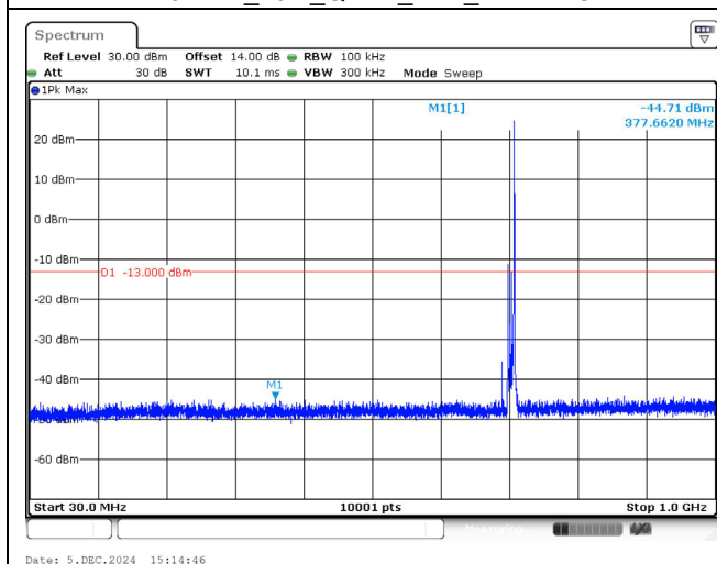
711.0 MHz_10M_QPSK_1RB_Below 1GHz
