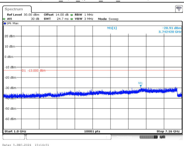
711.0 MHz_10M_QPSK_1RB_Above 1GHz
