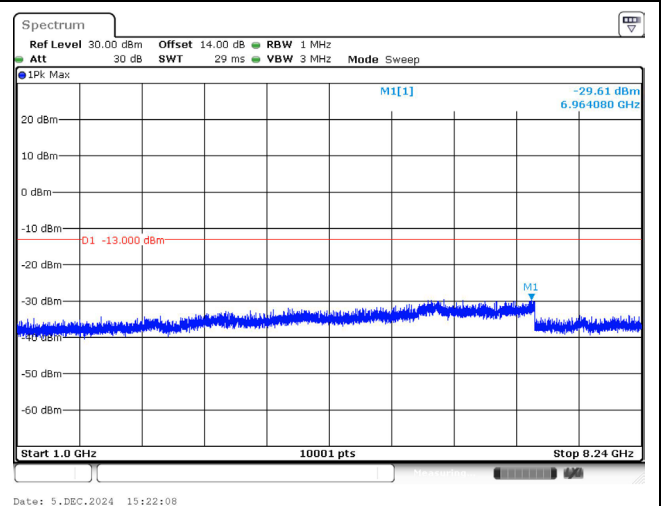
823.3 MHz_1.4M_QPSK_1RB_Above 1GHz
