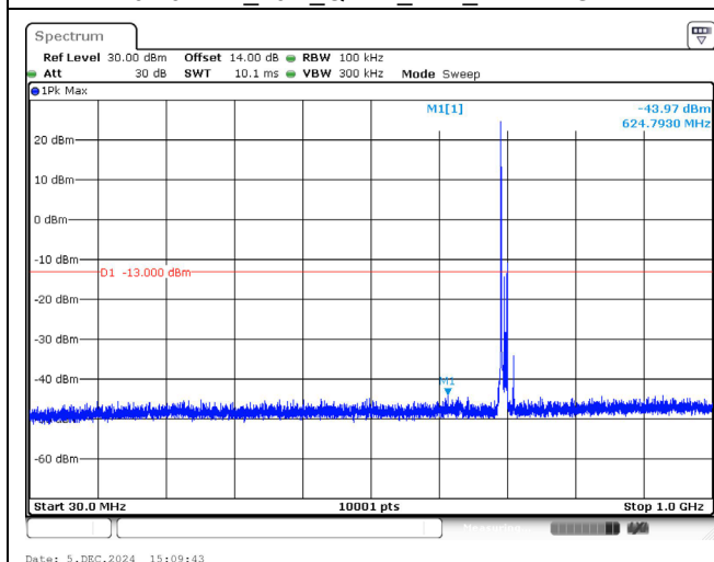
704.0 MHz_10M_QPSK_1RB_Below 1GHz
