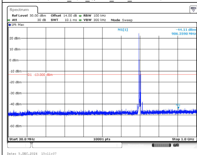
707.5 MHz_10M_QPSK_1RB_Below 1GHz
