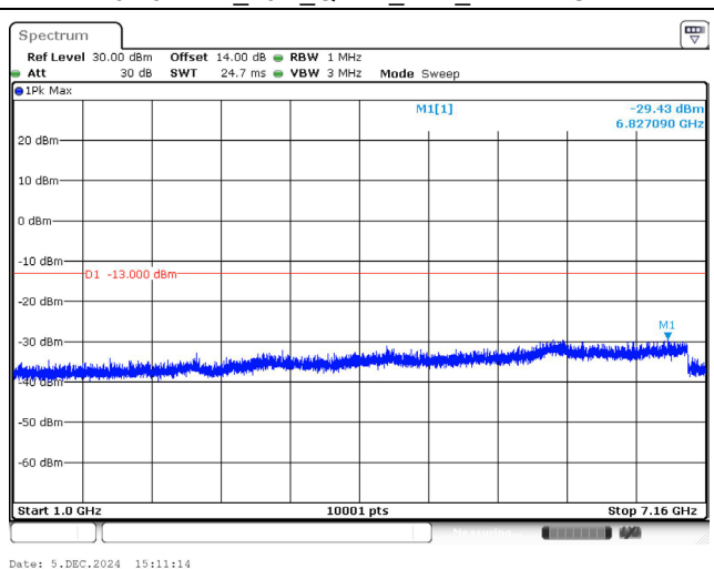
707.5 MHz_10M_QPSK_1RB_Above 1GHz
