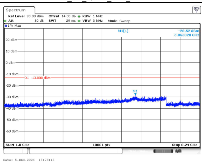
822.5 MHz_3M_QPSK_1RB_Above 1GHz
