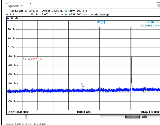
814.7 MHz_1.4M_QPSK_1RB_Below 1GHz
