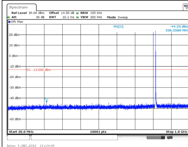
823.3 MHz_1.4M_QPSK_1RB_Below 1GHz
