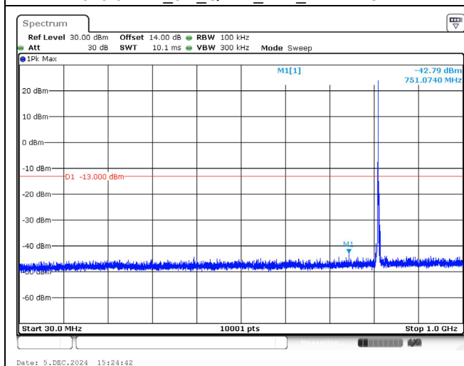
819.0 MHz_3M_QPSK_1RB_Below 1GHz
