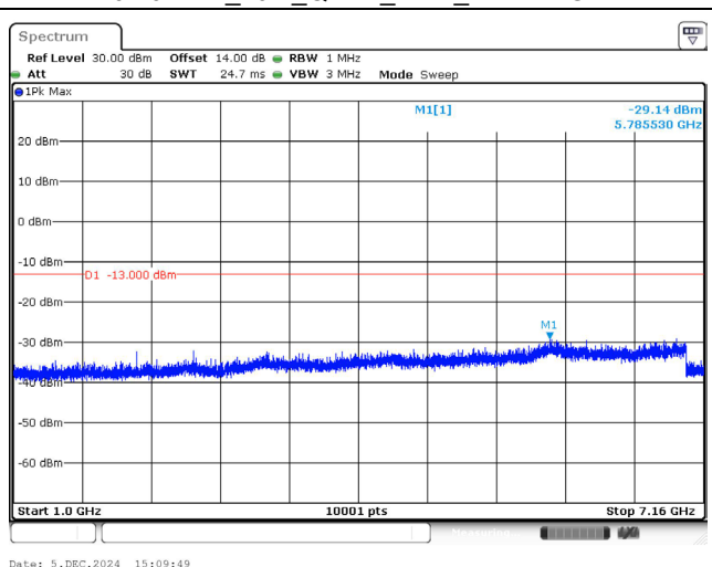
704.0 MHz_10M_QPSK_1RB_Above 1GHz
