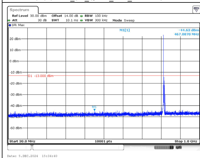
821.5 MHz_5M_QPSK_1RB_Below 1GHz
